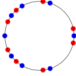
FIGURE 4. The Beukers-Heckman interlacing criterion [40] at work.
