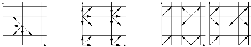
FIGURE 1. Some discarded models: trivial; intrinsic to the half-plane; symmetric.
