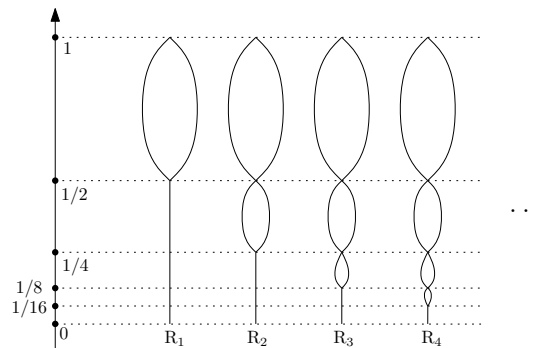
Figure 3.11: A sequence of Reeb graphs that is Cauchy but that does not converge in \mathbf{Reeb} because the number of critical values goes to +\infty . Indeed, each R_n has n + 2 critical values.
