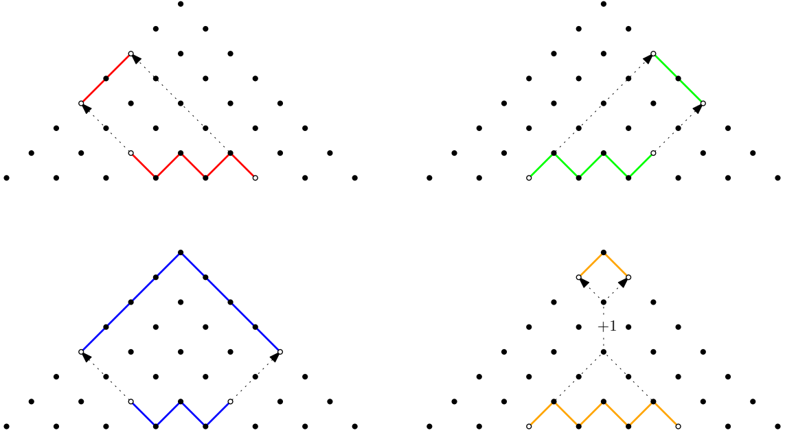
Figure 4.4: (From [28]) We show the axis of travel of birth and death endpoints of intervals of LZZ(f) to the up-down zigzag persistence module bounding the south face of the Mayer-Vietoris half-pyramid for interval modules that correspond to type I intervals (upper-left, red), type II intervals (upper-right, green), type III intervals (down-left, blue), and type IV intervals (down-right, orange) in LBC(f) . The +1 in the down-right figure means that the homological dimension is increased by one.
