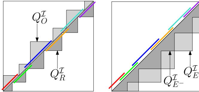
Figure 4.3: Left: Staircases of ordinary (light grey) and relative (dark grey) types. Right: Staircases of extended types— Q_{E^-}^\mathcal{I} is in dark grey while Q_E^\mathcal{I} is the union of Q_{E^-}^\mathcal{I} with the light grey area.
