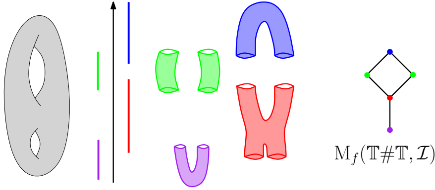
Figure 2.16: Example of the Mapper computed on the double torus \mathbb{T}\#\mathbb{T} with the height function f . The cover \mathcal{I} of \text{im}(f) \subseteq \mathbb{R} has four intervals (red, green, blue and purple), and the cover of the double torus has five connected components (one is blue, one is red, one is purple and the other two are green). The Mapper is displayed on the right.
