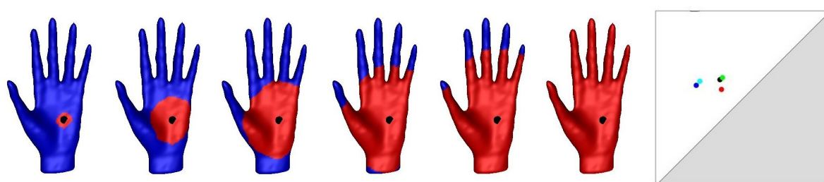
Figure 6.10: Same process as Figure 6.9 but with a different center point. Note the difference in the persistence diagram (far right). The colors in the diagram correspond to the same parts of the hand as in Figure 6.9. There is, however a new point in red, which corresponds to the hand base (palm), which was not present in the persistence diagram of the previous shape.
