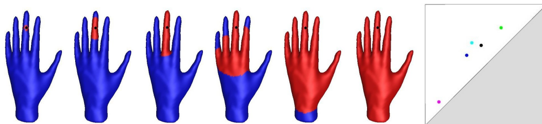
Figure 6.9: Geodesic balls centered at the black point are displayed in red. The persistence diagram corresponding to this family is shown in the far right. Note that each point can be easily associated with a shape part. The pink, blue, light blue, black and green points correspond to the middle, index, ring, pinky and thumb respectively. As the center point is close to the tip of the middle finger, one can see that its point in the persistence diagram is much closer to the diagonal than the other fingers. Note that for this shape, there are no essential holes.
