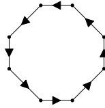
Figure 2.4: Example of an oriented 1-cycle.
