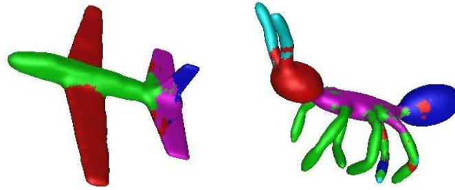
Figure 6.12: We compute the most common label for each face in a set of 100 nearest neighbors computed from a training set. No smoothing is applied but the segmentations on this pair of shapes are still reasonable (around 80 percent accuracy). However, this accuracy can decrease to 60 percent in other categories, thus we need a more elaborate algorithm for segmentation.
