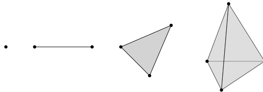
Figure 2.1: Example of geometric simplices in dimension 0, 1, 2 and 3.
