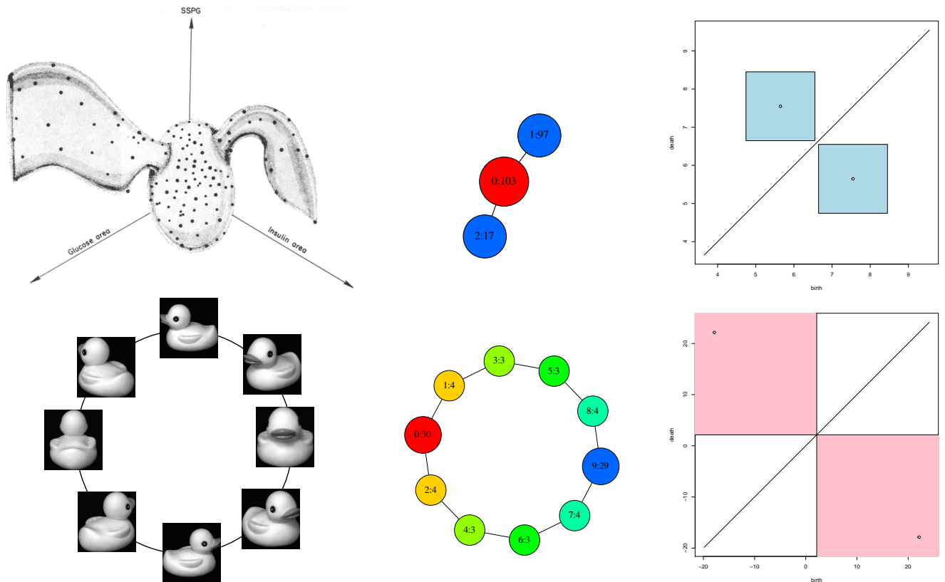
Figure 5.4: Mappers computed with automatic tuning (middle) and 85 percent confidence regions for their topological features (right) are provided for the Reaven-Miller dataset (first row) and the COIL dataset (second row).
