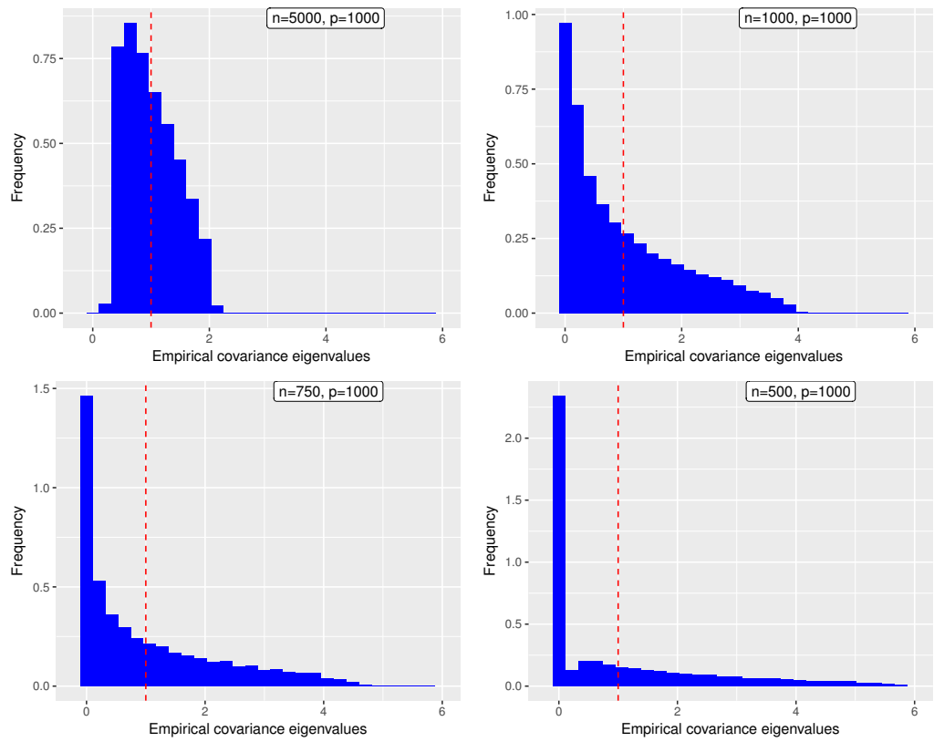
Figure 1.4 – Spectra of the empirical covariances of i.i.d. data coming from a \mathcal{N}(0, \mathbf{I}_{1000}) distribution. The number of observations has to be much higher than p for the spectrum to concentrate towards the theoretical value of 1. For smaller values of n , many eigenvalues are null or very small, and the rest of the spectrum is very spread out.
