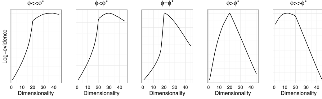
Figure 5.1 – Different shapes of the marginal likelihood curve for growing values of \phi . \phi^* corresponds to the maximum of the heuristic criterion that we describe in Subsection 5.3.3. The true dimensionality is 20.
