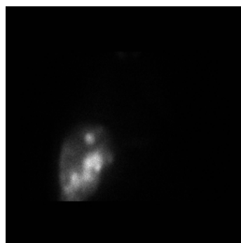
(a) ^{99m}\text{Tc} -MAA SPECT
