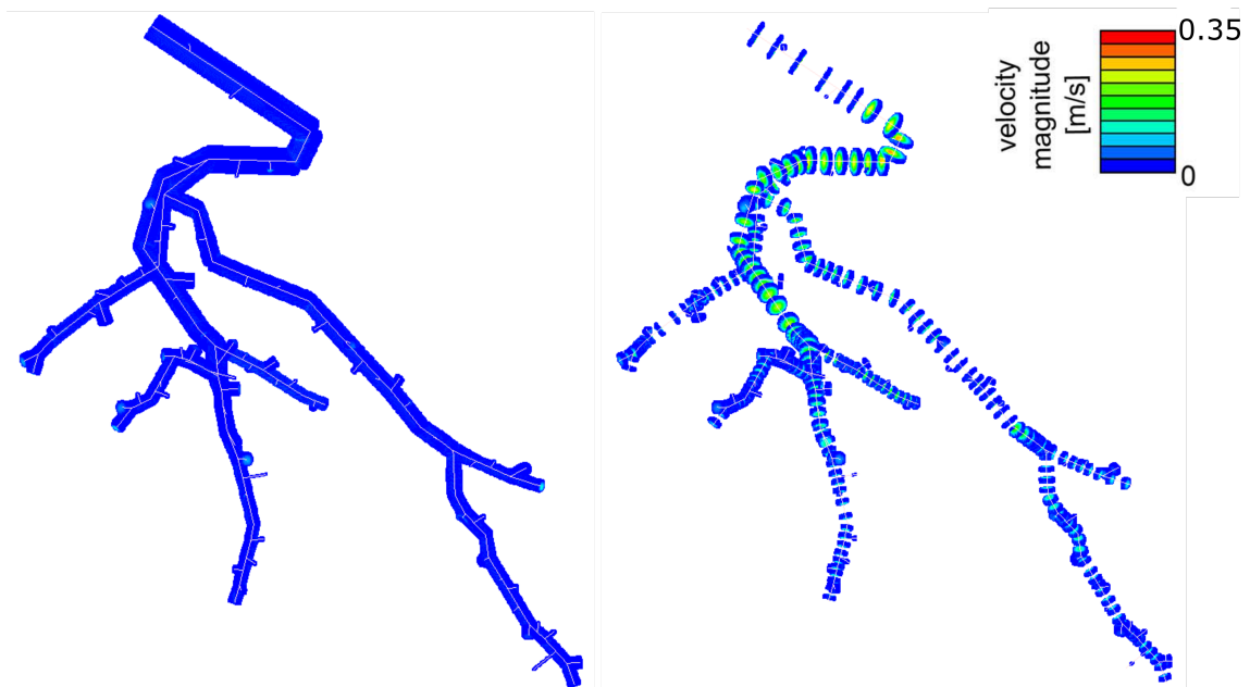
Figure 5.4: LBM blood simulation in the patient-specific arterial tree of Patient 2. Vessels with diameter > 2 mm represent the simulation domain. On the left, the vessels borders, where velocity is zero due to no-slip conditions, are visible. On the right image, regular slices of the vessels illustrate velocity at the interior of the vessels
