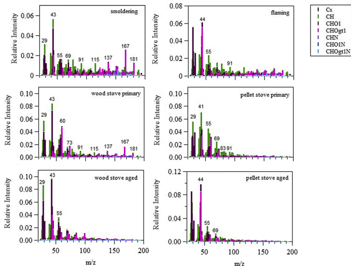
Fig. 6. High Resolution mass spectra of primary and aged biomass burning organic aerosol for a logwood stove (Exp. 1) and pellet stove (Exp. 10) experiment as well as organic aerosol sampled during the smoldering and flaming stage of the combustion with a logwood stove (Exp. 2).
