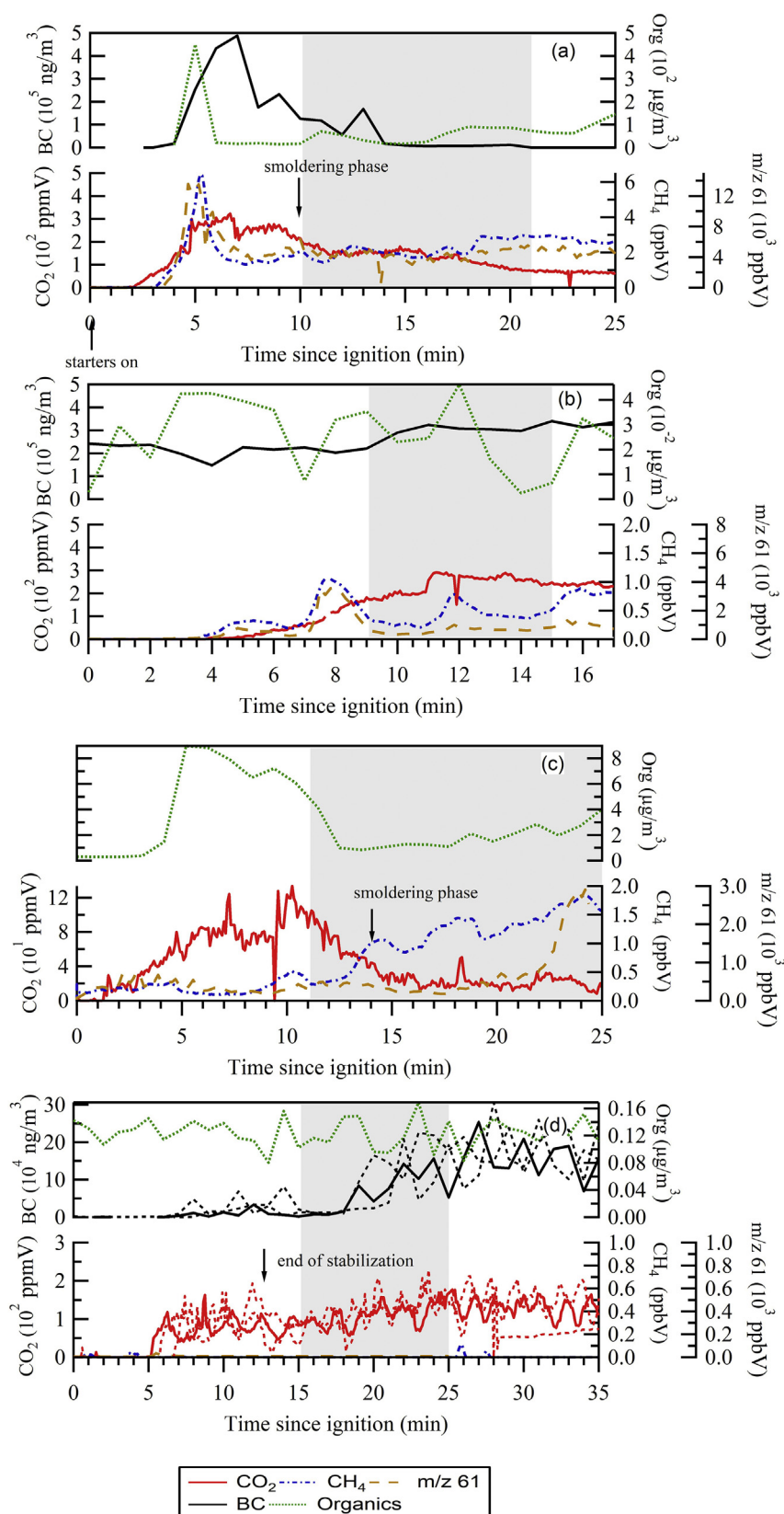
Fig. 3. Trace dynamics of the emissions of particulate (top) and gaseous (bottom) species during combustion. BC (black), organic aerosol (green), \text{CO}_2 (red), \text{CH}_4 (blue), and m/z 61.028 [\text{CH}_3\text{COOH}]\text{H}^+ (orange), corresponding to the protonated molecule of gas phase acetic acid (PTR-ToF-MS measurement). The grey bar indicates the phase injected in the smog chamber. (a) Wood Stove A (<2002) – Exp 1. (b) Wood Stove A (<2002) – Exp 4. (c) Wood Stove B (2010) Exp 6. Exp 10. (d) Pellet Stove C (2010) – Exp 9 (and exp. 10 and 11 in dotted line). (For interpretation of the references to colour in this figure legend, the reader is referred to the web version of this article.)
