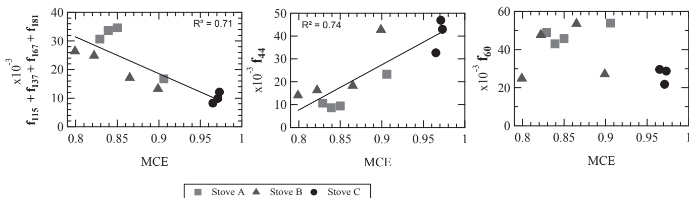
Fig. 7. Summed contributions to the total organics of specific biomass burning fragments: m/z 115 ( \text{C}_9\text{H}_7^+ ), m/z 137 ( \text{C}_8\text{H}_9\text{O}_2^+ ), m/z 167 ( \text{C}_9\text{H}_{11}\text{O}_3^+ ) and m/z 181 ( \text{C}_9\text{H}_9\text{O}_4^+ ), and the contribution of m/z 60 ( \text{C}_2\text{H}_4\text{O}_2^+ ) to the total organics, as a function of the MCE.
