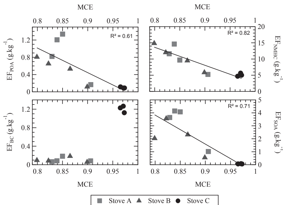
Fig. 5. Particulate phase emissions and gaseous phase emissions as a function of the Modified Combustion Efficiency (MCE).
