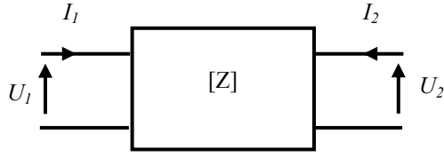
Figure 1. Two-port network
