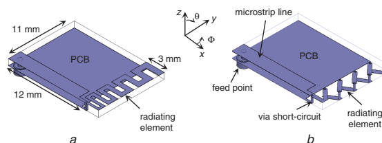
Fig. 2 Proposed antennas
