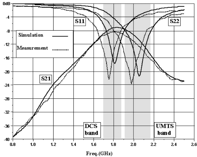
Fig. 5. Simulated and measured S_{11} , S_{22} , S_{21} of the DCS/UMTS PIFAs arrangement when feeding strips are facing ( d = 18 mm).
