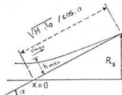
FIGURE 35 REPRESENTATION GRAPHIQUE DES NOTATIONS
