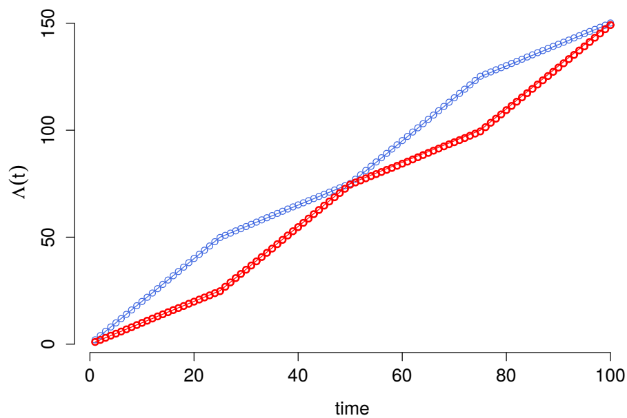
Figure 2.4 – Real 2.4a and estimated 2.4b integrated intensity functions (IIFs) according to the generative model in the first scenario ( \psi = 4 ). In blue, the intensity function \Lambda_1(\cdot) represents the mean number of interactions within clusters. In red, \Lambda_2(\cdot) represents the mean number of interactions between clusters.
