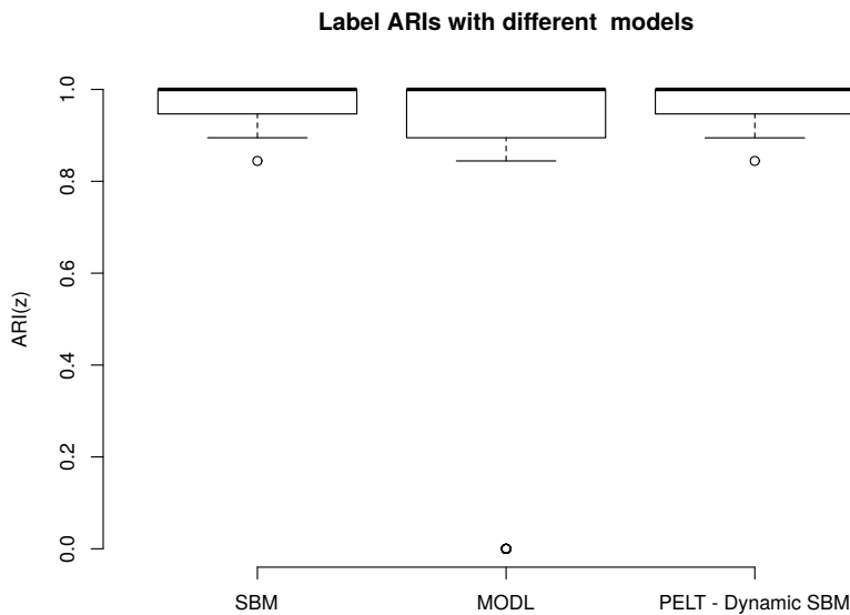
Figure 3.5 – Boxplots over 50 simulations of the ARIs for the clustering structures obtained by SBM, MODL and PELT-Dynamic SBM for scenario 2. More details in the text.
