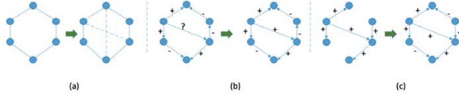
Figure 4.1: Different link analysis tasks [J. Tang, S. Chang, et al., 2015].
