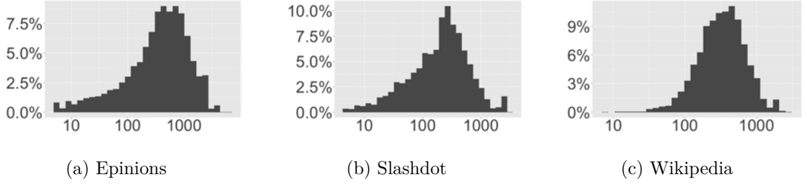
Figure 4.6: Distribution of size of primary neighborhood sets in three datasets (log scale)
