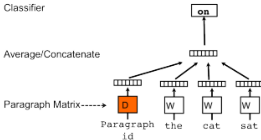
Figure 3.14: Doc2Vec [Le and Mikolov, 2014]. Doc2Vec is very similar with Word2Vec , except that it takes the document’s content into account.
