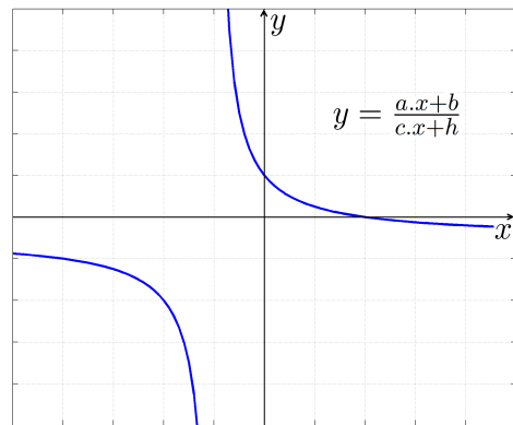
(f) Hyperbolic
