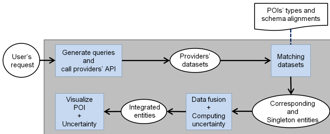
FIGURE 6.15: Process flow of UNIMAP prototype.
