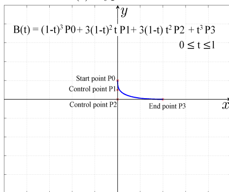
(h) Cubic Bezier with exponential decay
