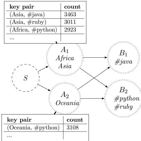
Figure 2.9: PO instrumentation: every instance counts the key pairs it receives and sends, and keeps the most frequent pairs in memory.
