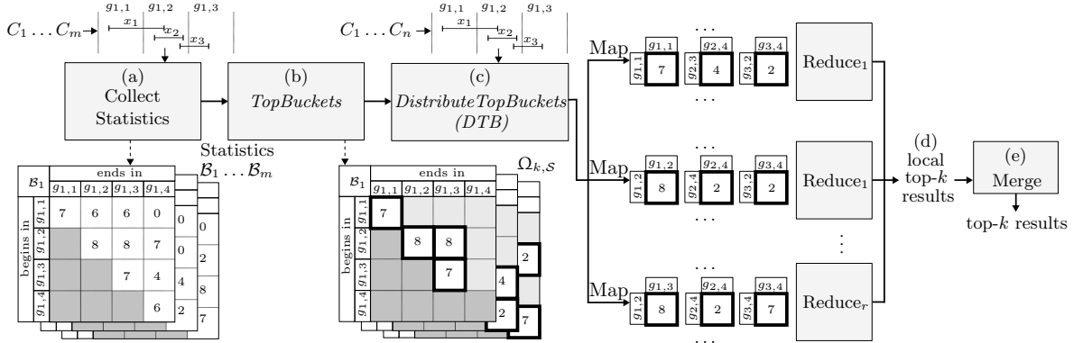
Figure 3.5: Overview of TKIJ
