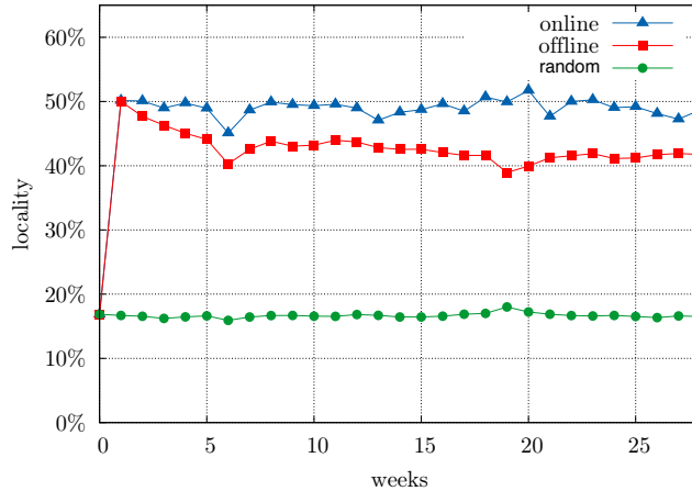
Figure 2.11: Locality obtained with different data placement policies
