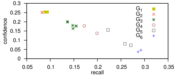
Figure 4.3: Avg. recall/confidence of the top-20 results of interestingness measures
