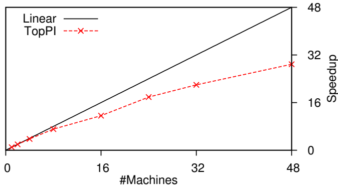
Figure 3.11: TopPI speedup when running on Hadoop with on Supermarket ( k = 1000 )
