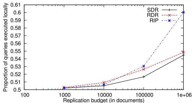
Figure 2.3: Query locality wrt. replication budget
