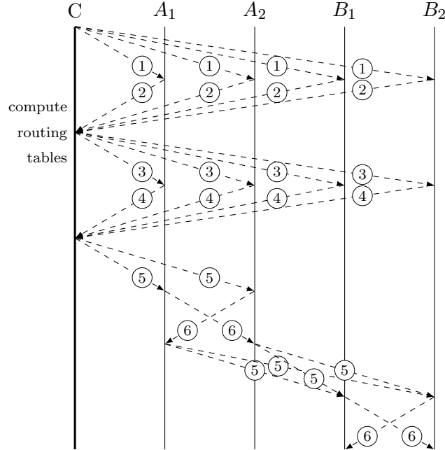
Figure 2.10: Reconfiguration protocol, forwarding routing tables and key states between POIs. ① Get statistics. ② Send statistics. ③ Send reconfiguration. ④ Send ACK. ⑤ Propagate. ⑥ Exchange keys.
