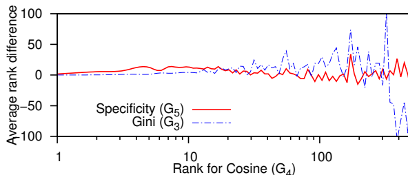
Figure 4.2: Rank correlations
