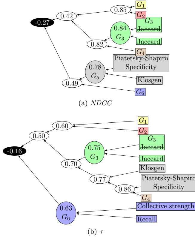
Figure 4.1: Hierarchical clustering of interestingness measures for a single target
