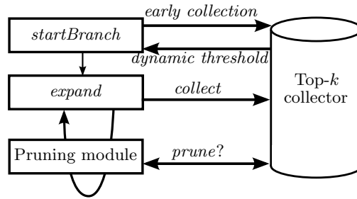
Figure 3.9: Overview of TopPI
