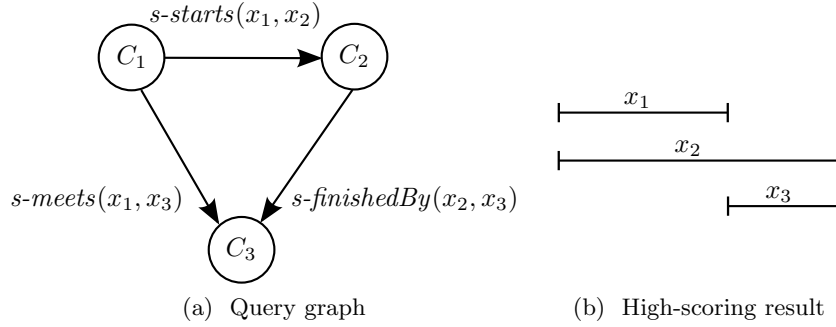
Figure 3.4: Example of RTJ query
