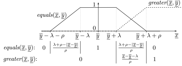
Figure 3.3: Approximating equals and greater . Here, \bar{x} \in \{x, \bar{x}\} , \bar{y} \in \{y, \bar{y}\} .
