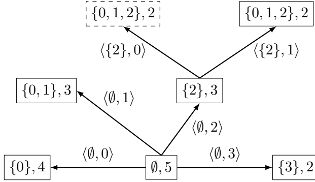
Figure 3.8: CIS enumeration tree on our example dataset (Table 3.3a). \langle P, i \rangle denotes extension to closed ItemSest operations.
