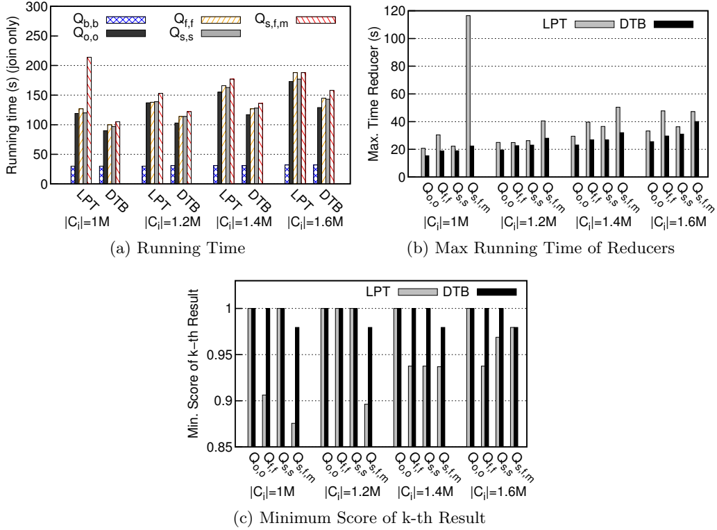
Figure 3.6: Synthetic Data - Workload Distribution
