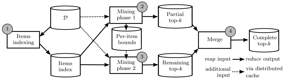
Figure 3.10: Hadoop implementation of TopPI
