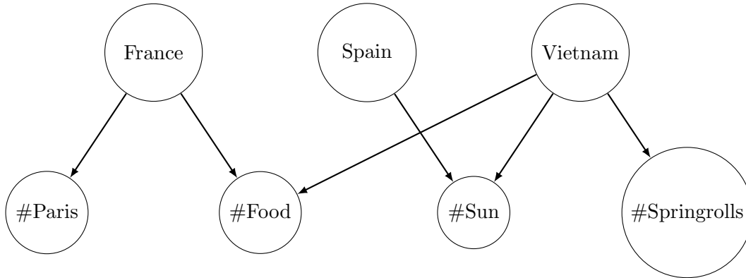
Figure 2.6: Graph obtained with routing sequences. The first key corresponds to a location, while the second key is a hashtag. Tweets posted in France are associated with hashtags #Paris and #Food.
