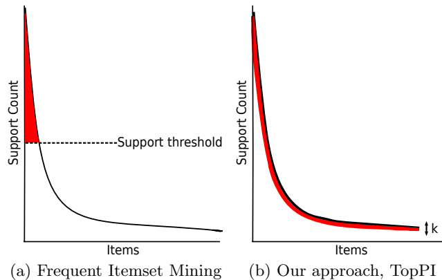
Figure 3.7: Schematic distinction between frequent itemsets mining and TopPI. The area in red represent each method’s output.
