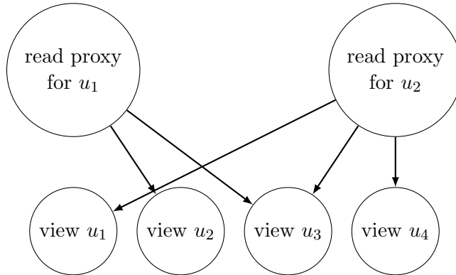
Figure 2.5: Graph obtained with multi-get queries in a social network. u_1 follows u_2 and u_3 while u_2 follows u_1 , u_3 and u_4 .
