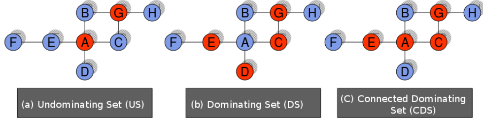
FIGURE 4.1: Dominating Set
