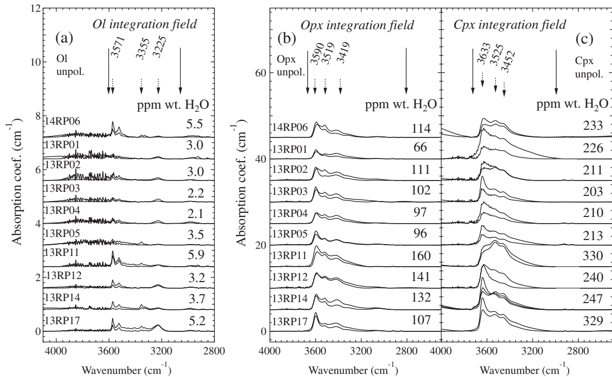
Fig. 6. Representative unpolarized FTIR spectra for Ray Pic spinel-peridotite xenoliths: (a) olivine (ol), (b) orthopyroxene (opx), and (c) clinopyroxene (cpx). Spectra with minimal and maximal absorbance are given for each sample. All spectra are normalised to 1 cm of thickness. Long black arrows indicate the integration range used for the IR calibration; the short dashed arrows indicate the major OH absorption bands of the mineral.
