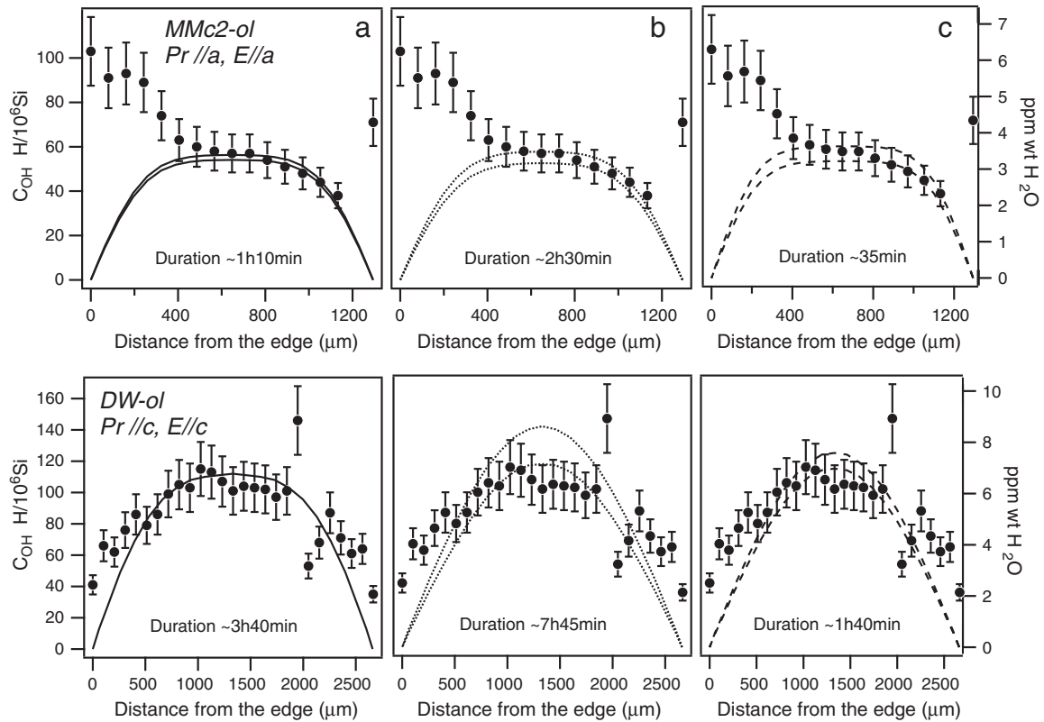
Fig. 12. Representative profiles of H concentration in MMC olivine and DW olivine and calculated with the 3D model. a) Solid curves show the two best results. b) Dotted curves: -50^{\circ}\text{C} . c). Dashed curves: +50^{\circ}\text{C} temperature.
