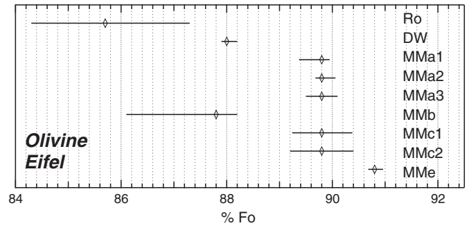
Fig. 4. Forsterite content expressed as %Fo (i.e., %Fo = Mg / (Mg + Fe) × 100) for xenoliths from Rockeskyllerkopf (Ro), Dreiser Weiher (DW), and Meerfelder Maar (MM).
