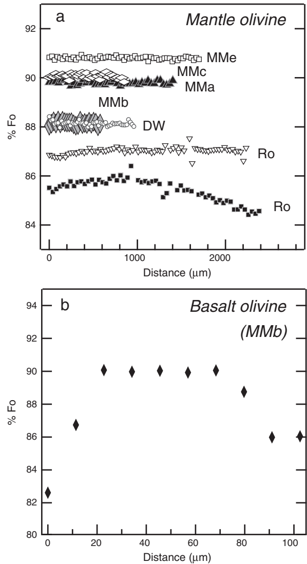
Fig. 5. Forsterite contents across olivine grains. a) Longest %Fo profile vs distance obtained for mantle-derived olivine from each thin section. b) %Fo profile vs distance obtained in an olivine phenocryst in the basalt crust of MMB sample.
