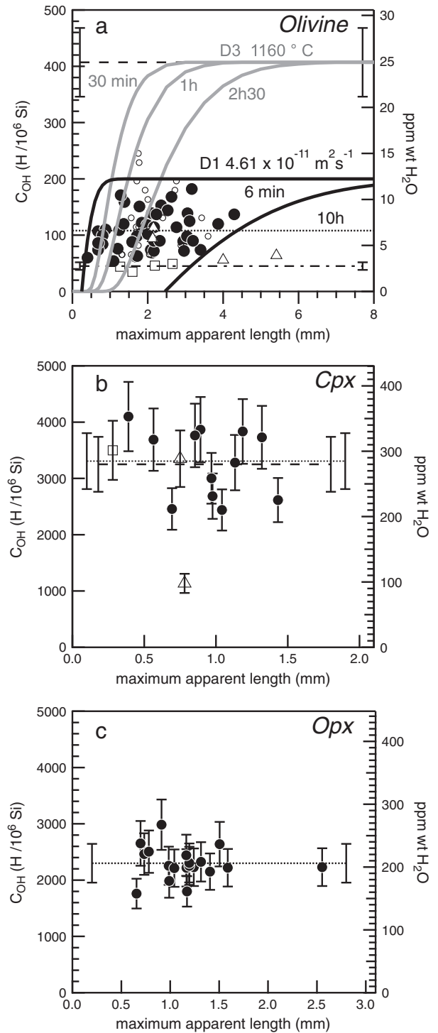
Fig. 8. C OH as a function of the maximum apparent length (mm) of the grain. Each datum point corresponds to one FTIR spectrum. C OH have 30% of uncertainties, and the error bar on the hydrogen concentration in olivine is not shown for clarity. Circles: MM squares: Ro; triangle: DW. The dotted line is the average hydrogen concentration. The dashed line is the expected initial H concentration in MM grains derived from partition coefficient of H 2 O olivine/opx = 0.11 (Aubaud et al., 2004). a) In the case of olivine, the dot-dashed line is based on the almost flat distribution of the data from Ro. The gray curves represent the variation of hydrogen concentration at grain centers as a function of the grain size from the 3D diffusion model with an initial concentration of 25 ppm H 2 O wt. (360 H/10 6 Si), and for various durations. The black curves are from the 1D diffusion model for an initial concentration of 12 ppm H 2 O wt. (200 H/10 6 Si), for various durations. See Section 4.4.1 for details.
