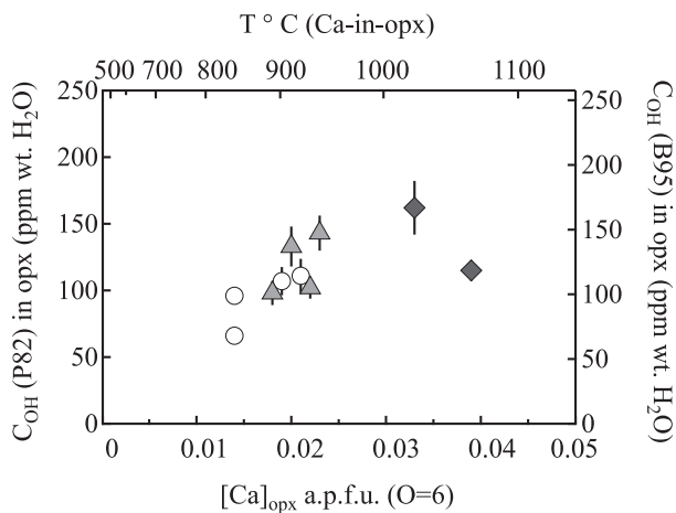
Fig. 14. Water contents in opx (in ppm wt. H 2 O, based on calibration of Paterson, 1982 (P82); and Bell et al., 1995 (B95)) as a function of [Ca] a.p.f.u. (atom per formula unit calculated for 6 bonding oxygens) for Ray Pic spinel-peridotite xenoliths. Corresponding temperature (in °C) was calculated using Brey and Köhler (1990) 'T Ca-in-opx ' geothermometer. Error bar on the average values of water content per sample is 1SD.
