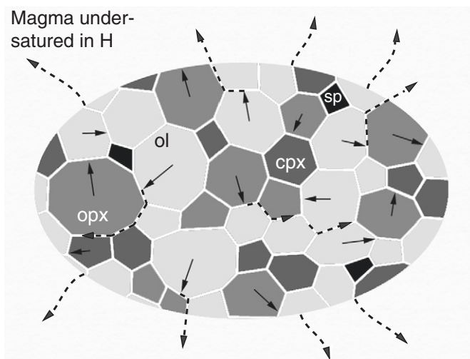
Fig. 11. Schematic diagram illustrating the mobility of H in a mantle xenolith transported by magma; dashed arrow: diffusion of H along the inter-granular space/interface to the magma, solid black arrow: diffusion of H from a crystalline solid to the intergranular space/interface.
