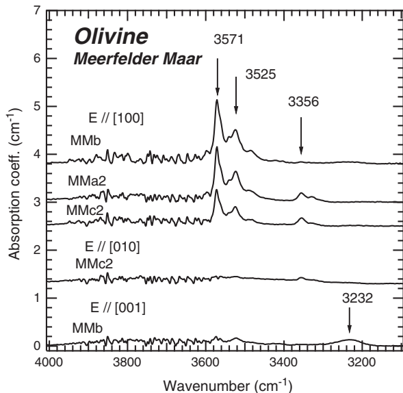
Fig. 7. Polarized infrared spectra of olivine representative of each crystallographic axis. Spectra are normalized to a thickness of 1 cm.
