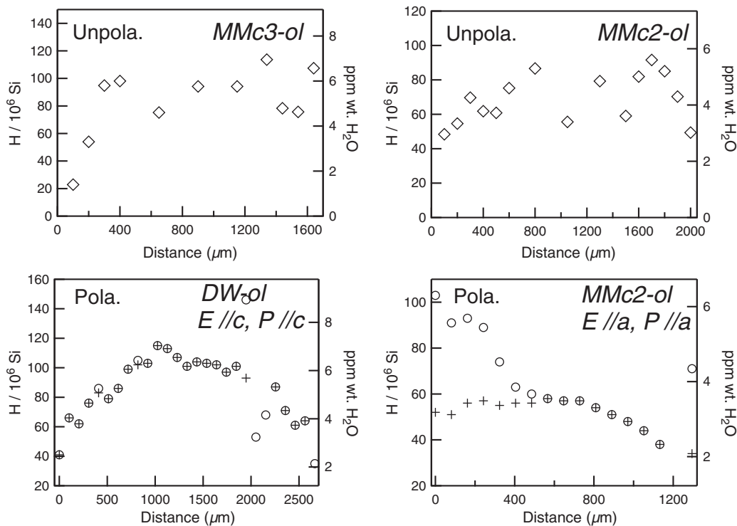
Fig. 10. Hydrogen concentration ( \text{H}/10^6 \text{ Si} and ppm wt. H 2 O) as a function of the distance along the grain of olivine (in \mu\text{m} ): the circles represent the concentration of the absorption spectrum from raw data; crosses correspond to the concentration calculated from the absorption spectrum corrected (without contamination or edge effects). Unpola.: unpolarized IR radiation; Pola.: Polarized IR radiation. The error on the hydrogen concentration is about 30%, the error bars are not shown for clarity.
