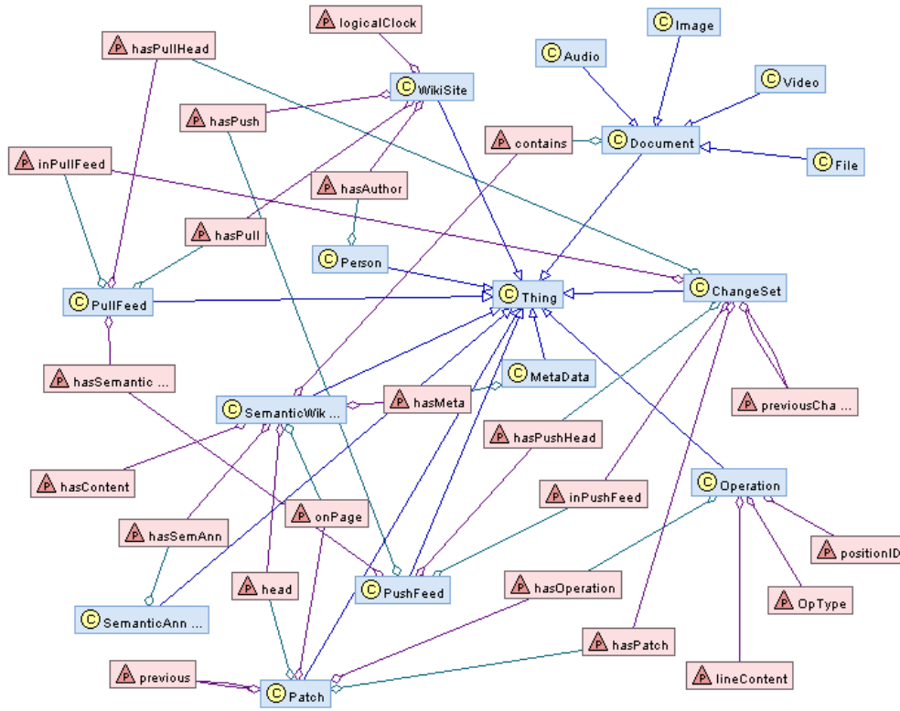
Figure 2.5 – Mutli-synchronous ontology
