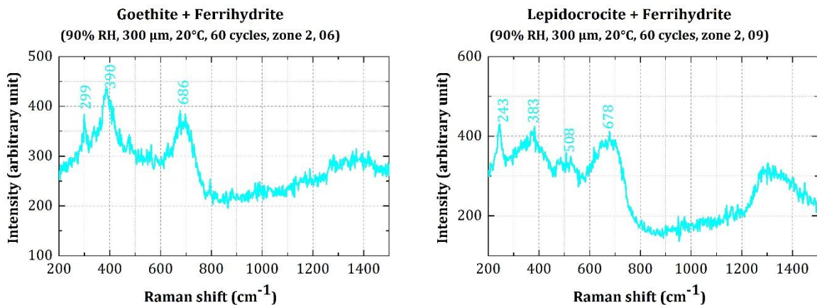
Figure 5-21: Raman spectra of corrosion products obtained on specimens having 300 μm residual crack width and subjected continuously to 90% RH
