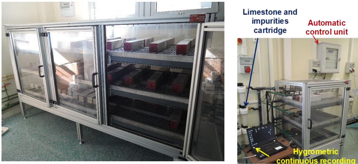
Figure 2-23: Real atomized device for humidification/drying cycles
