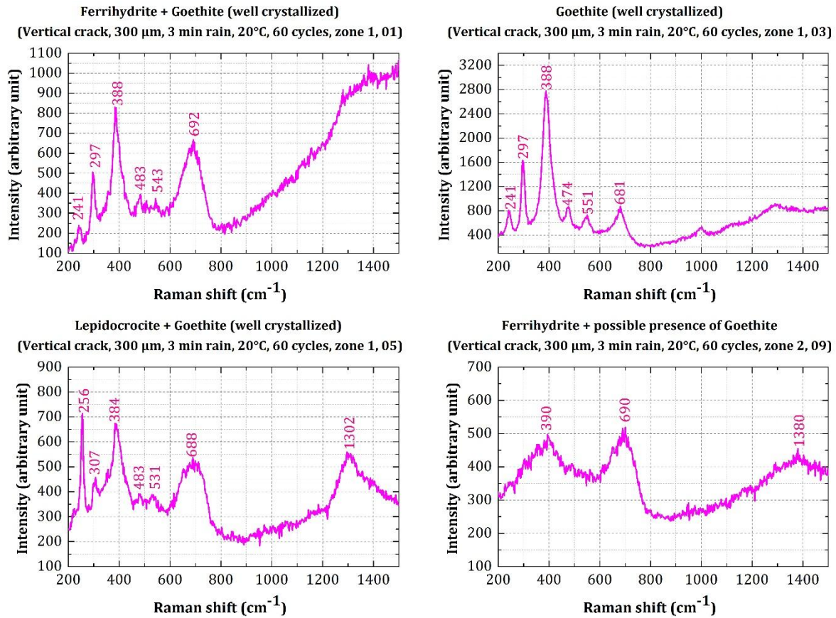
Figure 5-20: Raman spectra of corrosion products obtained on specimens having 300 μm residual crack width and subjected to 3 minutes rain at each raining/drying cycle.
