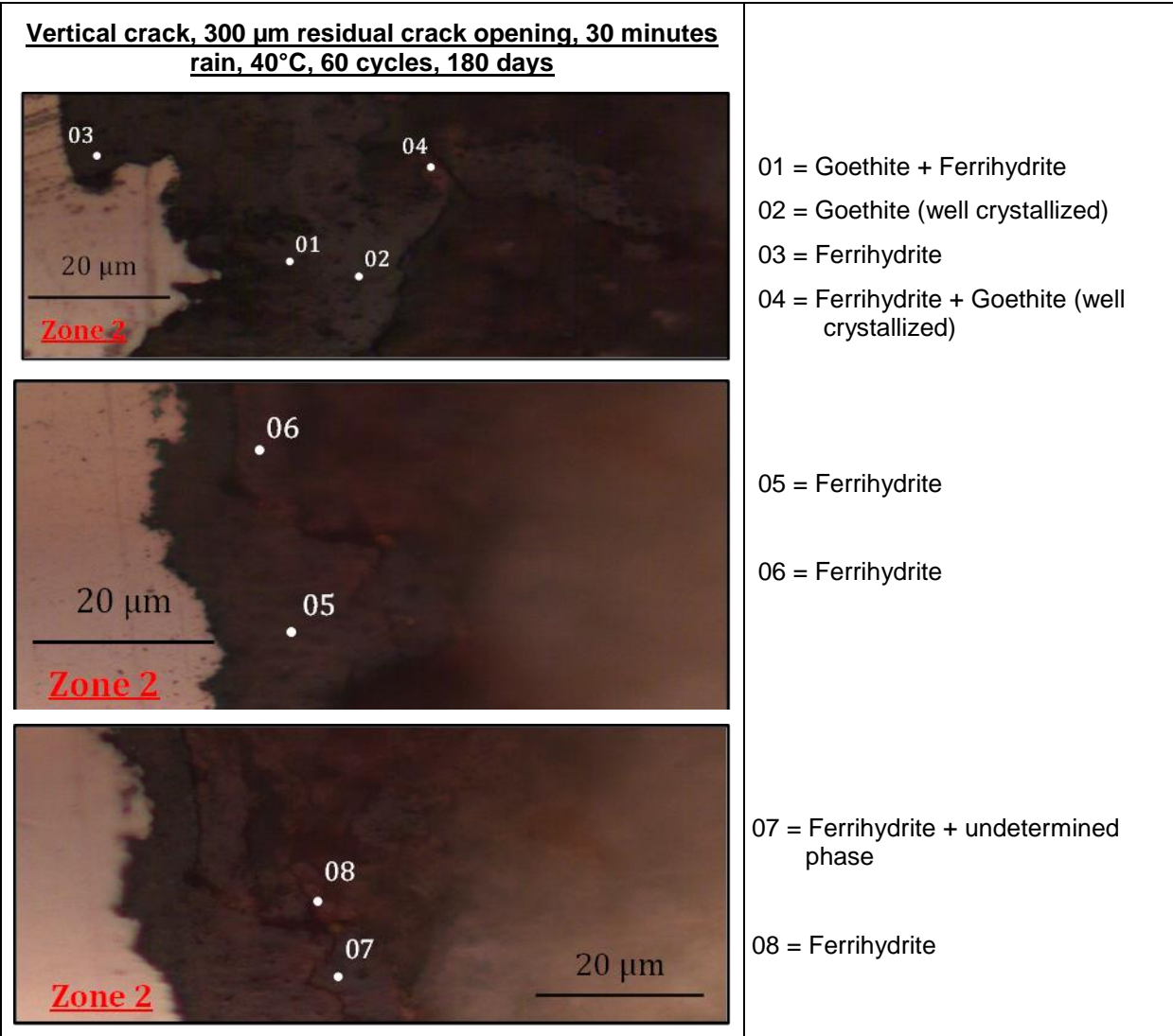
Figure 5-31: Corrosion layer observed at steel/mortar interface located deep in the crack in a specimen having 300 μm residual crack width and corroded under raining/drying cycles at 40°C
