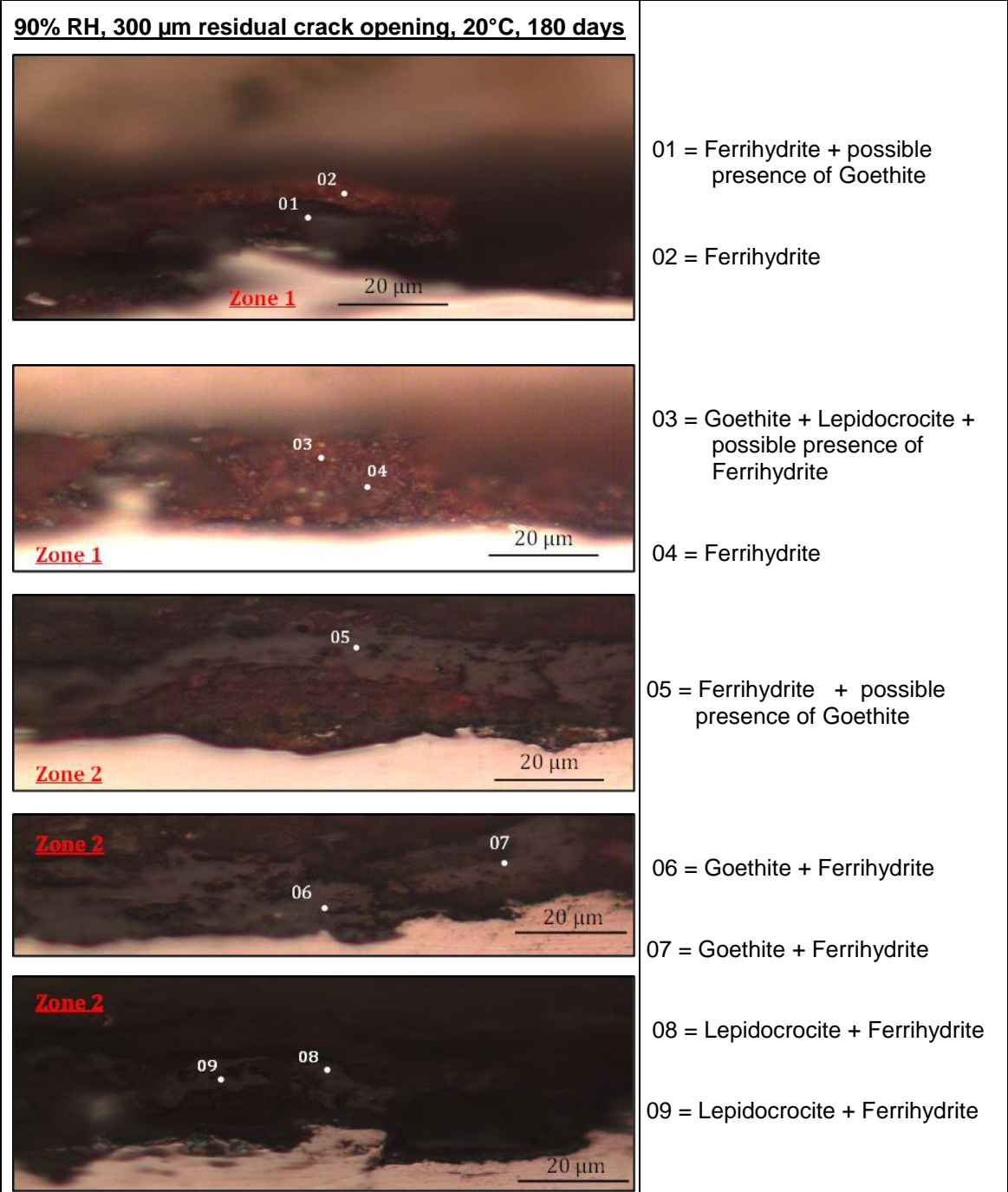
Figure 5-19: Corrosion layer observed at steel/mortar interfaces located far from the crack and deep in the crack in specimens having 300 μm residual crack width and exposed continuously to 90% RH.
