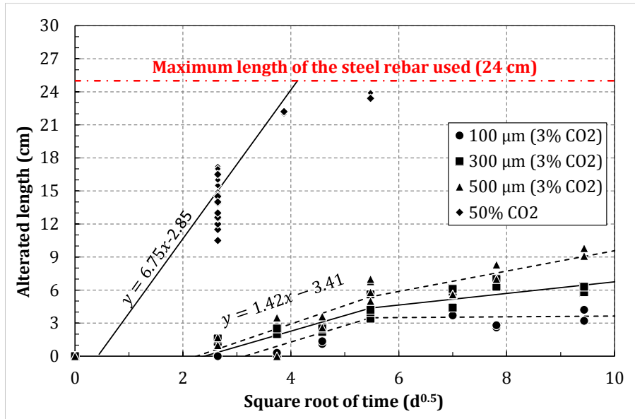
Figure 3-12: Carbonation length along the steel/mortar interface with respect to square root of time for two carbon dioxide concentrations (3% \text{CO}_2 ; 50% \text{CO}_2 )
