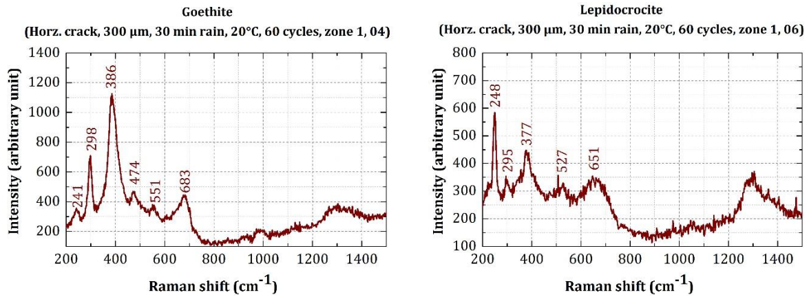
Figure 5-9: Raman spectra of corrosion products obtained on specimens having 300 μm residual crack width oriented horizontally with respect to rain
