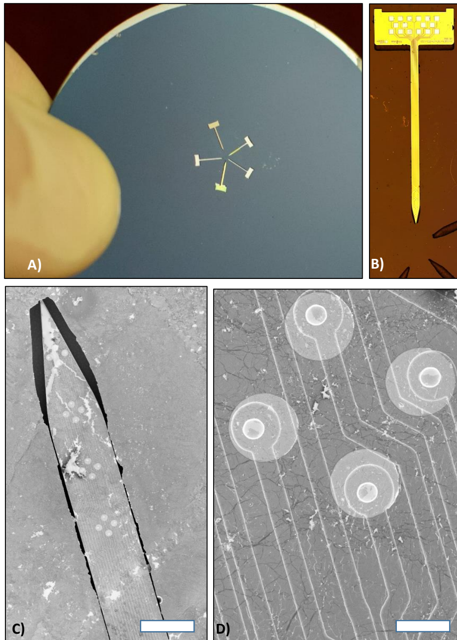
Figure 102 – Buried probe in a wafer is properly covered with graphene except few sites with graphene cracks: A wafer is used a mold to burry probes and have them on the same surface than silicon oxide to reduce strains on graphene during transfer B The probes are placed inside the molds (Micrography) C SEM picture of commercial intracranial probe drowned into its silicon mold and uniformly covered with graphene in grey. Scale bar is 100 \mu\text{m} D Close up view of graphene coated electrodes on the implant shows few graphene cracks and graphene wrinkles on the surface. Scale bar is 10 \mu\text{m}
