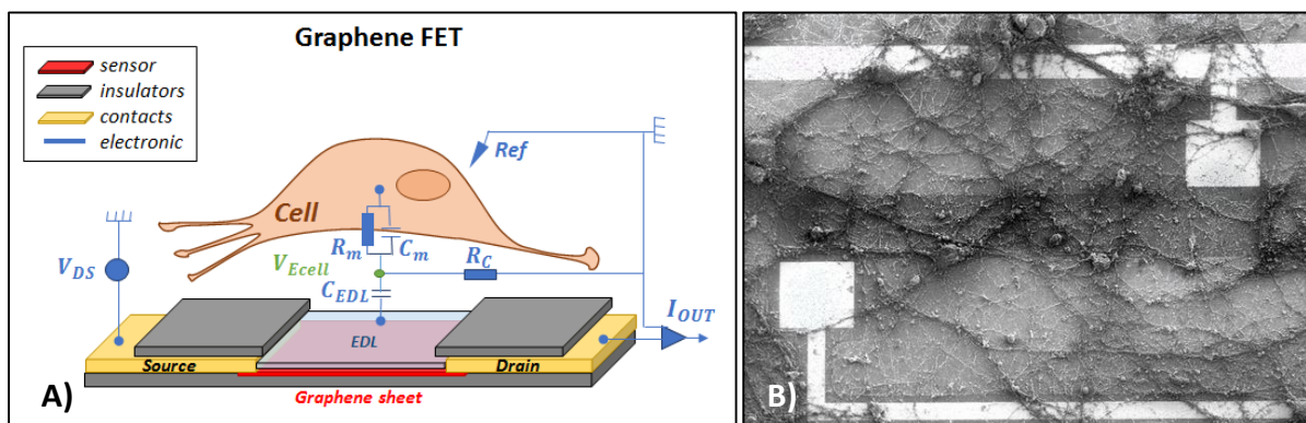
Figure 67 - Neurons in situ grown onto graphene Field Effect Transistors. A) Principle of extracellular detection of neurons spikes and the GFET electronics showing liquid gating measurement process. V_{DS} Corresponds to drain source polarization tension and C_{EDL} to the Electrical Double Layer Capacitance responsible for the gating insulation. B) SEM picture of neurons grown on a FET showing multiples neuritis and soma covering the G-FET. They will act as a front gate for the transistor and the two electrodes will allow detection of activity by Drain Source current measurement. From F. Veliev [99] Scale bar is 50 \mu m.
