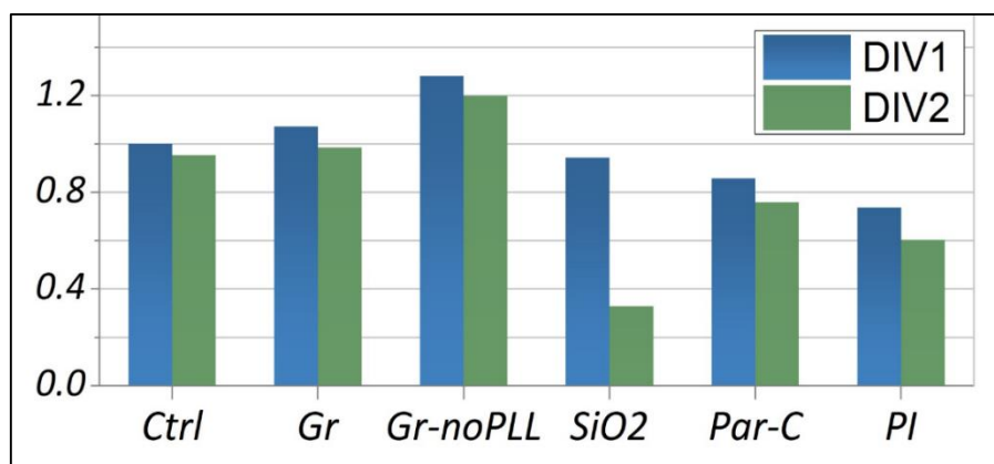
Figure 54 – Cell cultures on our panel of material revealed high graphene cytocompatibility: Statistical in-vitro neurons counting after hippocampal cells spreading on different substrate material has shown graphene to be a better supportive material for neurons development than SiO2. Institut Néel – F.Veliev [99].
