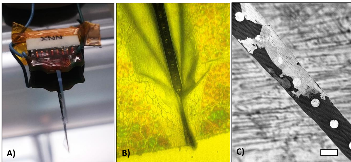
Figure 99 – Standard graphene transfer on 3D thin device does not provide good graphene coverage because of carrier strains A) Neuronexus implant with its connector placed on top of a silicon wafer for direct transfer. B) Optical microscopy shows important strain on PMMA layer once covering the probe, suggesting graphene strain linked to connector leverage. C) SEM picture after acetone PMMA removal shows very few and in bad shape graphene on some parts of the implant. Scale bar: 40 μm
