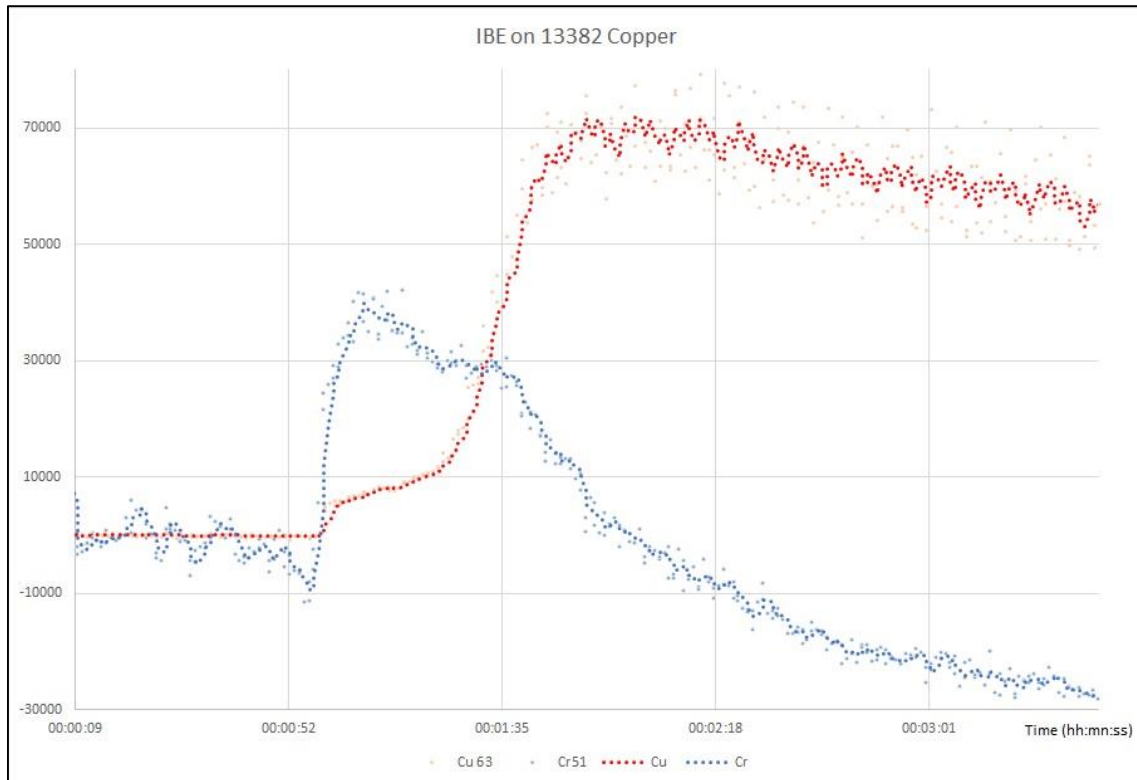
Figure 38 - EDX shows a chromium alloy on standard copper surface. Chromium and Copper tracking when physically etching a copper foil with Ion Beam Etching. In red, copper is more and more present when chromium in blue decrease along the etching of the Alfa Aesar #13382 copper foil surface
