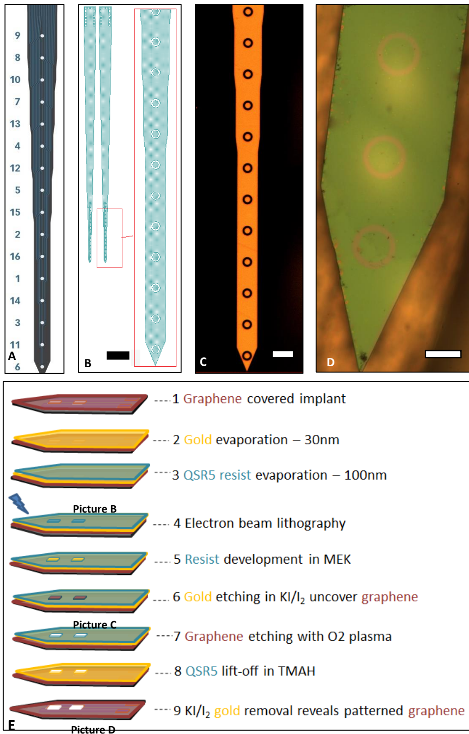
Figure 106 - 3D lithography custom process for graphene patterning on an implant using electron beam lithography: A) A Neuronexus 16MEA probe was taken as the reference design to develop this process B) I created a lithography mask by reverse engineering to prepare graphene e-beam lithography on the implant C) An optical microscopy picture of the so lithographed probe at step 6 shows etched gold to uncover graphene on desired zone to isolate underlying electrodes. A, B and C scale bars are 50 \mu m D) This photography shows very well the graphene etched on desired zone at step 9. This picture have been made on a dummy probe I built to find the perfect recipe and the good electron beam energy dose to polymerize QSR5 on gold. Scale bar: 40 \mu m E) Process flow of the QSR5 e-beam lithography process and graphene patterning through gold hard mask. Process is explained in text.
