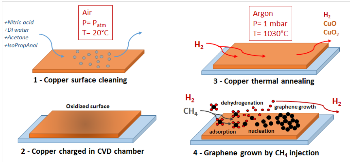
Figure 33 - Main steps of graphene growth on copper from hydrocarbon precursor: 1 – Copper surface is cleaned according to our recipe detailed in next paragraph “substrate preparation”. 2- Copper foil is charged in the CVD quartz tube on a quartz holder (see photo on Figure 9). 3 – After vacuum pumping and heating up to 1030^\circ , copper is thermal annealed during 30 to 60 min to remove surface and bulk oxide and eventually clean bulk contaminants that should leave the surface during this step. 4- Graphene growth is launched by \text{CH}_4 injection in a \text{H}_2 and Argon atmosphere that will trigger physisorption of \text{CH}_4 and chemisorption of \text{H}_2 on the surface then dehydrogenation of \text{CH}_4 and nucleation of carbon atoms on the surface to form honeycomb lattice of graphene. Bulk in and out diffusion of carbon atoms happens also but is not represented here, they will be detailed after.
