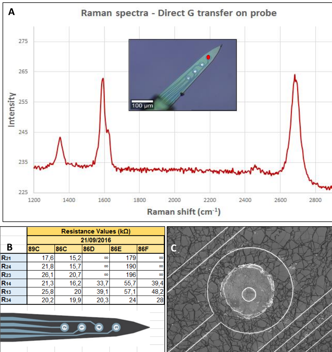
Figure 105 - Graphene coating is continuous as verified by conduction measurement and Raman spectroscopy: A) Raman spectra shows specific graphene peaks as explain in chapter II, G peaks is almost as high as 2D peak, suggesting multilayer graphene, probably linked to wrinkles seen on SEM picture. D peak however reveals few defects in graphene structure, most likely due to the strains induced on graphene by transfer without carrier B) A majority of sensors are connected to each other. The resistance between 2 well connected sites was evaluated to around 4kΩ by extrapolating the different values in function of distance between sensors. The main resistance value of around 20 kΩ might be coming either from graphene coupling to metallic sensors, or to the length of contact electrodes to the connector. C) Close up view of a covered sensor shows wrinkles that resemble multilayers area which could explain previous Raman state.
