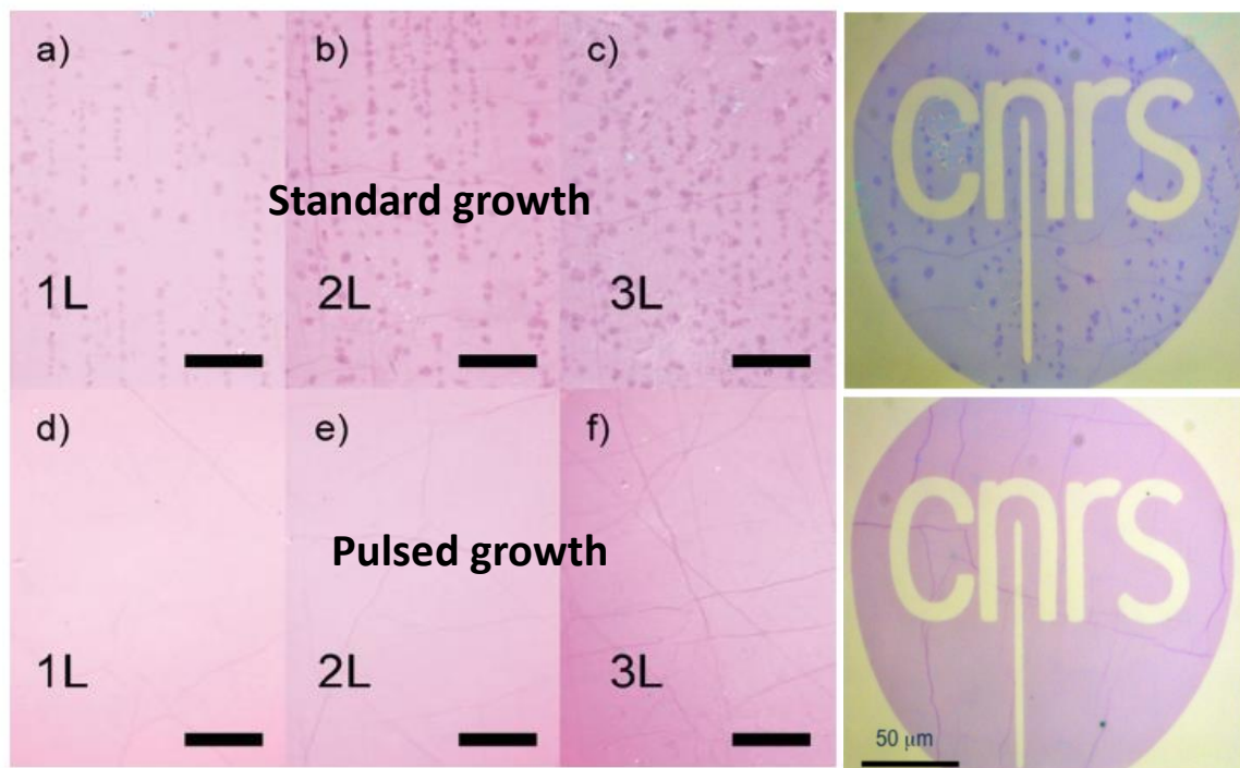
Figure 28 – Comparison between stacks made of piles of continuous CVD and pulsed CVD graphene: Optical microscope photography shows monolayer (a&d) transferred graphene on oxidized silicon. And multilayers obtained by successive transfers (b, c e and f). Top pictures (a,b&c) show standard CVD growth whereas bottom ones show pulsed growth graphene. Pulse growth allows removal of multilayer patches and is detailed in next paragraph. Right pictures show corresponding graphene patterned with CNRS logo. Z. Han, Institut Néel-[126].
