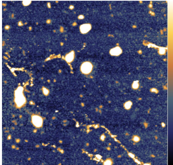
Figure 63 – Atomic force micrograph (non-contact mode) performed on HA coated graphene (10 x 10 μm size) showing agglomerates of HA (brightness areas). Color z-scale is 10 nm.
