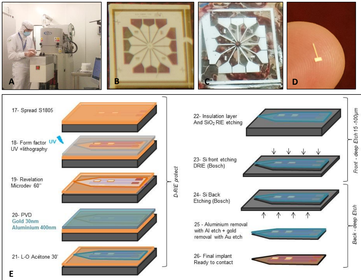
Figure 93 - From flat substrate devices to a 3D micro machined probe using Deep Reactive Ion Etching: A Shows DRIE machine, B a flat device (previously introduced) and C the same device after DRIE etching. D shows the size of an implant I built to be used as a dummy probe to test 3D graphene transfer. E Process flow: I start with a photolithography to pattern a protective metal hard mask, then use PVD deposition of metal to create a layer of gold and aluminum and finally, after resist liftoff, I perform etching of the different layers until probe of the desired thickness is released.
