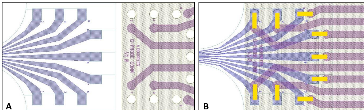
Figure 97 - Polyimide ribbon connector custom design which allows wire soldering through polyimide vias: A On left the connector pads of the implant, and on right the polyimide ribbon I designed. B When aligning polyimide ribbon extremity on top of the pad area of the implant, holes in polyimide are facing implant pads and thus allow wiring (in yellow) with gold wire to connect implant and polyimide electronics paths.
