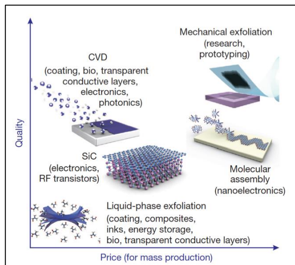
Figure 29 - Method of graphene synthesis are classified in function of their production cost and the quality produced; Depending on the application targeted, one must choose the preferred method in term of surface and quality as much as cost. Note that there is a sweet spot occupied by the CVD techniques which enable mass production of polycrystalline graphene with rather good yield. From [127].
