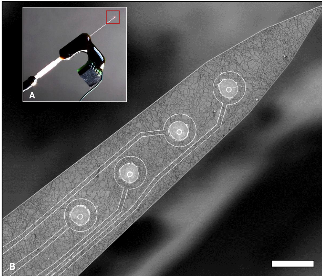
Figure 104 - Monolayer graphene conformal coating into commercial available silicon probes: A) A Neuronexus Q-trodes probe with an optical fiber integrated to the device and its connector attached B) A Neuronexus© Qtrode implant with its connector underwent direct no-carrier graphene transfer (as shown in Figure 103) to successfully achieve uniform coating of its whole surface with a preserved continuous monolayer of graphene. We distinguish the wrinkles on the graphene surface corresponding to graphene local folding. Scale bars are 50 \mu\text{m} .
