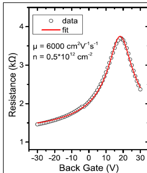
Figure 22 - Fitting channel resistance allows extraction of mobility \mu and residual carrier concentration n_0 values. A G-FET is built and its transconductance measured, plotted as resistance curve and fitted according to previous R expression, known values and incremental finding of \mu and n_0 values that are of the same order than previously found (From [99])
