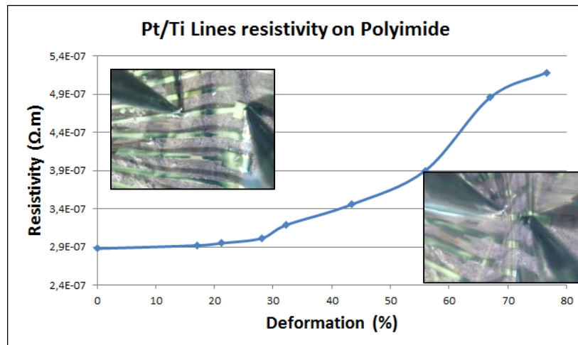
Figure 98 - Polyimide ribbon's platinum electrodes resistivity variation during deformation: The deformation rate was calculated from the distance measurement between the two probes while folding the ribbon progressively as illustrated on the two pictures.
