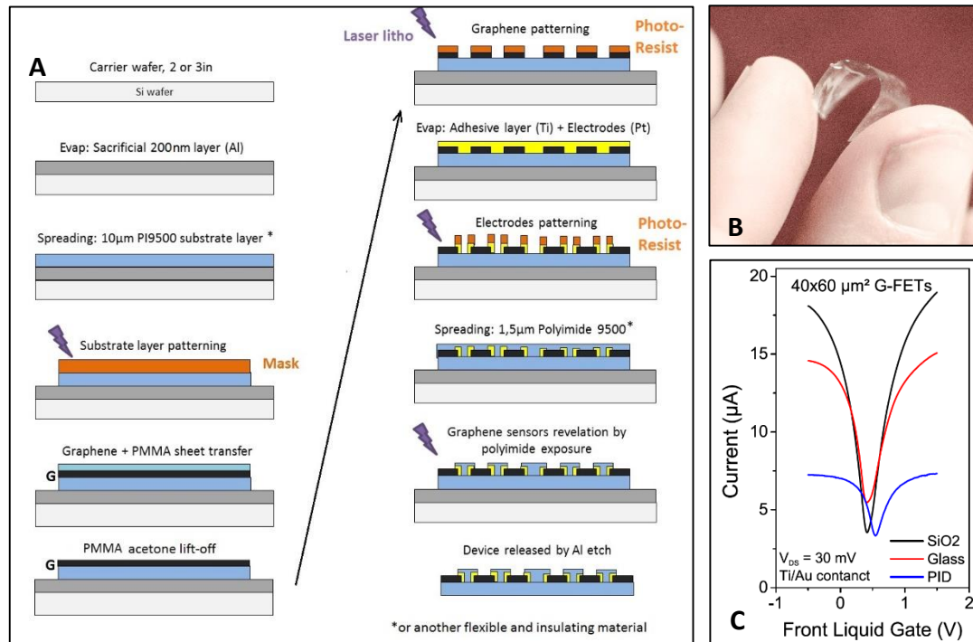
Figure 94 – Process flow to build a polyimide flexible device supporting GFETs and transconductance measurement of our GFETs devices built on different substrates: A) Pprocess flow to build a flexible device on polyimide (PID) or another flexible and insulating substrate uses the same steps than standard silicon devices except that we previously prepare a 200 nm sacrificial Al layer between the silicon wafer and the flexible material, here a 10 µm thick polyimide, in order to release the device from silicon after all the lithography and metallization steps. B) A flexible device released from silicon wafer C) Field effect in 40x60 µm G-FETs fabricated on different substrates in collaboration with F.Veliev, Institut Neel. The measurements were made in liquid gate condition in PBS solution at V_{sd}=30\text{mV} . GFETs on polyimide exhibit the higher contact resistance and a shifted Dirac point, however performance in terms of transconductance are not changing compared to SiO 2 based GFETs.
