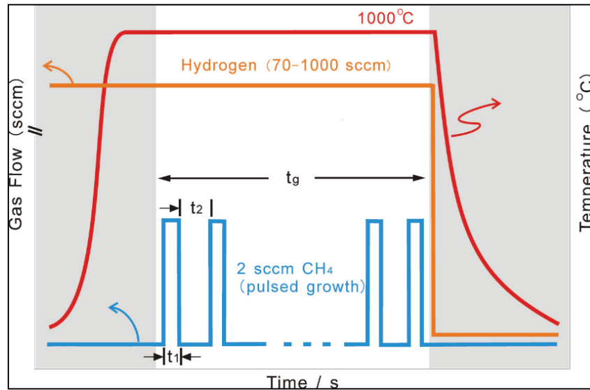
Figure 36 - Pulsed growth recipe diagram shows temperature ramp up and plateau together with injected gases: forming gas is continuously injected whereas pulses of methane injection allow the slow nucleation of carbon atoms in their sp^2 honeycomb conformation.
