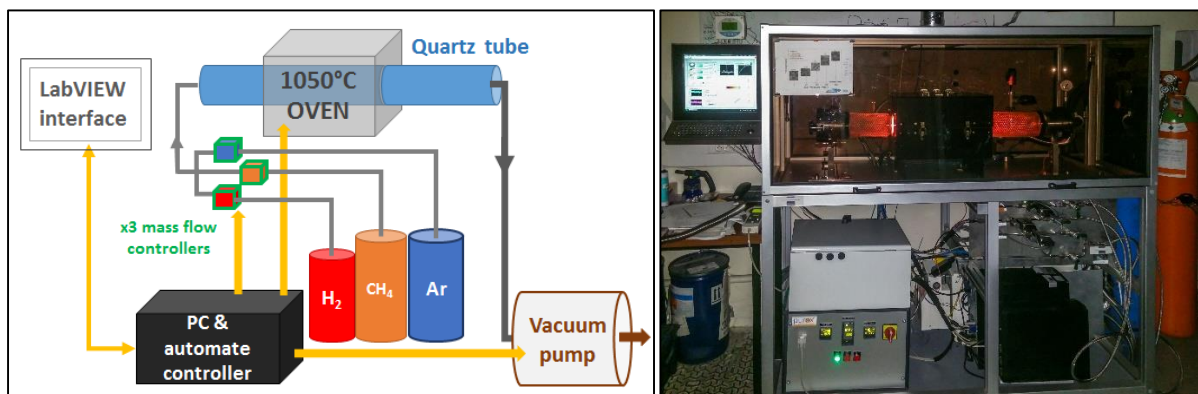
Figure 31 - CVD growth machine setup I used to grow graphene. This picture shows our CVD machine principle: mass flow controlled gases injection in an oven quartz chamber under vacuum back pumping. Recipe are semi-automated thanks to a LabVIEW program and many sensors (pression, temperature, cooling and venting systems). Photography shows our setup illustrated on left.
