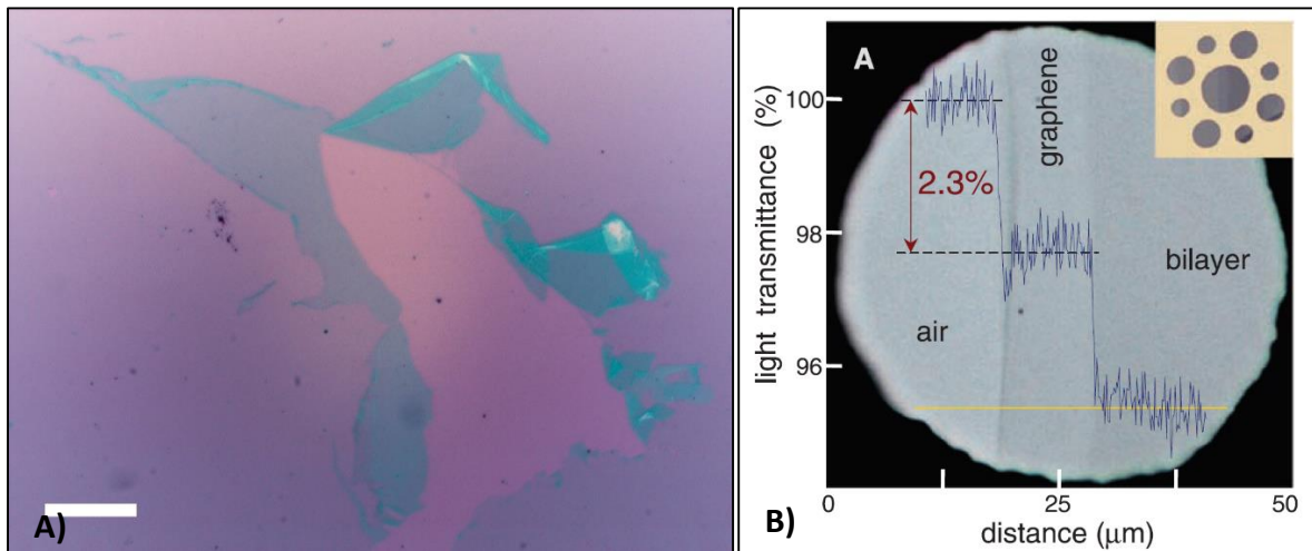
Figure 27 –Optical microscope photography shows graphene transparency relative to the number of layers: A) here one of our graphene sheet shredded on a 285nm oxide thick \text{SiO}_2 substrate. The shredding in the monolayer shows the contrast difference with bilayer and 3- layers folded graphene parts. Scale bar: 40\mu\text{m} . B) Suspended graphene on a 9 holes matrix (on top right hand corner) (illustrates 2.3% absorbance per layer. After [121])
