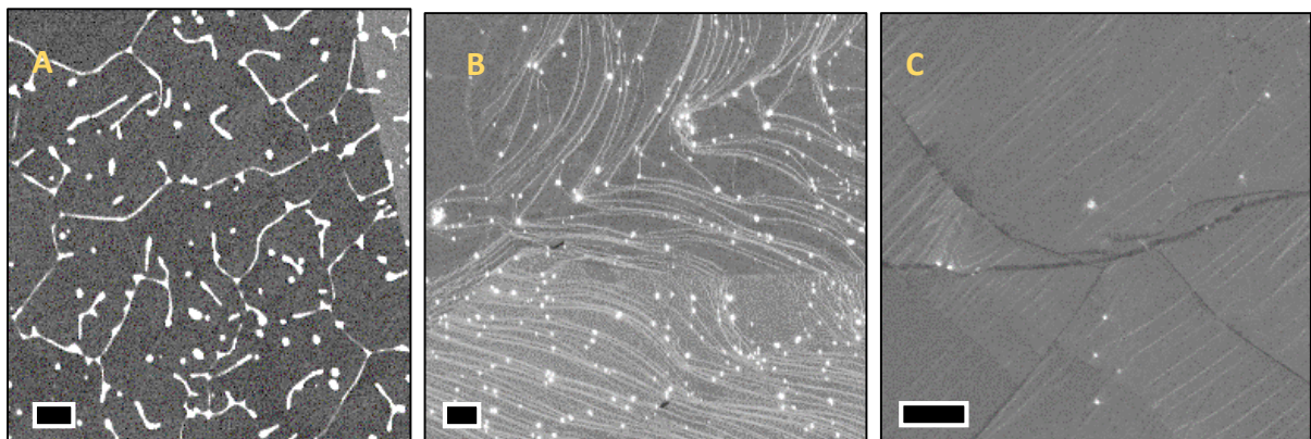
Figure 39 - SEM pictures of different growths done during this thesis show the improvement of graphene surface achieved with proper preparation of copper substrate; Graphene surface, from left to right: A #13382 copper without surface preparation besides annealing, B New copper source after annealing only and C after nitric acid cleaning recipe and annealing. Scale bars: 2µm
