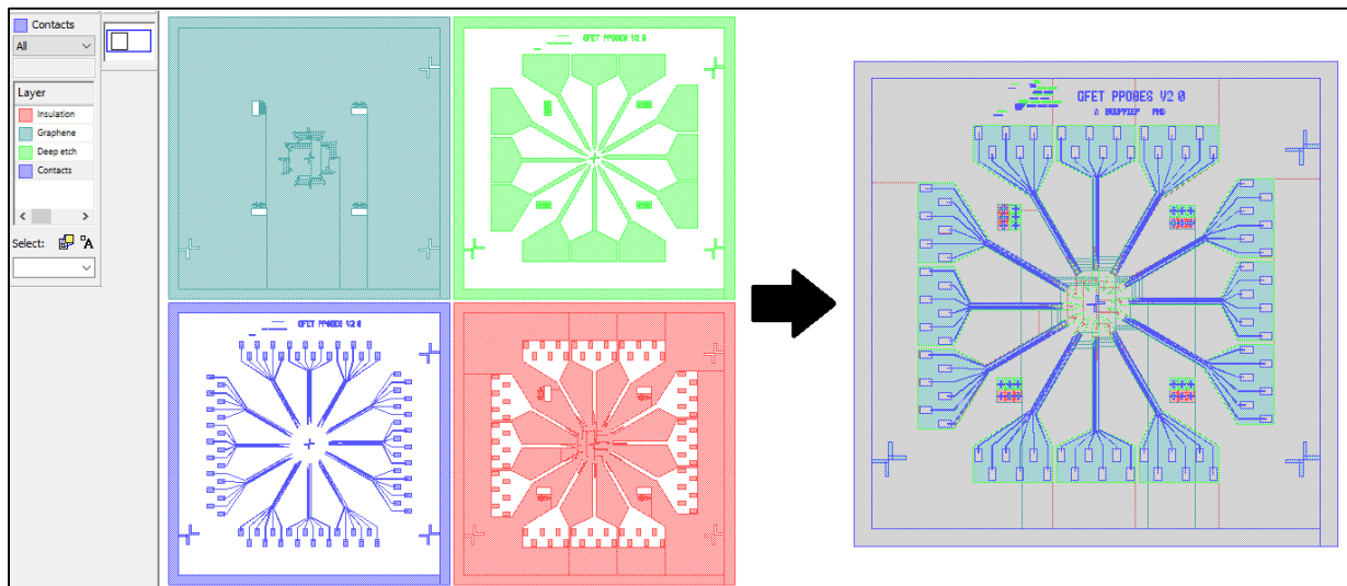
Figure 88 - Device design is made through 2D stacks representing layers that will be piled up during step by step microfabrication: here one of my first design to test Graphene FETs fabrication on 3D probes. The process will be detailed along this chapter from this first computer design step to microelectronic layer assembly.
