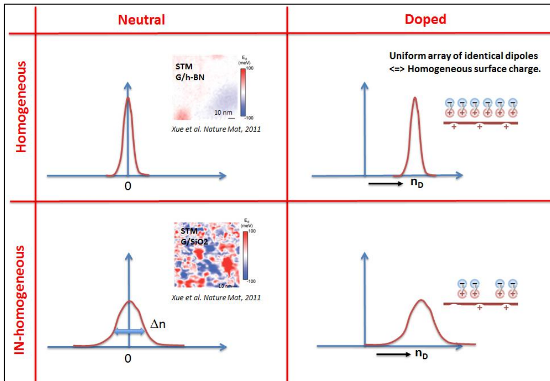
Figure 24 – Influence of doping and charge density homogeneity on FET transconductance: while doping shifts the neutral density point n_D , surface charge in-homogeneity will enlarge the peak width by increasing the local charge variation \Delta n .
