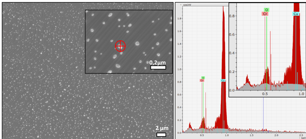
Figure 37 - SEM picture shows very dense contamination after #13382 copper thermal annealing. Contaminants are around 100nm diameters and EDX shows strong copper peak as much as chromium and oxygen peaks, suggesting a related contamination. The higher peak corresponds to copper.
