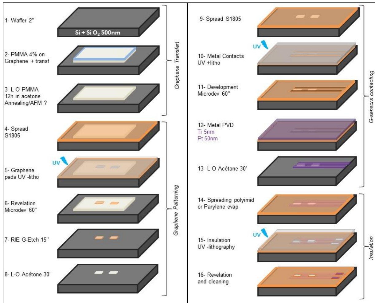
Figure 92 -Fabrication flow of G-FETs on silicon oxide: The steps are described in the text of the thesis to explain the tools used to perform devices fabrication.
