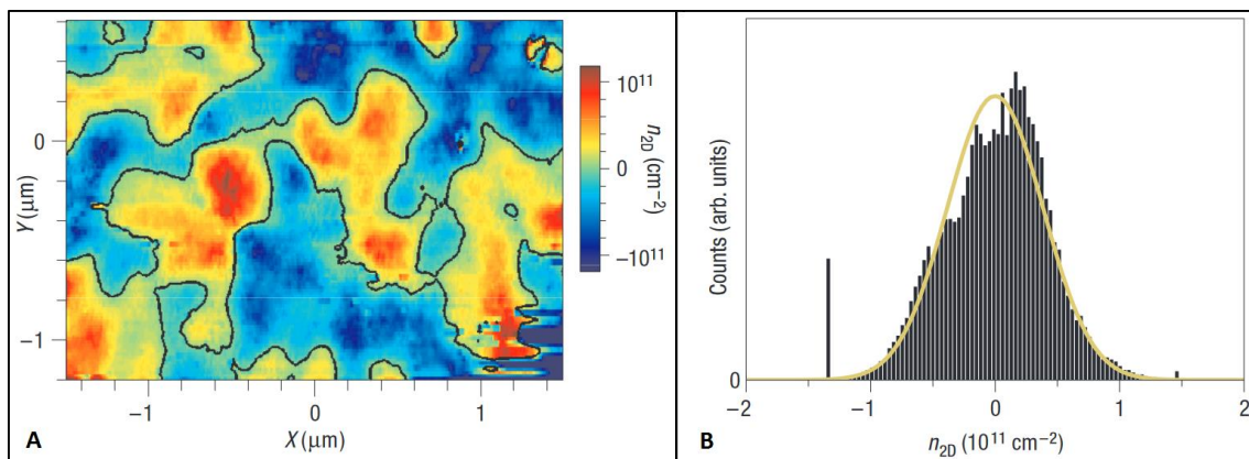
Figure 23 - Spatial density fluctuations of charge in graphene correspond to electron/hole puddles: A) Color map of spatial carrier density variations in a graphene flake extracted from surface potential measurement with a scanning single electron transistor. Blue puddles correspond to holes and red puddles to electrons, whereas the zero density are the black contour. B) The histogram of the density distribution corresponds to a Gaussian distribution, which fit extraction gives a density fluctuation of the order of \Delta n_0 = \pm 3.9 \times 10^{10} \text{ cm}^{-2} . From [102]
