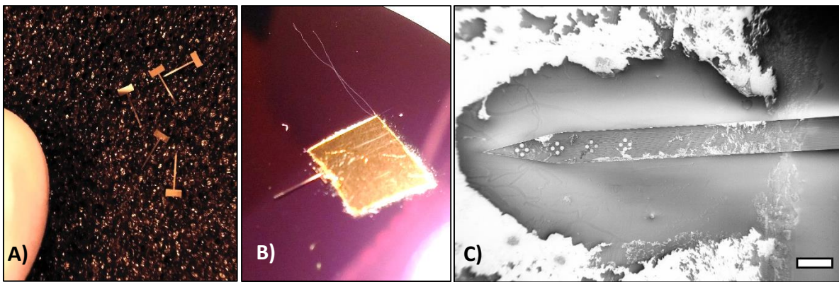
Figure 100 – Unconnected implants are easier to coat with graphene but too thick to avoid film breaking during acetone lift off A) Unconnected micro machined probes used for graphene transfer on 3D tests. B) Despite perfect lying on a silicon oxide wafer, C) SEM imaging shows that strain were yet too strong to avoid graphene blowing out all around the probe. Scale bar is 200 \mu m.
