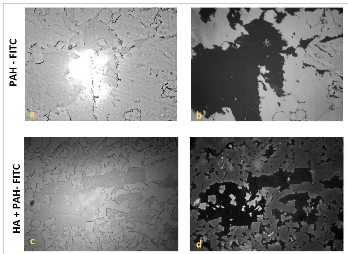
Figure 58 - Optical Microscopy on left and FITC fluorescence microscopy reveals graphene tearing off by saline solution drying: on right micrography reveals damages caused to graphene layer in black) after PAH-FITC layer adsorption; the graphene shows FITC emission, suggesting no PAH adhesion.
