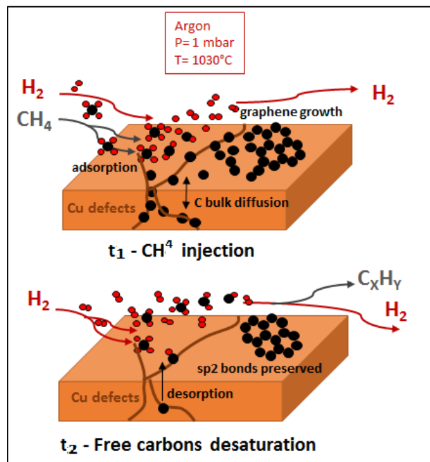
Figure 35 - Pulsed growth principle in 2 steps: \text{CH}_4 injection and \text{H}_2 alone alternance allow desorption of diffused carbon atoms in bulk through Copper defect. \text{sp}^2 bonds are strong enough to overcome the \text{H}_2 "etching of non- \text{sp}^2 bonded carbon atoms. This alternance allows monolayer growth favoring only \text{sp}^2 surface segregation of carbon atoms.
