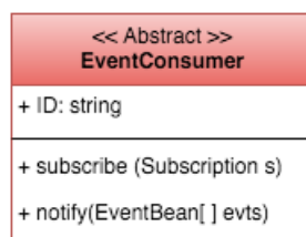
Figure 5.13 – Base class for defining a consumer
