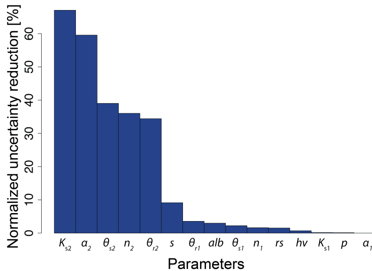
FIGURE 5.4: Parameter importance in terms on their effects on groundwater recharge predictive uncertainty
