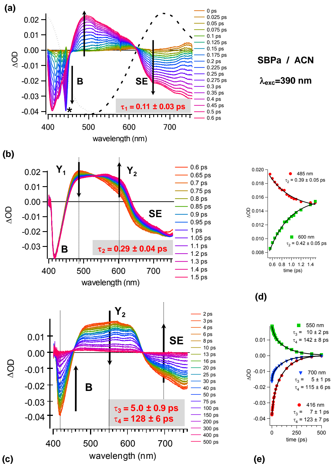
Figure V.1 Femtosecond transient absorption spectral evolution of SBPa in ACN following laser excitation at 390 nm, divided into three temporal windows: a) [-1 - 0.6 \text{ ps}] , b) [0.6 - 1.5 \text{ ps}] , c) [2 - 500 \text{ ps}] . Characteristic times found using the global fitting method are indicated in red. Graphs d) and e) show typical kinetics for chosen wavelengths and their fits with mono-exponential and bi-exponential functions, respectively. The star indicate stimulated Raman pick of the solvent. Pump-probe correlation time: \tau = 180 \text{ fs}
