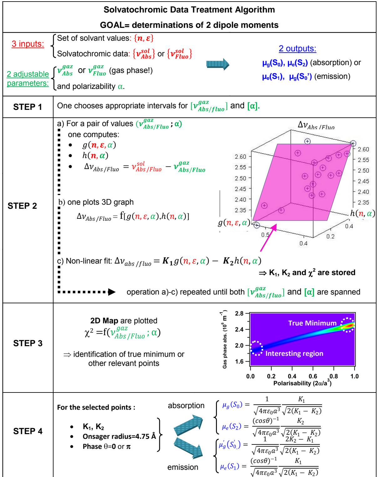
Figure IV.17 Solvatochromic data treatment algorithm for determination of dipole moments from stationary absorption and fluorescence data.
