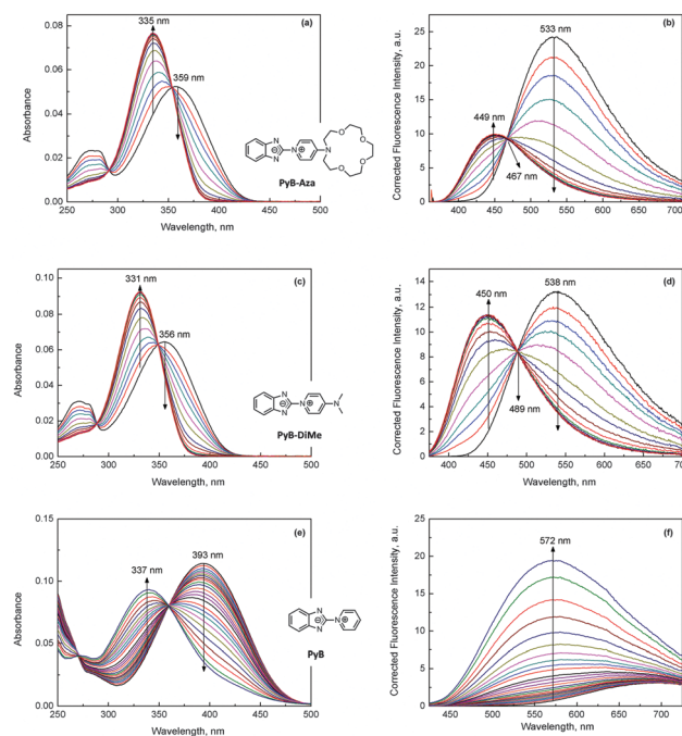
Fig. 2 Absorption (a, c and e) and fluorescence (b, d and f) spectra of PyB, PyB-DiMe and PyB-Aza in the presence of increasing concentrations of \text{Ca}^{2+} in MeCN; (a and b) [PyB-Aza] = 2.5 \mu\text{M} , \lambda_{\text{ex}} = 359 nm; (c and d) [PyB-DiMe] = 2.5 \mu\text{M} , \lambda_{\text{ex}} = 354 nm; (e and f) [PyB] = 10 \mu\text{M} , \lambda_{\text{ex}} = 393 nm.
