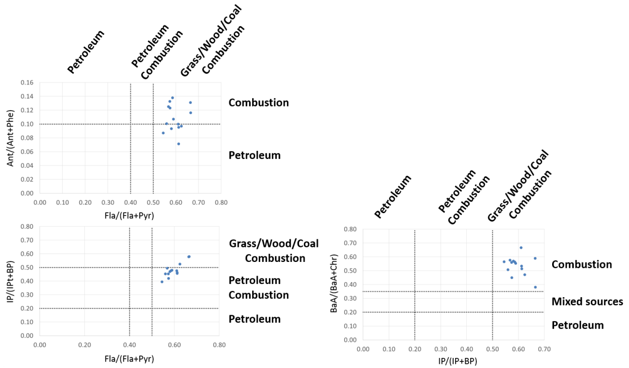
SI-8. PAHs sources in surface sediments in the Heron Lake during the screening of January 2015.
