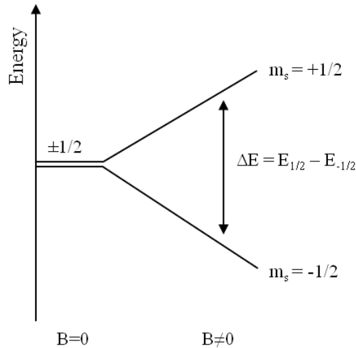
Figure I.3: Zeeman effect.
