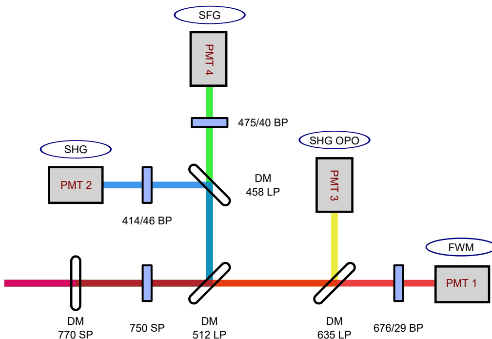
Figure 1.8: Detail of the detection area in the experimental setup (Fig. 1.7). The signal is deviated from the excitation path after the objective using a dichroic mirror (DM) at the microscope and spectrally cleaned by a shortpass filter (SP). It is then split by extra dichroic mirrors and further filtered by bandpass filters (BP). There are four photo-multiplier tubes (PMT) that collect the four different nonlinear signals (FWM, SHG from each beam and SFG).
