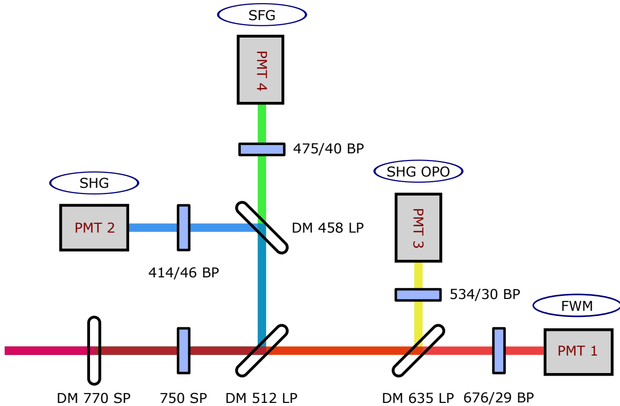
Figure 3.3: Detail of the PMT Detectors in the experimental setup (Fig. 1.7). The signal is spectrally cleaned by a Shortpass filter (SP) and then split by Dichroic mirrors (DM), and further filtered by Bandpass filters (BP). There are four Photo-multiplier tubes (PMT) that collect four different nonlinear signals (FWM, SHG Ti:Sa, SHG OPO and SFG). This combination of filters is changed accordingly when the excitation wavelengths are changed.
