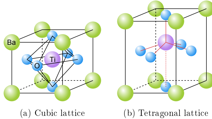
Figure 3.1: Two possible atomic distributions for BaTiO 3 . (a) shows a cubic lattice where the Ti atom is in the center of the unit cell, Ba atoms are on the corners, and O atoms are at the faces. (b) shows a tetragonal lattice where the Ti atom has displaced out of the center and it has “pushed” the atoms around it in the same direction, due to electric forces. An electric dipole is thus created.
