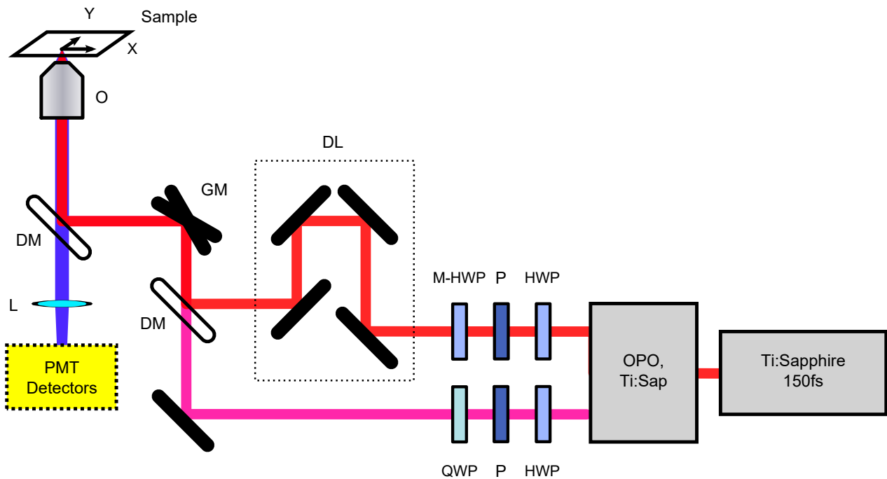
Figure 5.5: Experimental setup with a Ti:Sapphire pulsed laser (830 nm) and an Optical parametric oscillator (OPO, 1088 nm), a Delay line for one of the beams (DL), Galvonometric scan mirrors (GM), Dichroic mirrors (DM), a 40\times 1.15 NA Objective lens (O), Sample (S), Polarizers (P), Halfwave plates (HWP), of one which is Motorized (M-HWP), a Lens (L), and the detection is done by a system of PMT detectors (PMT), which is detailed in Fig. 5.6.
