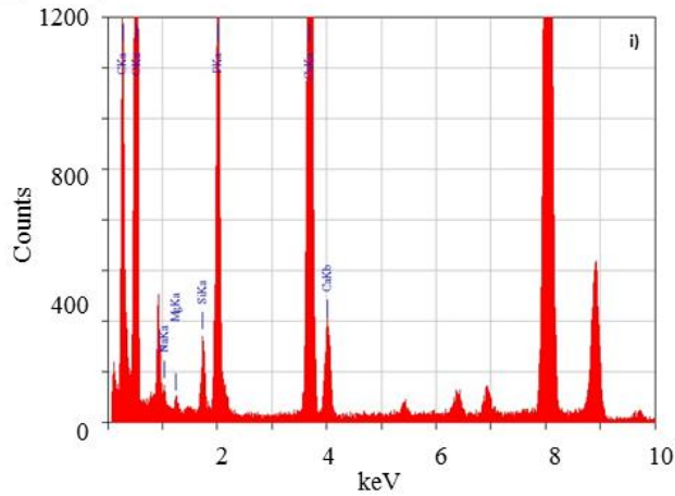
Figure A.3.2. Scanning EDX of the 700 °C and 600 °C bone samples.
