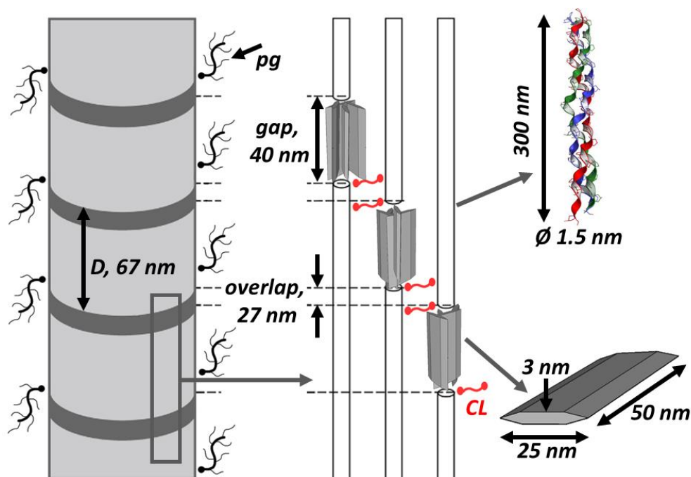
Figure 1.13. Mineralized fibril structure: collagen molecules and mineral nanocrystals organization ( D - collagen periodicity). The gap and overlap regions are the source of characteristic 67 nm collagen banding. Mineral nanocrystals that are located within the gap zones are oriented with the c -axis being parallel to the collagen fibrils.
