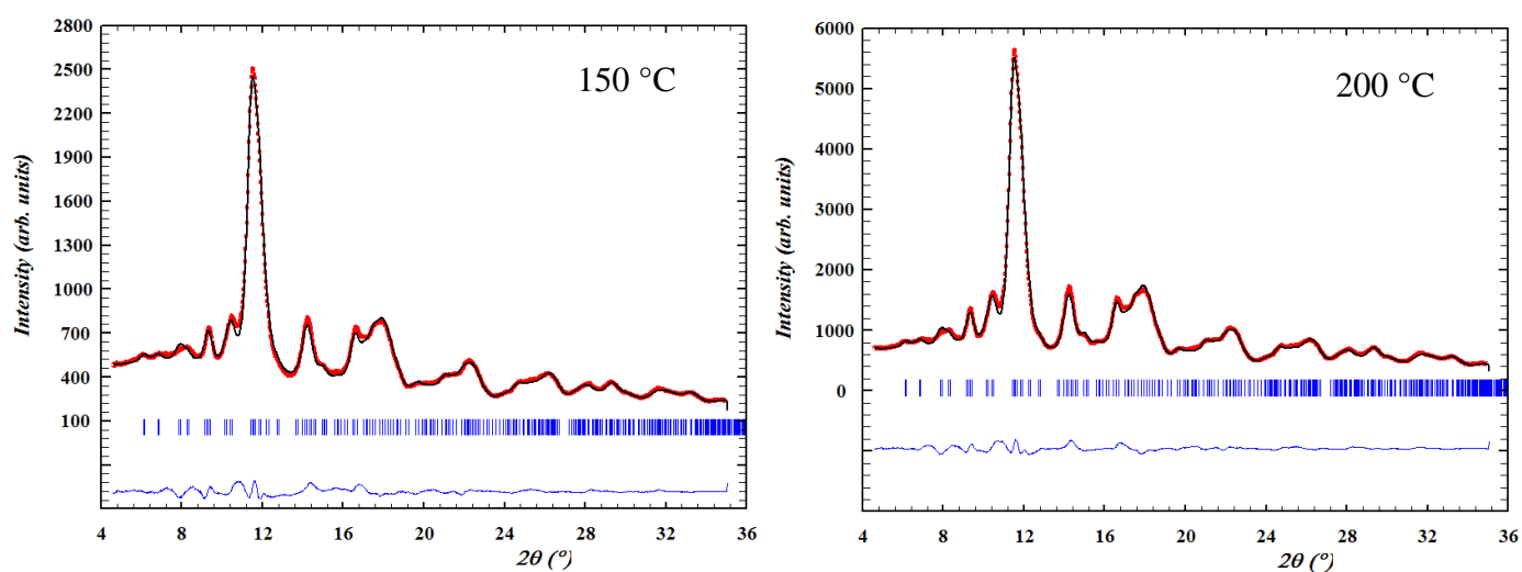
Figure A.4.2. Rietveld-refined diffraction patterns for the 150 °C and 200 °C samples.
