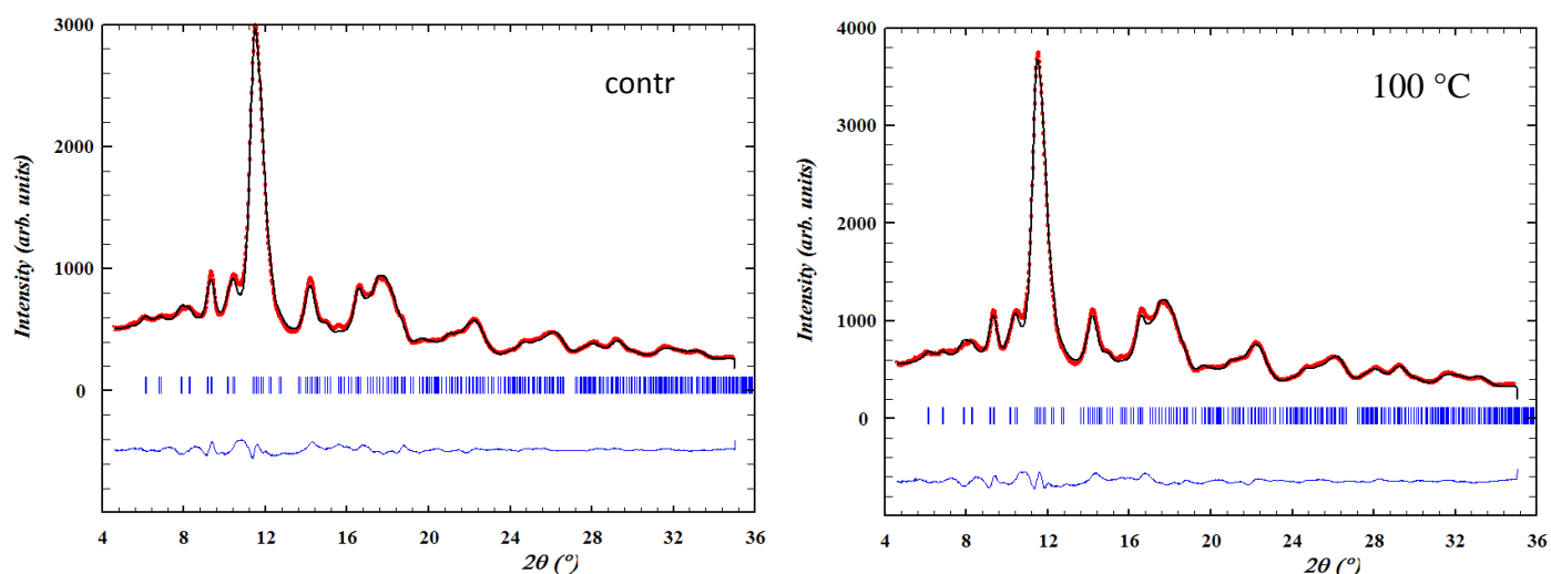
Figure A.4.1. Rietveld-refined diffraction patterns for the control and 100 °C samples.
