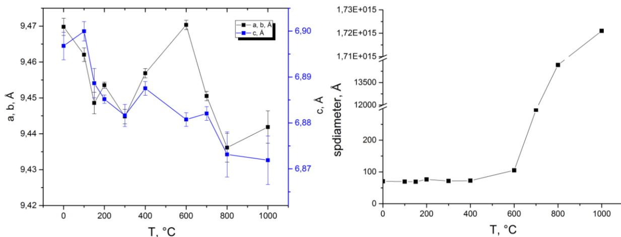
Figure 3.54. Left: lattice parameters vs temperature. Right: spdiometer vs temperature (errors are of the order of 10^{-2} \text{ \AA}^{-1} ).
