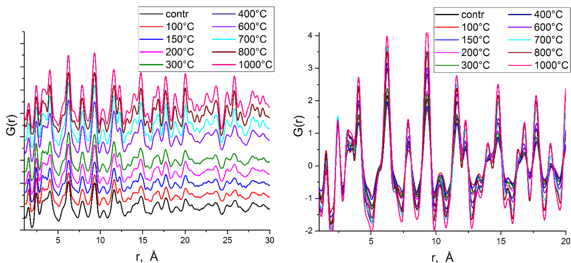
Figure 3.51. G(r) for heated bone with different zoom. Left - offset, right - no offset.
