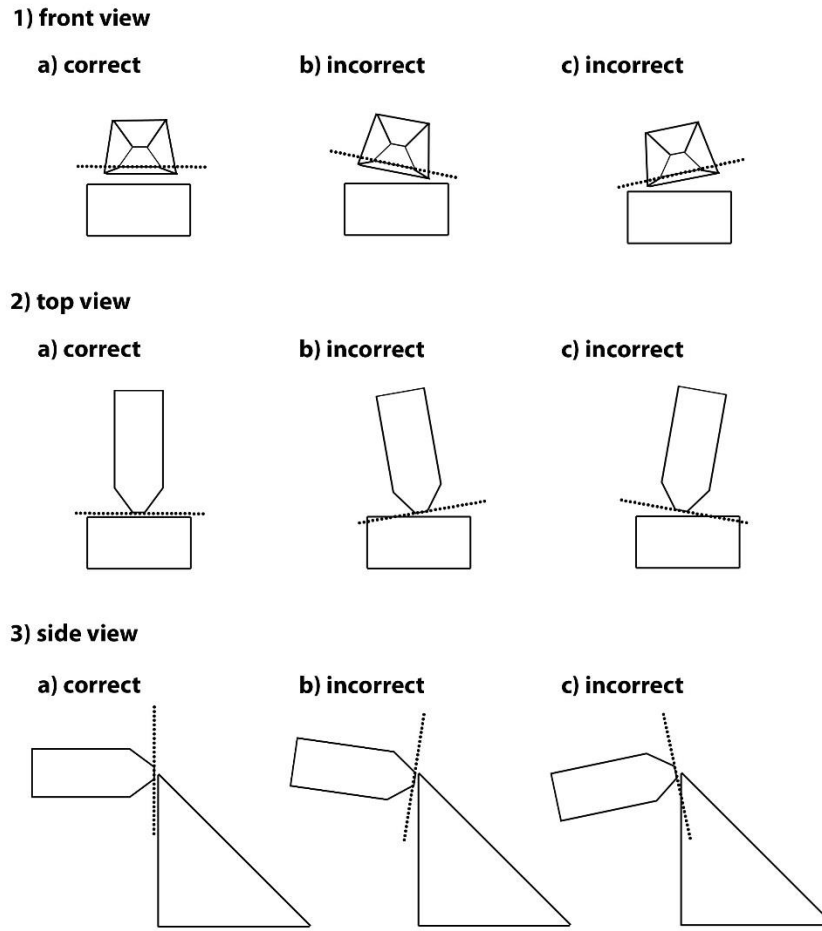
Figure A.4. Aligning the resin block and knife for thin sectioning. Possible correct and incorrect positions of the block with respect to the knife edge in all three dimensions [208]. Advance the block face towards the knife and observe the reflection of the knife edge getting thinner and thinner. Use the 1 \mu m advance once you get very close to the knife edge.
