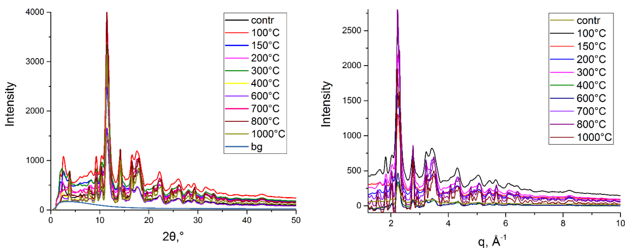
Figure 3.46. XRD spectra for heated bone. Left: I(2\theta) . Right: I(q) .
