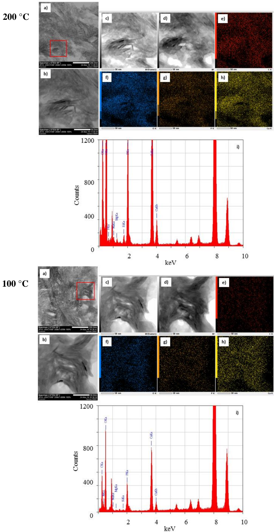
Figure A.3.4. Scanning EDX of the 200 °C and 100 °C bone samples.
