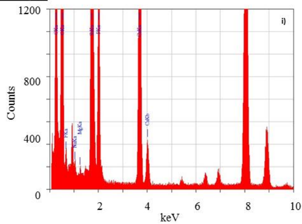
Figure A.3.3. Scanning EDX of the 400 °C and 300 °C bone samples.
