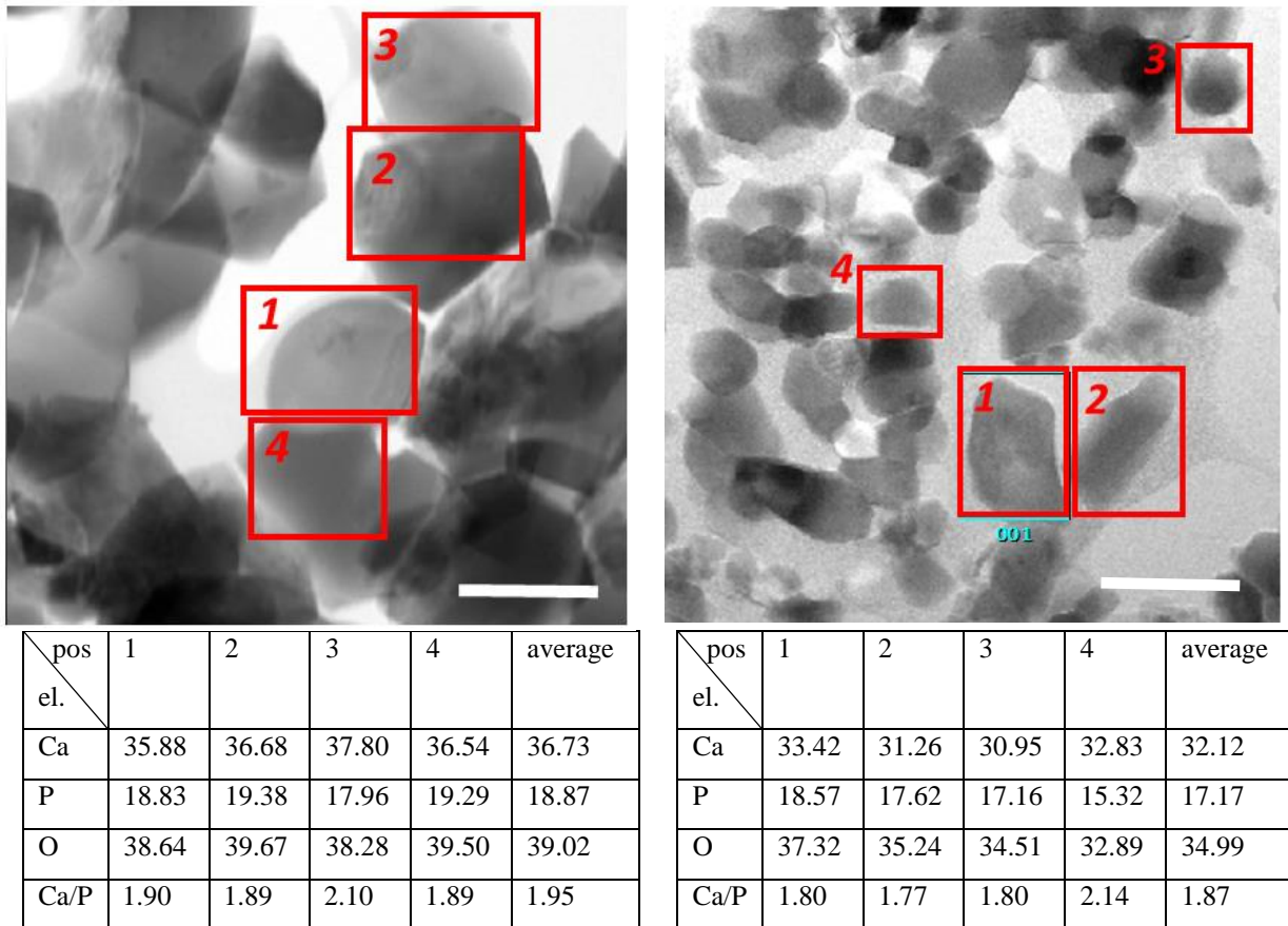
Figure 3.35. Single crystal EDX analysis. Bright field images showing scan positions with corresponding elemental mass concentration (in %) and Ca/P ratio for 1000 °C (left) and 800 °C (right).
