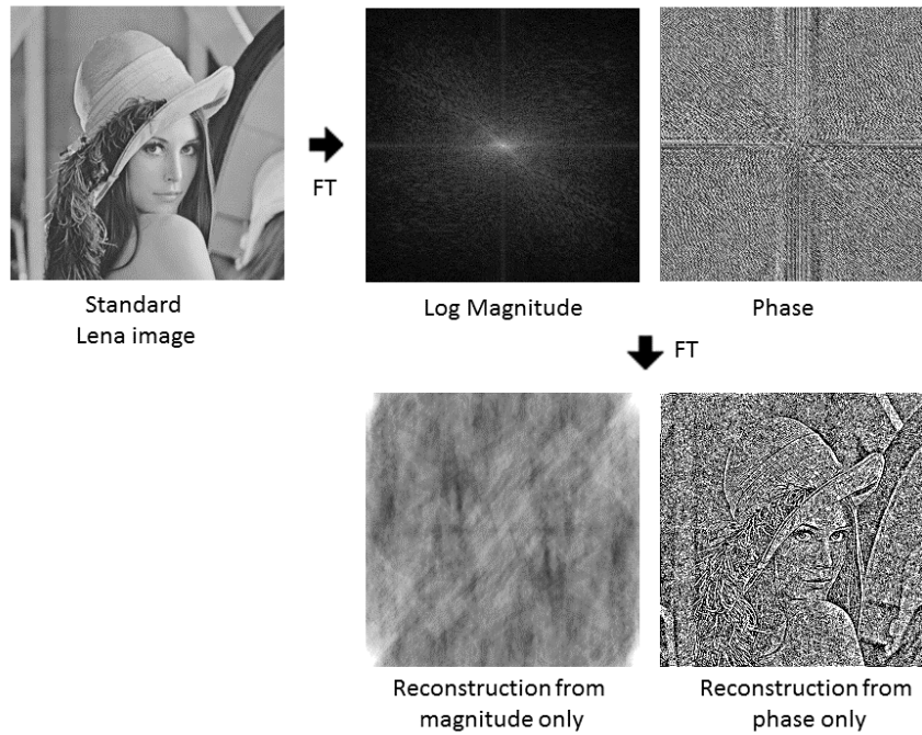
Figure 2.13. Illustration of the phase problem. Separated Fourier transforms of magnitude and phase (calculated with ImageMagick software).
