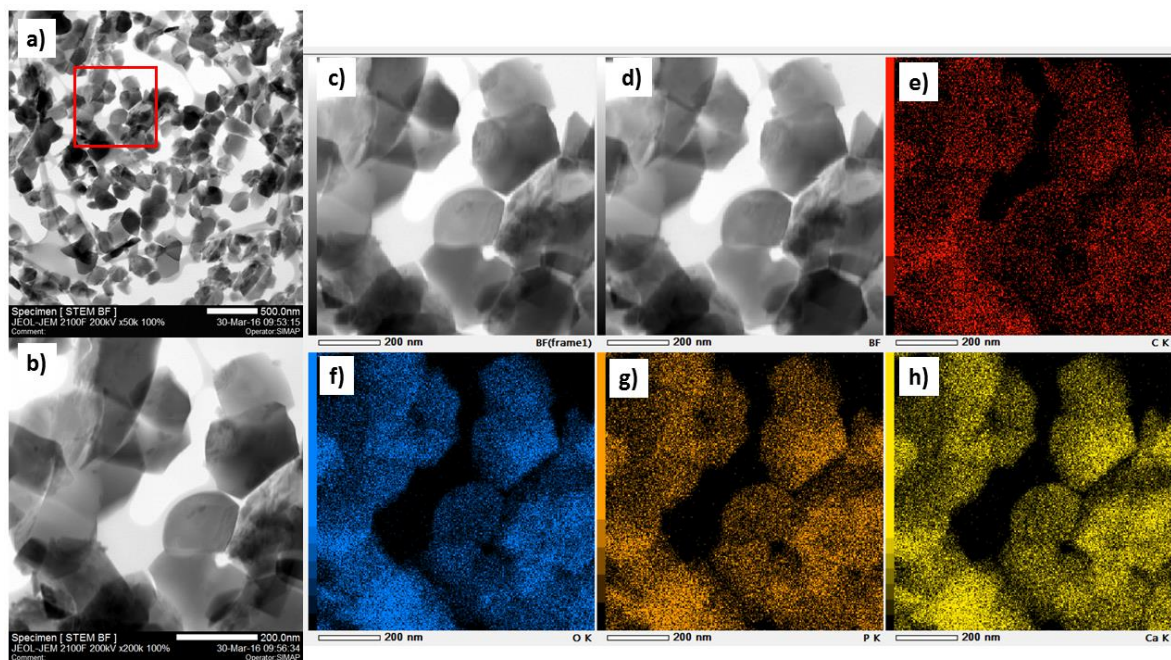
Figure 3.31. Scanning EDX of the 1000 °C bone sample: a), b) bright field images of the scan position; c), d) bright field images before the first and the last scanning frame; e), f), g), h) elemental maps of C, O, P and Ca, respectively.
