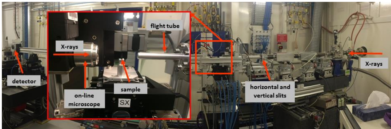
Figure 2.22. Experimental setup for CXDI experiment at ID10.
