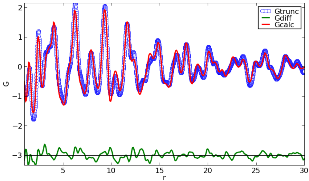
Figure A.4.6. PDFgui fit for the control sample. Blue circles: experimental PDF; red curve: modelled PDF; green: misfit function.
