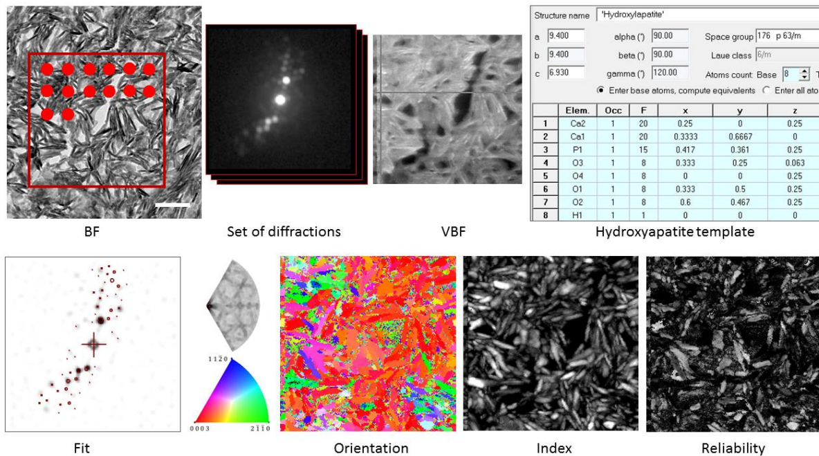
Figure 2.24. General scheme of ACOM-TEM acquisition and data interpretation: bright field image of bone with shown scanning area, set of diffraction patterns, virtual bright field image, structure template for hydroxyapatite, example of fit with stereographic projection, orientation map with inverse pole figure color map, index and reliability maps, which are explained in the following.
