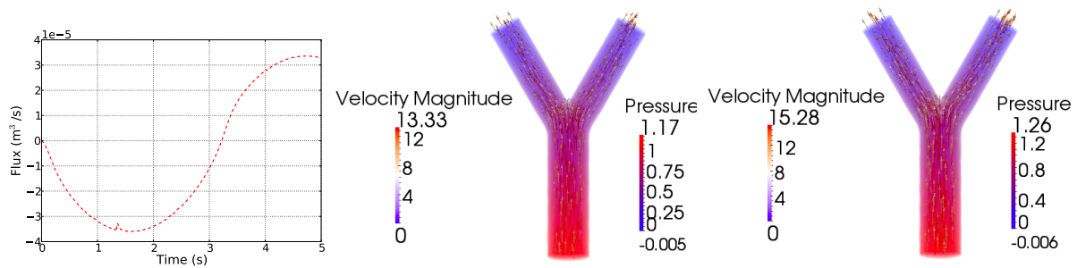
Figure 2.17: Left: flux (m³/s) as a function of time (s) at the inlet. Center and right: velocity vector (in 10 -6 m/s) and pressure fields (in 10 -1 Pa) at t = 0.12 s (center) and at t = 0.13 s (right). Nonsymmetric stress tensor, basic formulation of the convective term, coarse mesh, \Delta t = 0.01 s and p_{\text{in}}(t) = 10 \sin(t) in 10 -1 Pa. With stabilization described in Section 2.3.4, \beta = 1 .
