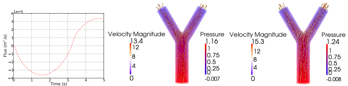
Figure 2.18: Left: flux (m³/s) as a function of time (s) at the inlet. Center and right: velocity vector (in 10 -6 m/s) and pressure fields (in 10 -1 Pa) at t = 0.12 s (center) and at t = 0.13 s (right). Symmetric stress tensor, basic formulation of the convective term, coarse mesh, \Delta t = 0.01 s and p_{\text{in}}(t) = 10 \sin(t) in 10 -1 Pa. With stabilization described in Section 2.3.4, \beta = 1 .
