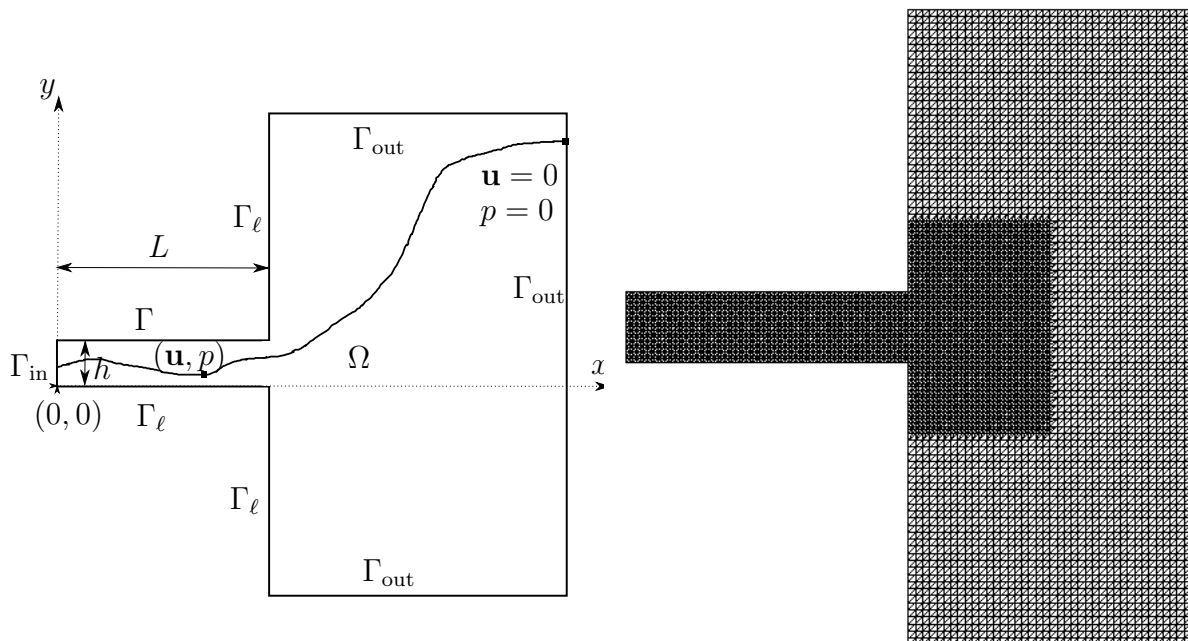
Figure 4.10: Domain (left) and mesh (right).
