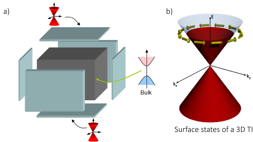
Figure 1.10. – a) Schematic description of a three dimensional topological insulator (3D TI). b) Band structure of the surface states on a 3D TI. The arrows represent the spin of the electrons and are always perpendicular to its momentum. Adapted from [164].
