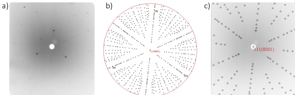
Figure 2.10. – Laue diffraction of BSTS. a) measurement of our BSTS. b) Prediction of the diffraction pattern for a rhombohedral crystal structure cleaved orthogonal to the c axis. c) Superposition of a) and b).
