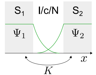
Figure 4.1 – Schematic of a Josephson junction. The order parameters of each lead decreases outside the superconducting region. The overlap between \Psi_1 and \Psi_2 defines the coupling constant K .
