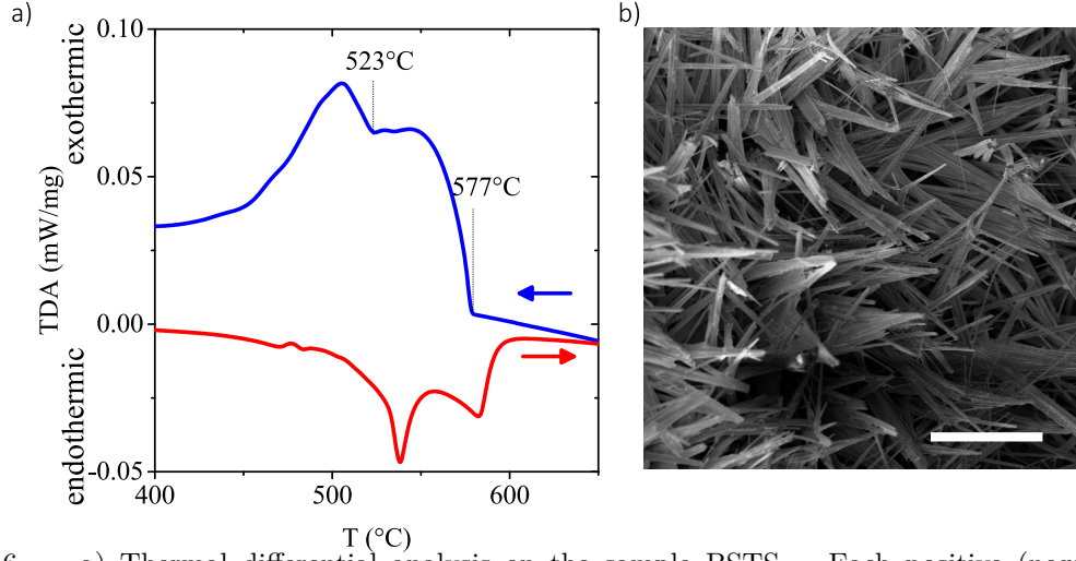
Figure 2.6. – a) Thermal differential analysis on the sample \text{BSTS}_b . Each positive (negative) spike corresponds to an exothermic (endothermic) reaction. The heating was at 300\text{ °C/h} and the cooling at 1200\text{ °C/h} . b) Scanning electron microscopy image of the surface of the sample \text{BSTS}_b . The horizontal white line is 50\text{ }\mu\text{m} for scale.
