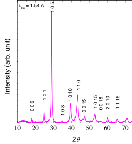
Figure 2.9. – Powder X-ray diffraction of \text{BSTS}_d . The expected peaks are labeled by their hkl index.
