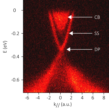
Figure 6.1. – Angle resolved photo-emission spectroscopy of \text{Bi}_2\text{Se}_3 measured at SOLEIL (collaboration J.-Y. Veuillen, J. Avila and M. C. Asensio). The energy is measured with respect to the Fermi level ( E_F = 25.7 eV) versus the parallel wave vector. The surface states (SS) cross in a linear way at the Dirac point (DP) 0.35 eV below the Fermi level. The latter is placed in the bulk conduction band (CB) which leads to a bulk metallic behavior.
