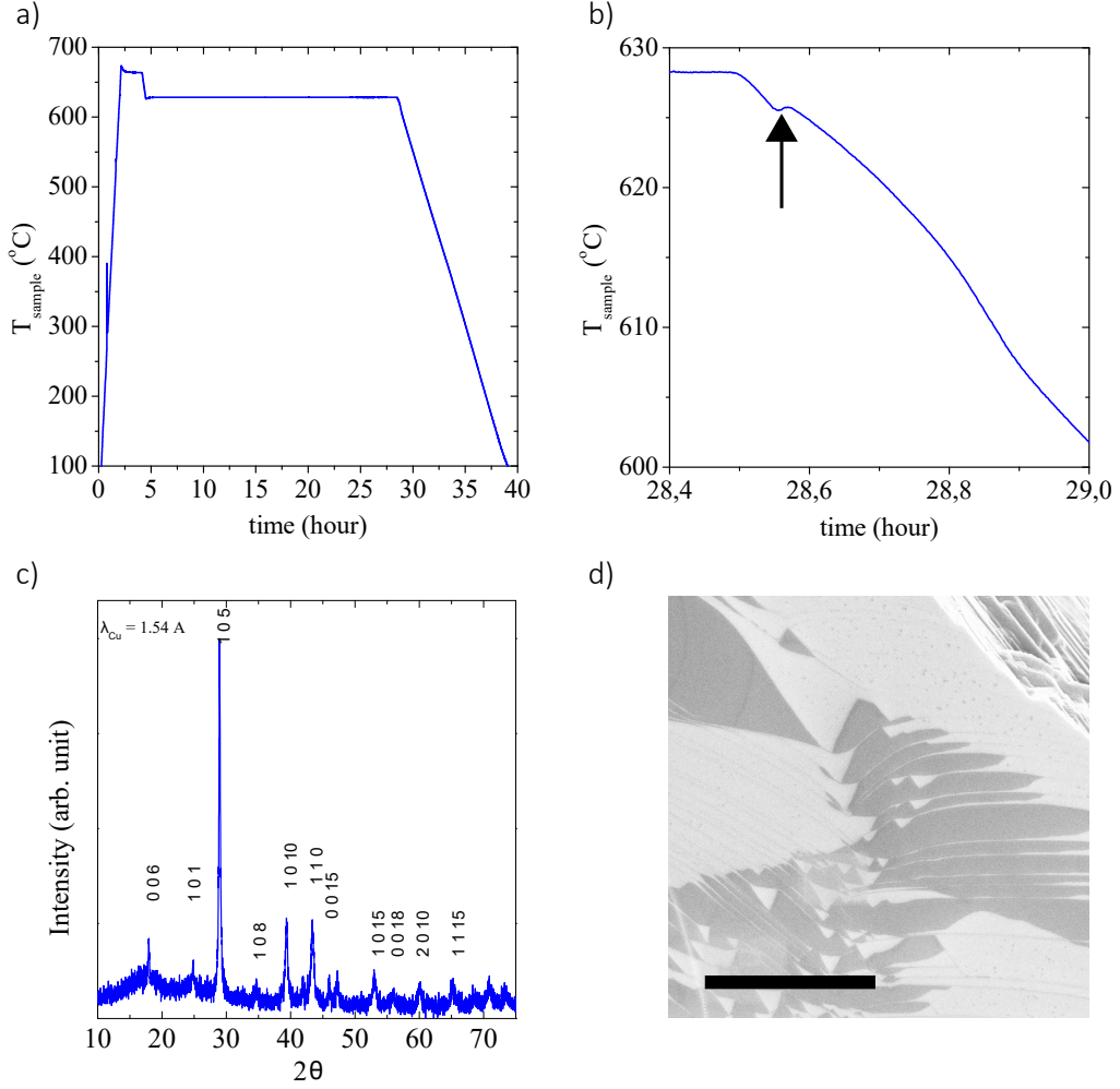
Figure 2.7. – Details on BSTS c : a) Temperature of the quartz tube during the growth. b) Zoom of a) during the cooldown. Highlighted by the black arrow, a reaction occurs at 625 °C after the landing at 3 628 °C. c) Powder X-ray diffraction of BSTS c . The expected hkl plane indexes are labeled. d) Scanning electron microscopy image of BSTS c with an in-lens detector. Two phases are visible. The horizontal black line is 50 μm for scale.
