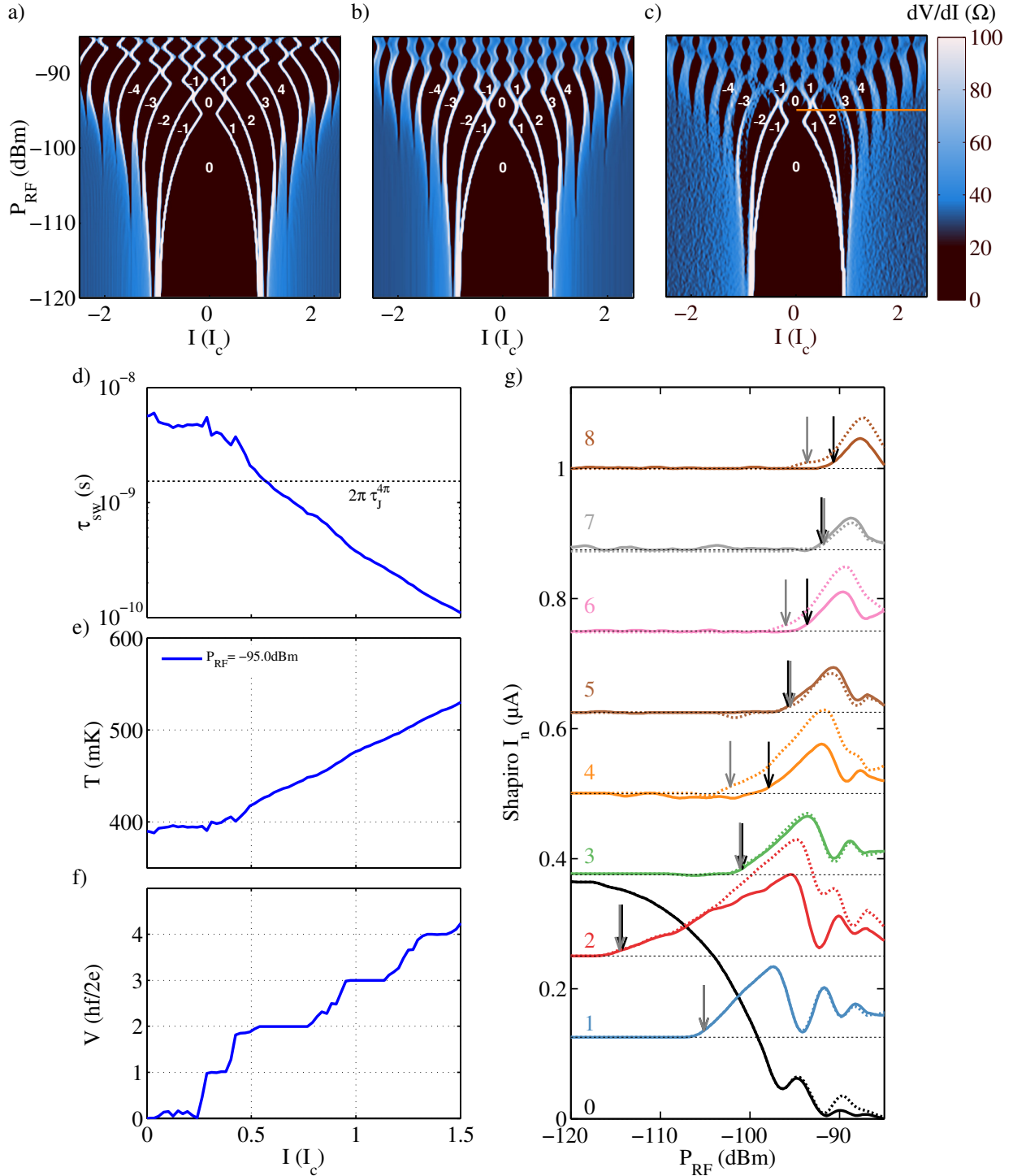
Figure 5.19. – Result of RSJ model of two JJ with 20% (80%) of 4\pi ( 2\pi ) supercurrent, irradiated at 2 GHz, with R = 30 \Omega , I_c^{4\pi} = 500 nA. a-c) Differential resistance maps vs the bias current I_{DC} and the RF power P_{RF} of simulations a) without heating effects, b) with Joule heating on the conventional supercurrent, c) with Joule heating and thermally activated poisoning. The thermodynamic parameters are the following : \mathcal{V} = 0.20 \mu m^3 , \Delta_{mini} = 500 \mu eV and \tau_0 = 1.9 fs. The indexes label the first Shapiro steps. The orange line show the line-cut corresponding to d-f). d-f) Current dependence at -95 dBm of the switching time (d), the electronic temperature (e) and the DC voltage (f). g) Amplitude of each Shapiro step versus radio frequency amplitude. The continuous lines correspond to the extracted I_n from figure c) (with poisoning) while the dotted lines correspond to the same simulation without poisoning effects b) (but still with heating on the 2\pi supercurrent). We indicate the appearance of each steps by black (gray) arrows corresponding to the simulation with (without) poisoning.
