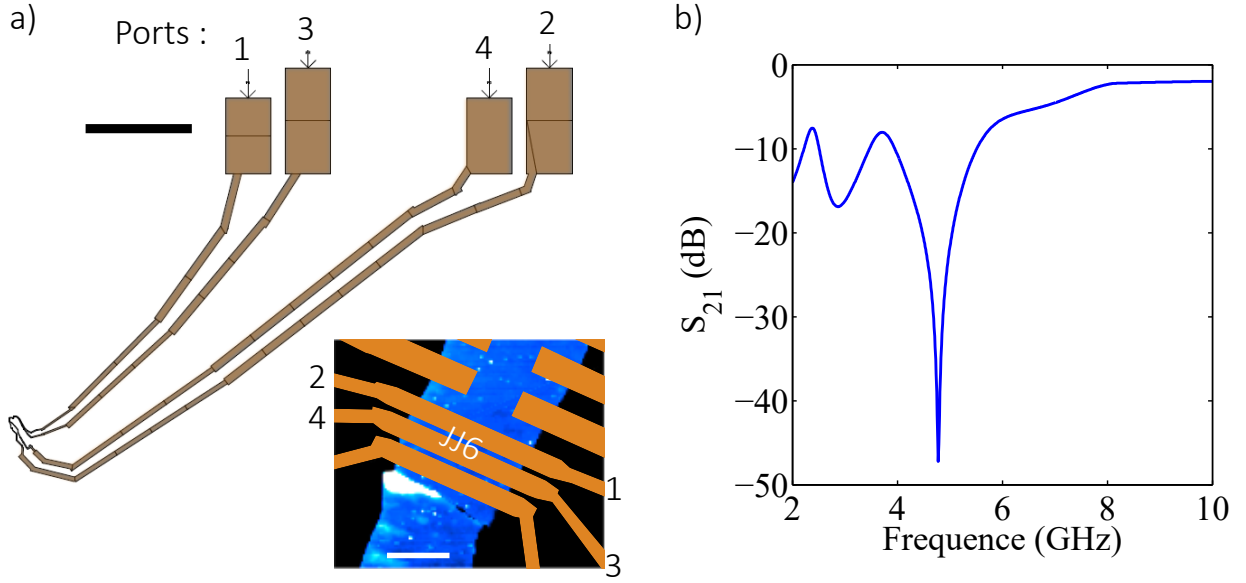
Figure 7.7. – a) Design of the electrodes patterned on the substrate that form the junction JJ6. The pads are labeled from 1 to 4. The black line is 250 \mu\text{m} for scale. (inset) False colors image of an atomic force microscopy. In blue is the flake of BSTS and in orange are the design of the superconducting electrodes. The Junction JJ6 is formed in-between the two leads that are connected to the four labeled pads. The white line is 1 \mu\text{m} for scale. b) Transmission matrix coefficient from line 1 to line 2 versus the frequency of the input signal. A dip in the coefficient means a poor transmission of the signal that stays located inside the sample.
