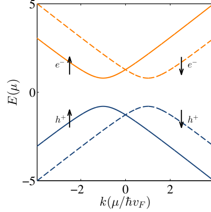
Figure 4.12 – Energy dispersion relation for the 4 energy states of (4.51) with the following parameters : \mu = 1 \text{ meV} , v_F = 5 \times 10^5 \text{ m s}^{-1} and \Delta = 800 \mu\text{eV} . Solid lines corresponds to, say, up spin, and dashed line to the opposite spin.
