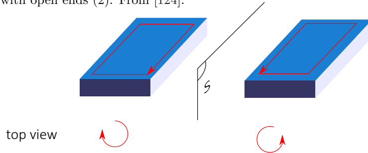
Figure 1.4. – Schematic of the chiral property of the quantum Hall edge state. The initial system (left) has an edge state rotating clockwise. The symmetric with respect to a vertical plane changes the rotation direction of the edge state. The right system is not identical to the left one.
