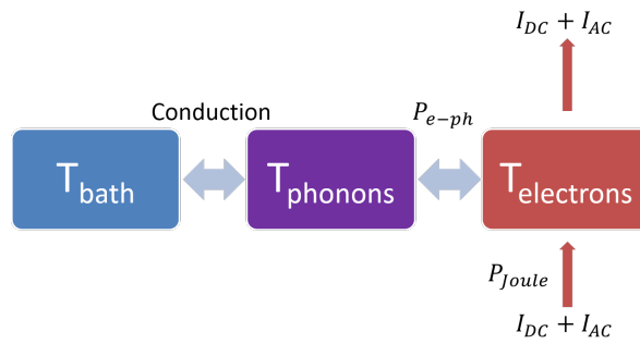
Figure 5.6. – Schematic of heat transfer between the three baths at different temperatures defined in a mesoscopic system. Heating comes mainly from Joule heating and is dissipated through the phonons of the system and the substrate.
