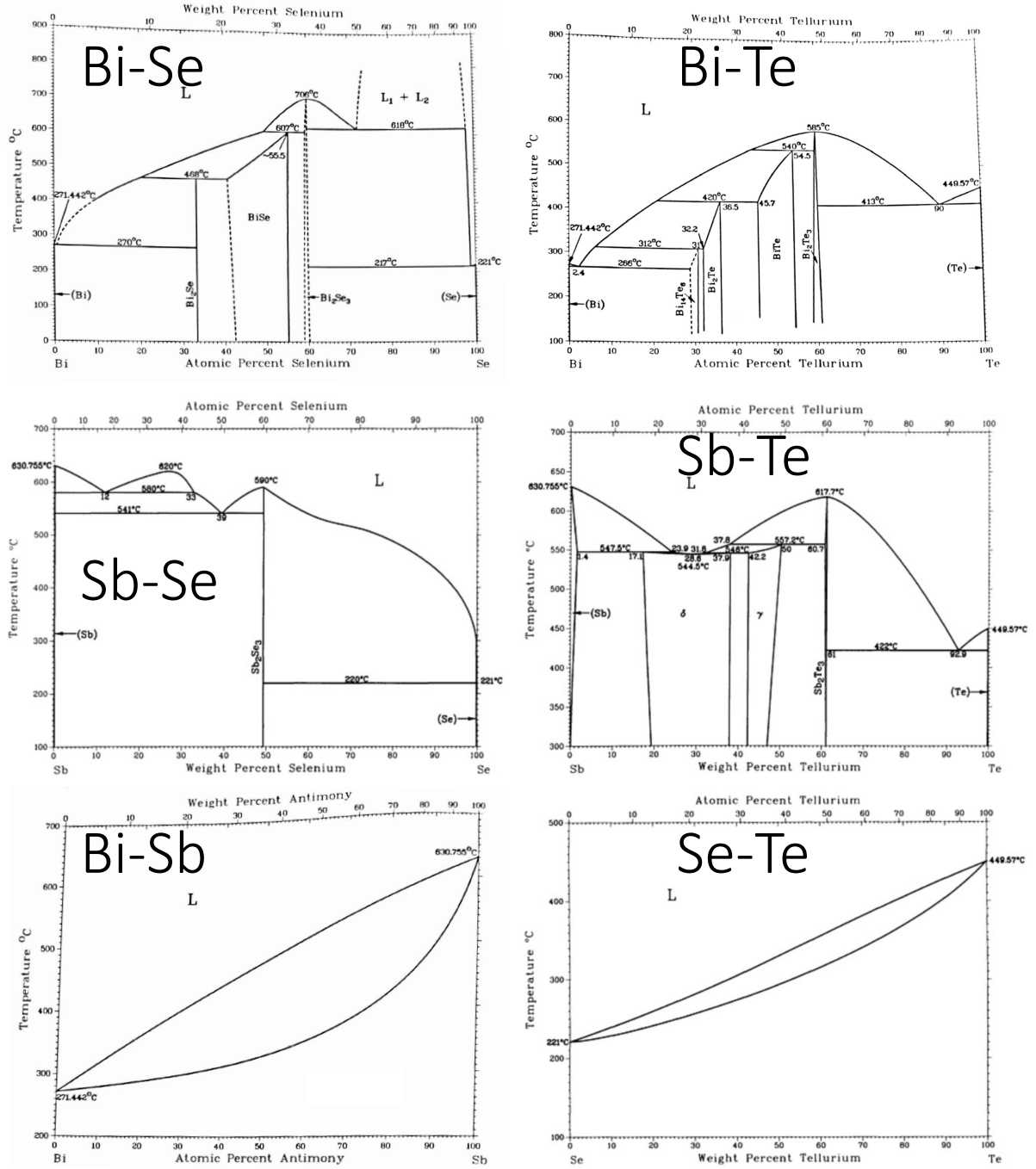
Figure 2.4. – Binary phase diagrams between the four components of the material BiSbTeSe 2 . These graphs are extracted from Massalski & Okamoto [119]. L represents the liquid phase and the other compounds are labelled with their melting temperatures. We should recall that only the binary compounds Bi 2 Se 3 , Bi 2 Te 3 and Sb 2 Te 3 are topological insulators with the rhombohedral crystallographic structure.
