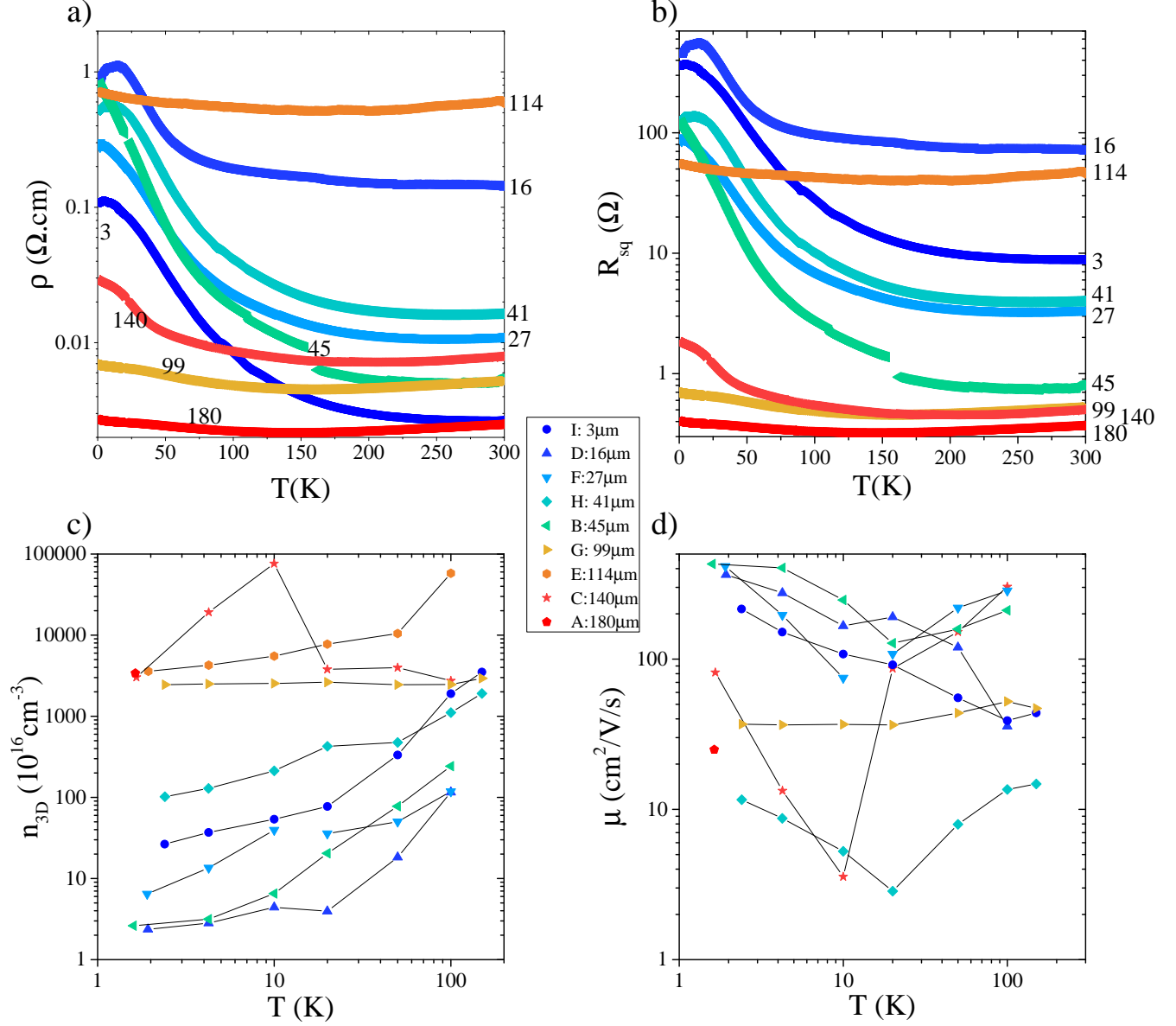
Figure 2.13. – Transport properties of samples extracted from \text{BSTS}_d . All samples are manually cleaved in the shape of a rectangle. The contact in silver paste are placed in the geometry of a Hall bar. Their thicknesses are estimated with optical microscopy. The resistivity (a) and sheet resistance (b) are measured versus temperature. At several temperatures, we perform Hall measurements to estimate the carrier density (c) and electron mobility (d).
