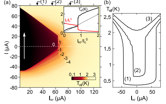
Figure 5.10 – (a) Calculated electronic temperature T_{\text{el}} map corresponding to the situation of figure 5.9, i.e. for a device at T_{\text{bath}} = 100 mK. The first Shapiro steps are labeled. The white arrow indicates the direction of the sweep in the simulation. Inset: Line cut of this map showing the electronic temperature at zero DC bias current as a function of the microwave current and calculated value of the critical current at this electronic temperature. The dashed line indicates the I_c(T_{\text{el}}) = I_{\text{RF}} correspondence. (b) Line cuts of the map (a) showing the dependence of the electronic temperature as a function of the DC bias current I at different values of the microwave current I_{\text{RF}} indicated by arrows at the top of the map. Extracted from [43].
