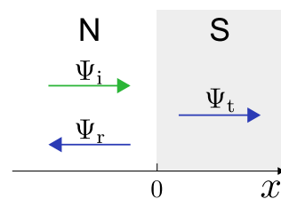
Figure 4.3. – Schematic of an SN interface. An incoming electron (green) can be back-reflected or transmitted.
