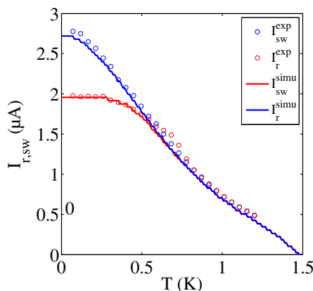
Figure 6.8. – Estimation of the volume of the junction. The circles display the measured switching and retrapping currents of junction LC106. The curves represent the simulated switching and retrapping currents with a volume \mathcal{V}_{\text{LC106}} = 2.4 \mu\text{m} \cdot 30 \text{ nm} \cdot (150 \text{ nm} + 400 \text{ nm}) = 4 \times 10^{-2} \mu\text{m}^3 .
