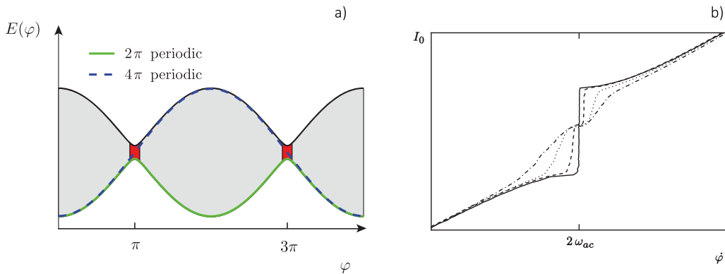
Figure C.2. – (a): Energy-phase relation of the 4\pi periodic ABS by taking into account LZ transitions. The grey and red regions corresponds to the adiabatic and non-adiabatic evolution of the system. In the adiabatic limit, the 4\pi periodic ABS is not subject to LZ transitions (dashed blue line), whereas in the non-adiabatic limit, the 4\pi periodic ABS loses its 4\pi periodicity. (b): Zoom on the second Shapiro step of the simulated current-voltage characteristic of a 1D topological Josephson junction hosting zero energy Majorana modes. The junction is current biased and irradiated with radio-frequencies. The curves are different simulations for an increasing gap E_g between the upper and lower energy states using the resistively shunted junction model with a E_J/E_g = 500 (solid), 100 (dashed), 50 (dotted), 30 (dotted-dashed). With E_J = \hbar I_c/2e being the Josephson energy. Extracted from [49].
