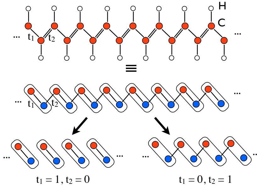
Figure 1.5. – Schematic representation of a molecule of polyacetylene extracted from [171]. Atoms of carbon are bond by either single or double bonds. The hopping term of electrons from one carbon to its left (right) neighbour is t_1 ( t_2 ). The two limit cases t_1 = 1 and t_1 = 0 are sketched in the lower schematic.
