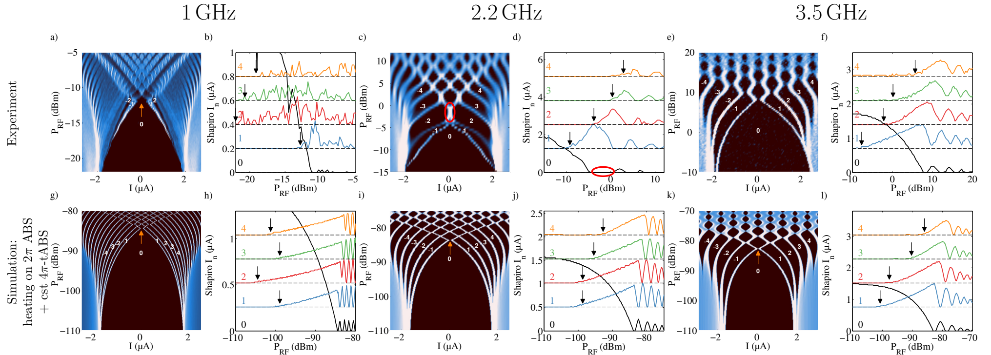
Figure 6.10. – Differential resistance of the junction LC106-JJ2 under RF irradiation at 1, 2.2 and 3.5 GHz and the associated amplitude of the Shapiro first steps I_n . The first Shapiro steps are labeled. The orange arrow and the red circle point at anomalies at the crossing point between the switching branch and the retrapping branch. It is further discussed in the main text. The arrows point at the RF power where the step appear.
