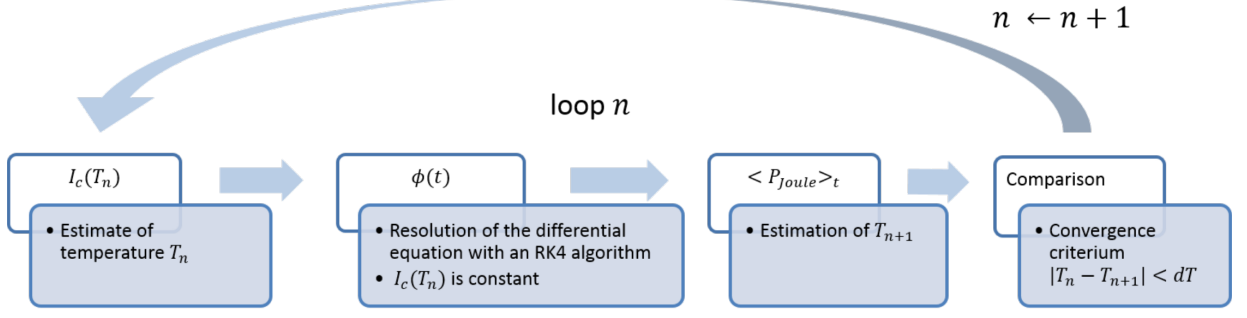
Figure 5.8. – Schematic of the algorithm used to self-consistently determine the temperature for each pair of parameter (I_{DC}, I_{RF}) . We start by supposing a temperature T_n (The first iteration is with the bath temperature T_0 = T_{\text{bath}} = 100 \text{ mK} ) which gives a critical current I_c(T_n) . We solve Eq. (5.14) during a long period of time (greater than 1/f_{RF} ). From \phi(t) we estimate the Joule heating which gives us a new estimation of the temperature ( T_{n+1} using Eq. (5.21)). If |T_{n+1} - T_n| is small enough, we exit the convergence loop and start again for the next pair of parameter (I_{DC}, I_{RF}) . If not, the calculation starts again with T_{n+1} .
