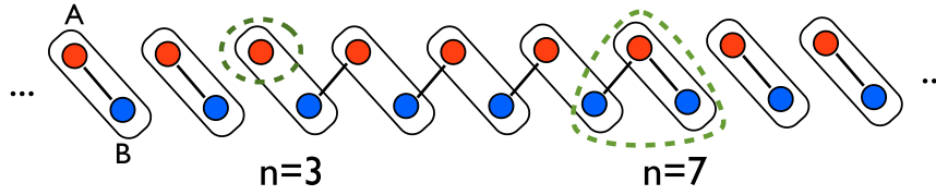
Figure 1.7. – Example of charge soliton in the SSH model. The system is composed of inter-cell hopping in-between n = 3 and n = 7 and outside of this region the system has intra-cell hopping. Extracted from [171].
