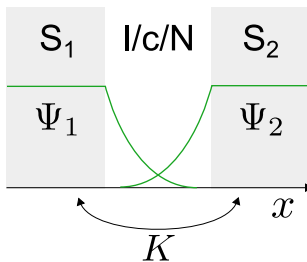
Figure 4.1 – Schematic of a Josephson junction. The order parameters of each lead decreases outside the superconducting region. The overlap between \Psi_1 and \Psi_2 defines the coupling constant K .
