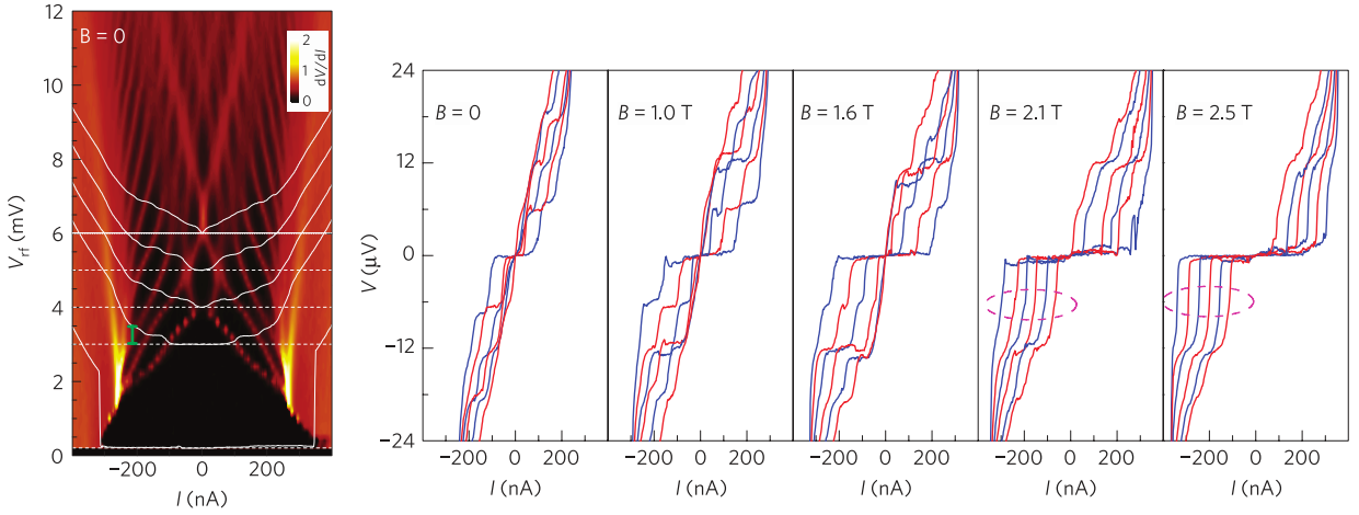
Figure 4.16. – Left panel: The colored plot shows the differential resistance (unit of k\Omega ) with respect to RF irradiation amplitude in mV at 3 GHz and DC current bias at zero magnetic field and dilution fridge temperature. The white dotted lines are linecuts of the |V(I)| characteristic at V_{\text{RF}} = 0.2, 3, 4, 5 and 6 mV drawn in white solid lines. The green line represents a scale of 12 \mu\text{V} on the |V(I)| curves. Right panel: V(I) characteristics of the junction for increasing magnetic field. For B lower than 2 T, all Shapiro steps are visible at voltages V_n = n \cdot hf_{\text{RF}}/2e = n \cdot 6 \mu\text{V} . For magnetic field greater than 2 T, the step n = 1 at 6 \mu\text{V} disappears as emphasized by the dotted circles. This disappearance of an odd Shapiro step is an evidence of a topological superconductivity. Adapted from [142].
