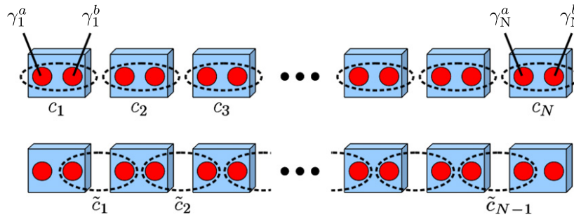
Figure 4.9. – Schematic of the Kitaev chain. Upper panel: the fermion operator c_j is composed of two Majorana fermion operator on the same site j . Lower panel: in the case of \mu = 0 and t = \Delta , two neighboring \gamma form a new fermion operator \tilde{c} which sits on two different site. This new point of view leaves two Majorana operators unpaired: \gamma_1^a and \gamma_N^b . Extracted from [113].
