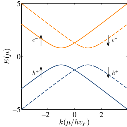
Figure 4.12 – Energy dispersion relation for the 4 energy states of (4.51) with the following parameters : \mu = 1 meV, v_F = 5 \times 10^5 m s ^{-1} and \Delta = 800 \mu eV. Solid lines corresponds to, say, up spin, and dashed line to the opposite spin.
