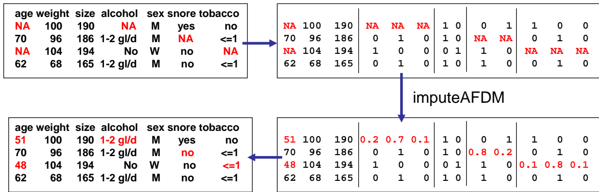
Figure 3.2: Illustration of the regularized iterative FAMD algorithm on the incomplete snore data. Top left: the incomplete data; top right: coding of the data; bottom right: the imputed data; bottom left: the original data set completed.
