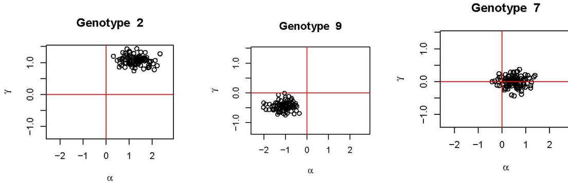
Figure 5.4: Genotype effect: for a subset of genotype i_{(i=2,7,9)} representation of (\alpha_i^s \sqrt{J}, q_{i,1}^s \sqrt{d_1}^s) , s = 1, \dots, 1000 , that is the main effect and interaction of each genotype.
