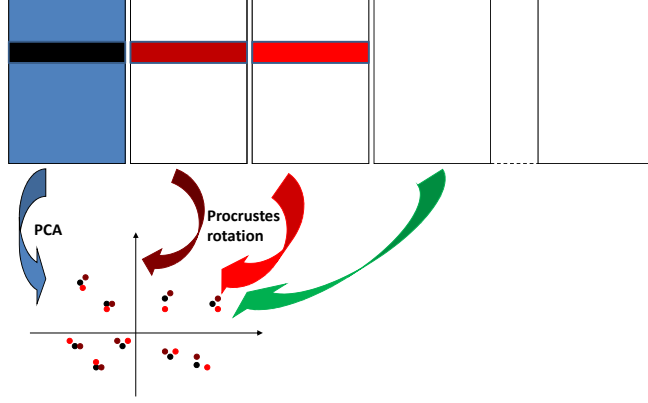
Figure 5.1: Procrustes rotations of the rows of the PCA estimators onto the initial configuration. The first table corresponds to X and the others to \hat{\mu}^{(S)^1}, \dots, \hat{\mu}^{(S)^*} obtained either by the asymptotic, the bootstrap or the jackknife strategies. PCA is applied on X to get the representation of the rows of \hat{\mu}^S (black dots), then the rows of each \mu^{(S)^*} are rotated and represented (red dots, brown dots, etc).
