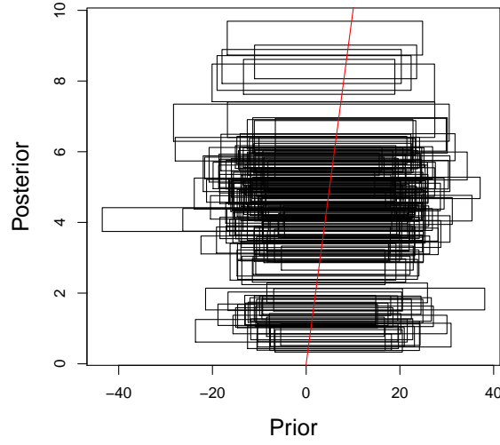
Figure 5.3: Prior-posterior credible boxes for the \mu_{ij} ( i = 1, \dots, 16 ; j = 1, \dots, 10 ). The red line corresponds to the equality between the abscissa and the ordinate.
