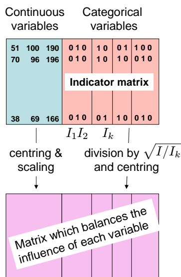
Figure 3.1: Coding the data in factorial analysis for mixed data.
