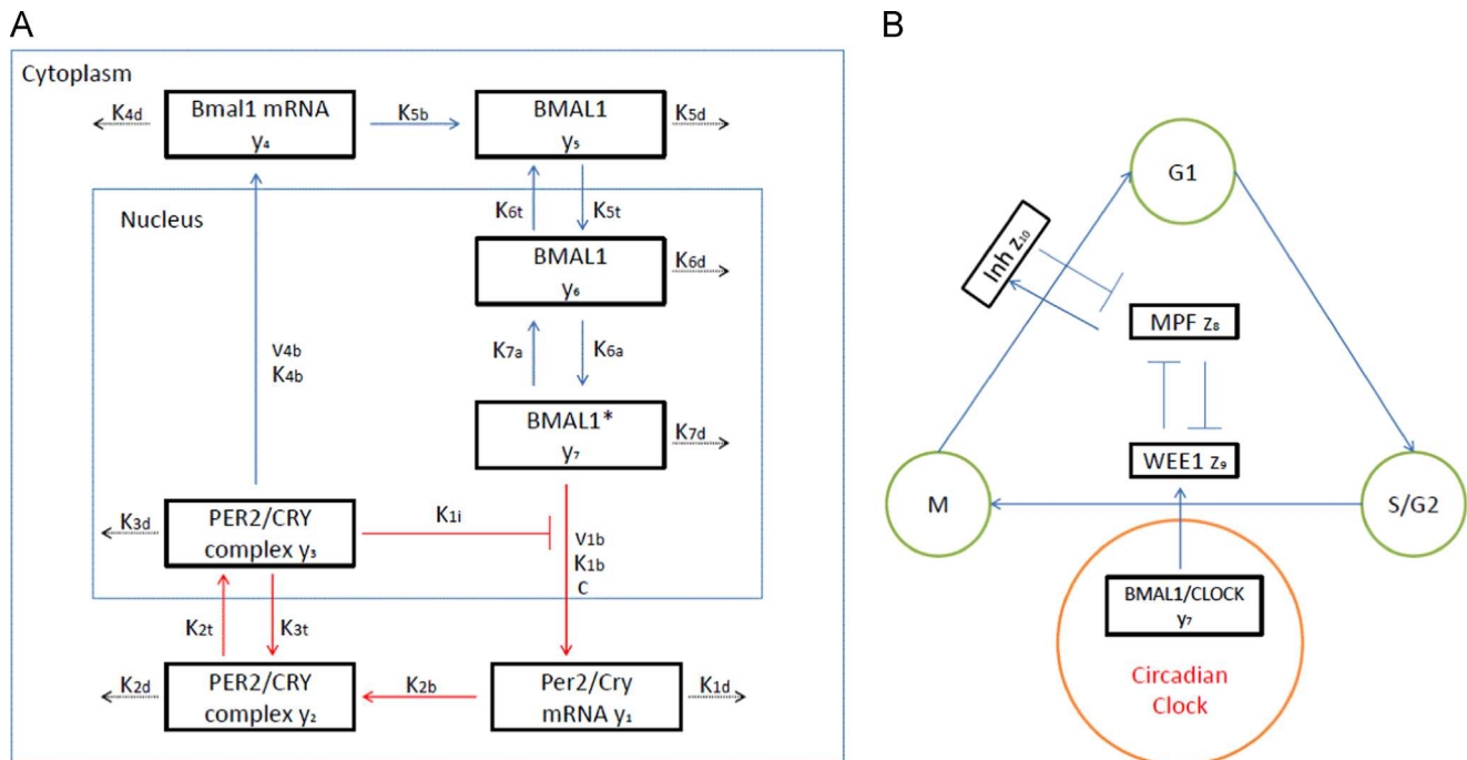
Fig. 1. (A) Scheme of the circadian clock network: the activated heterodimer BMAL1/CLOCK (BMAL1*, y_7 ) activates Per 2 and Cry genes, which produce Per2/Cry mRNA ( y_1 ). PER2 and CRY proteins are synthesized and bind in the cytosol to form a complex ( y_2 ) to be transported into the nucleus ( y_3 ). This complex inhibits the activity of BMAL1/CLOCK complex, thus destroying its own source of transcription and closing the negative feedback loop. The nuclear complex PER2/CRY ( y_3 ) also activates Bmal 1 transcription, which produces an increase in Bmal 1 mRNA ( y_4 ), and cytosolic protein concentration ( y_5 ). The BMAL1/CLOCK complex is then transported to the nucleus ( y_6 ), where it is activated. The activated BMAL1/CLOCK complex (BMAL1*, y_7 ) restarts the activation process of Per2/Cry . (B) Schematic representation of the coupling between the cell cycle and the circadian clock through the protein WEE1 ( z_9 ) (Matsuo et al., 2003). In the model, the cell cycle is divided into three successive phases G1, S/G2, M. Transitions from one phase to another depend on the activity of MPF ( z_8 ). For cells to leave G1 and enter S/G2, MPF activity must exceed a fixed threshold \theta_1 = 0.09 . For cells to leave S/G2 and enter M phase, MPF activity must exceed that of WEE1 ( z_9 ). In the M phase, MPF activates its inhibitor ( z_{10} ), which represses MPF activity, letting it shut down and forcing the cell to exit mitosis. Division occurs once MPF activity reaches a low threshold level \theta_2 = 0.06 . Coupling between the cell cycle and the circadian clock is achieved by the transcriptional activation of Wee1 , which induces WEE1 activity ( z_9 ) by the active BMAL1/CLOCK complex ( y_7 ).
