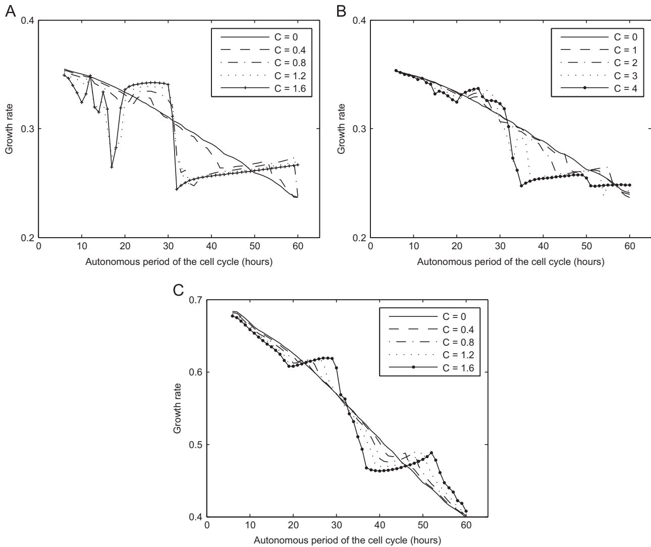
Fig. 5. Effects of coupling on the growth rate. (A) Present model. (B and C) Effects of coupling on the growth rate with other models chosen from the literature for the circadian clock: Mirsky et al. (2009) (B), and Leloup and Goldbeter (2004) (C).
