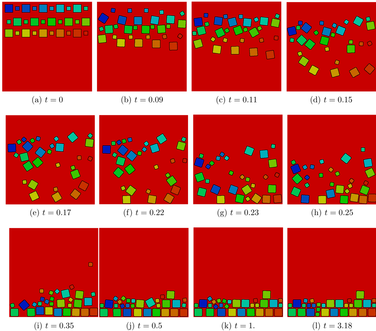
Figure 5.25: Simulation of 30 square rigid bodies of different size falling under gravity. The intensity of the force is constant k = 100 .
