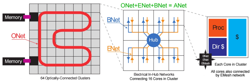
FIGURE 2.9: ATAC's 2 level clustered architecture, where clusters are connected by bundle of optical waveguides using WDMA. For reception, each cluster incorporates a special electrical broadcast network. (Image taken from [3])
