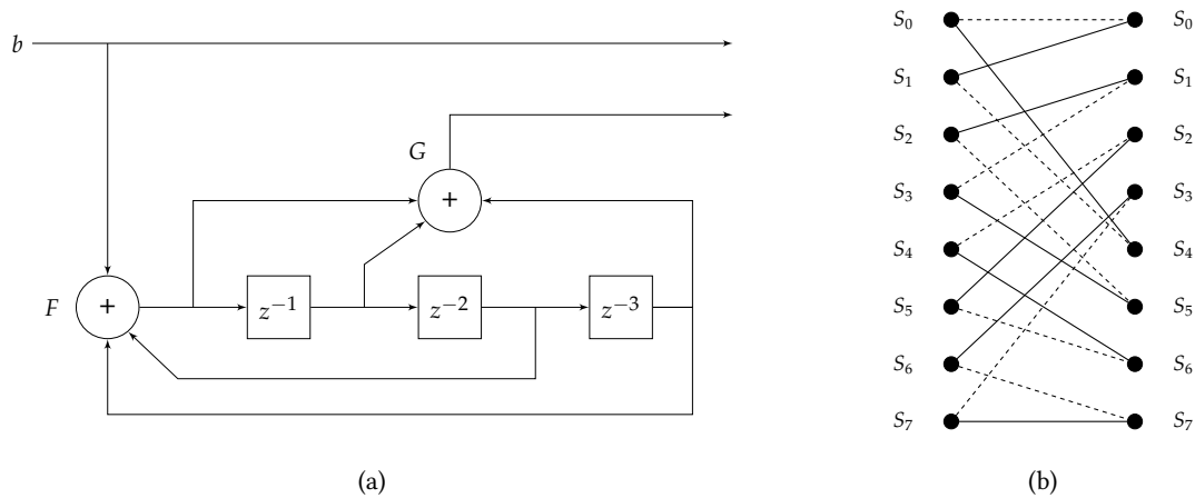
FIGURE 1.11 – Encoder (a) and trellis (b) of the [13\ 15] convolutional code in its recursive form
