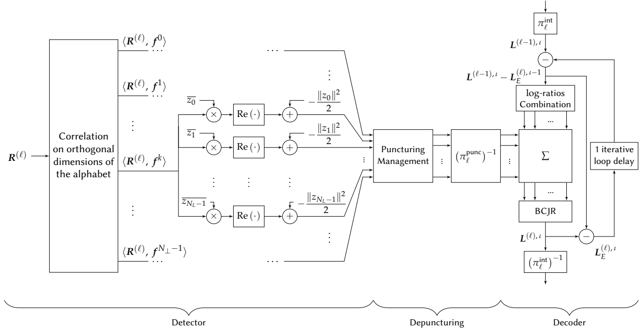
FIGURE 3.9 – The Coplanar Turbo-FSK one stage receiver's architecture.
