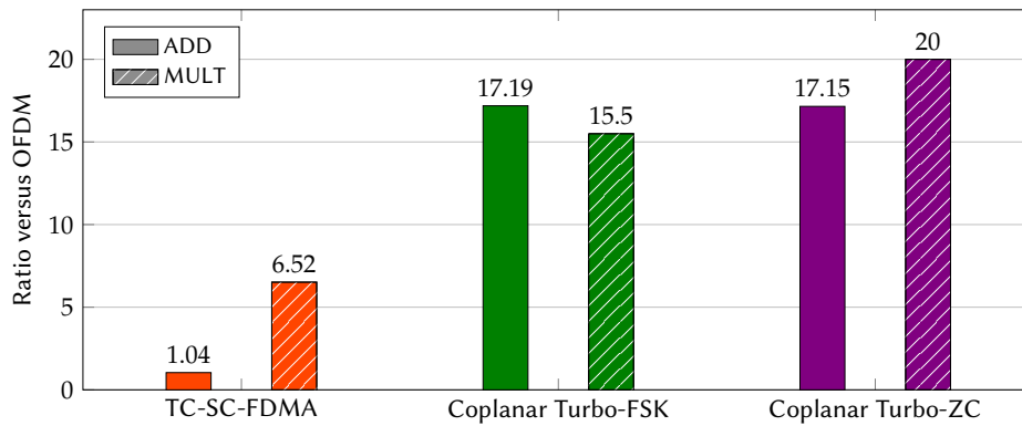
FIGURE 4.20 – Complexity ratios with respect to the TC-OFDM, for the high throughput scenario.
