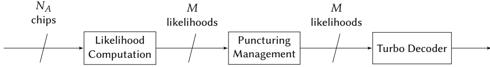
FIGURE 4.9 – Demodulator/Decoder for the Coplanar Turbo-FSK and Turbo-ZC schemes.
