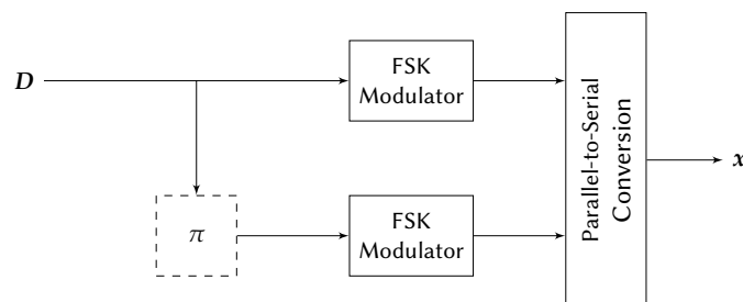
FIGURE 2.1 – Parallel concatenation of two FSK modulations.
