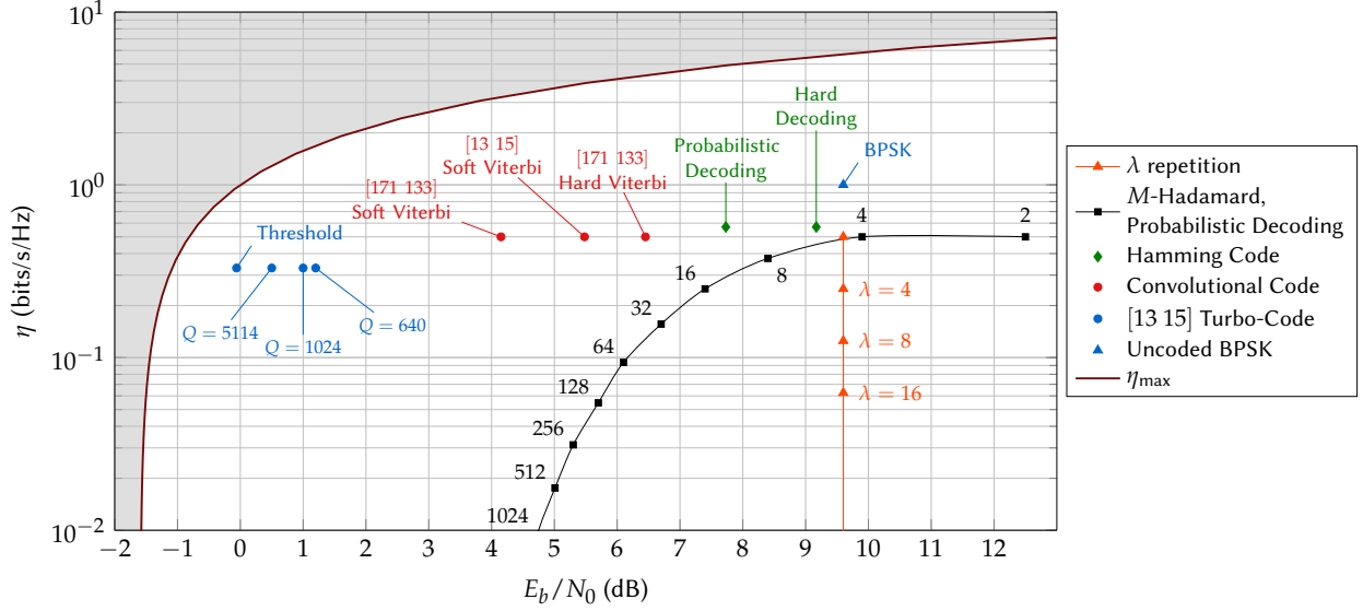
FIGURE 1.14 – Comparison of the spectral efficiency and the required E_b/N_0 at \text{BER} = 10^{-5} of various FEC schemes, under the AWGN channel. The maximum achievable spectral efficiency according to the channel capacity from (1.15) is also represented.
