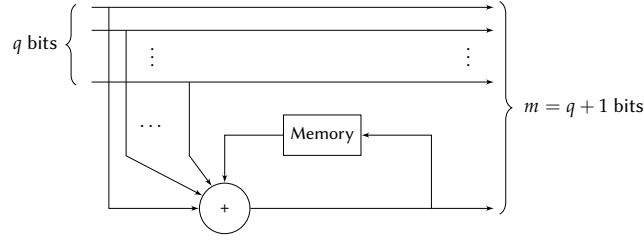
FIGURE 2.7 – The Parity-Accumulator encoder
