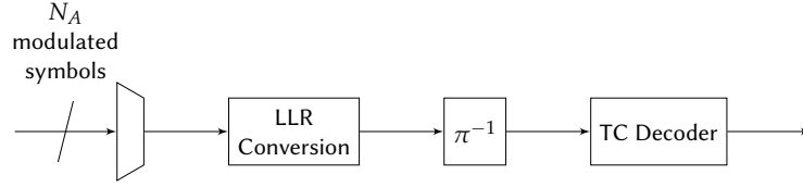
FIGURE 4.3 – Demodulator/Decoder for the TC-OFDM scheme.
