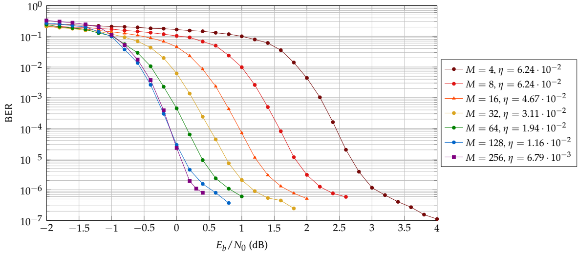
FIGURE 2.18 – Performance of the Turbo-FSK scheme with parameters \lambda = 4 , Q = 1024 , for various size of FSK alphabet M and under the AWGN channel. 10 iterations are performed, and the MAP algorithm is used.
