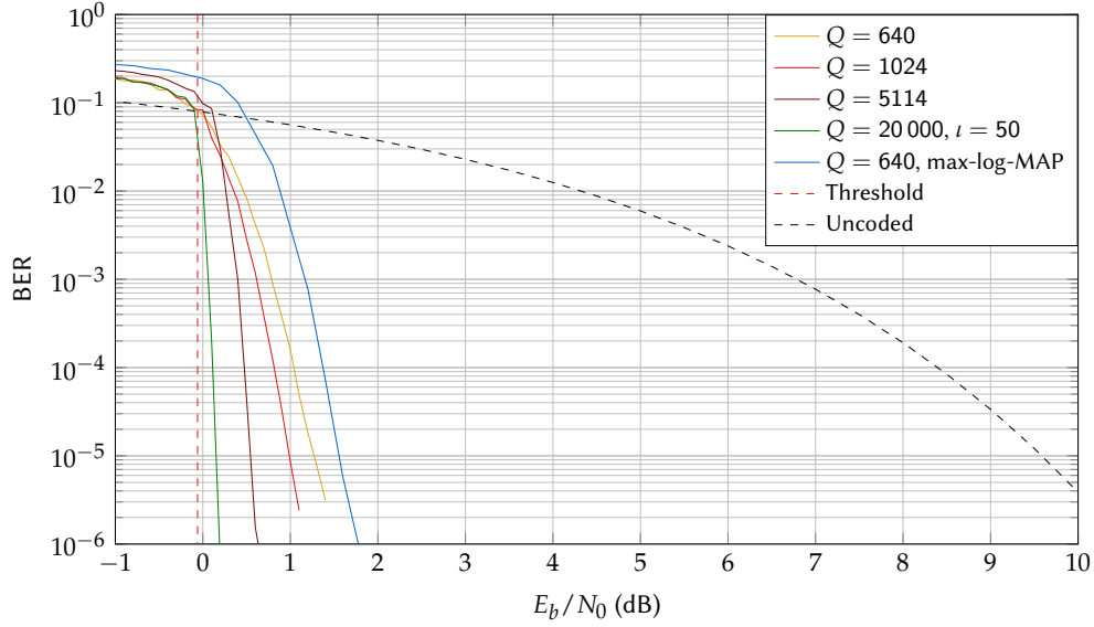
FIGURE 1.13 – Performance of the [13 15] TC for various interleaver sizes Q , under the AWGN channel. A total of \iota = 10 iterations are performed unless stated otherwise.
