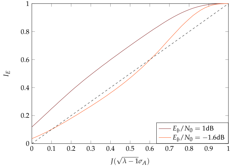
FIGURE 2.21 – EXIT Charts of the Turbo-FSK decoder with parameters M = 128 , \lambda = 4 , for various values of E_b/N_0 . The information block size was set to Q = 100\,000 .
