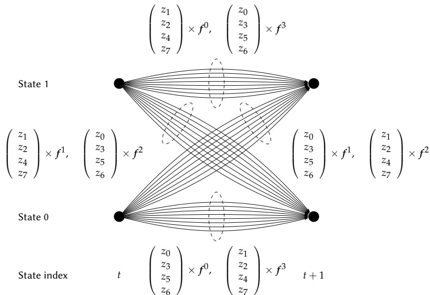
FIGURE 3.12 – A section of the trellis with X mapping for the configuration N_{\perp} = 4 and N_L = 8 .
