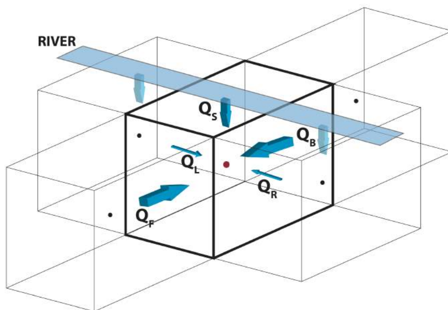
Figure 6.2 : Budget of a cell where a river condition is applied (particle endpoint)
