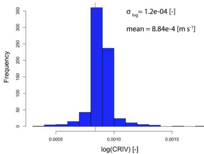
Figure 5.6 : Distribution probabiliste de CRIV
