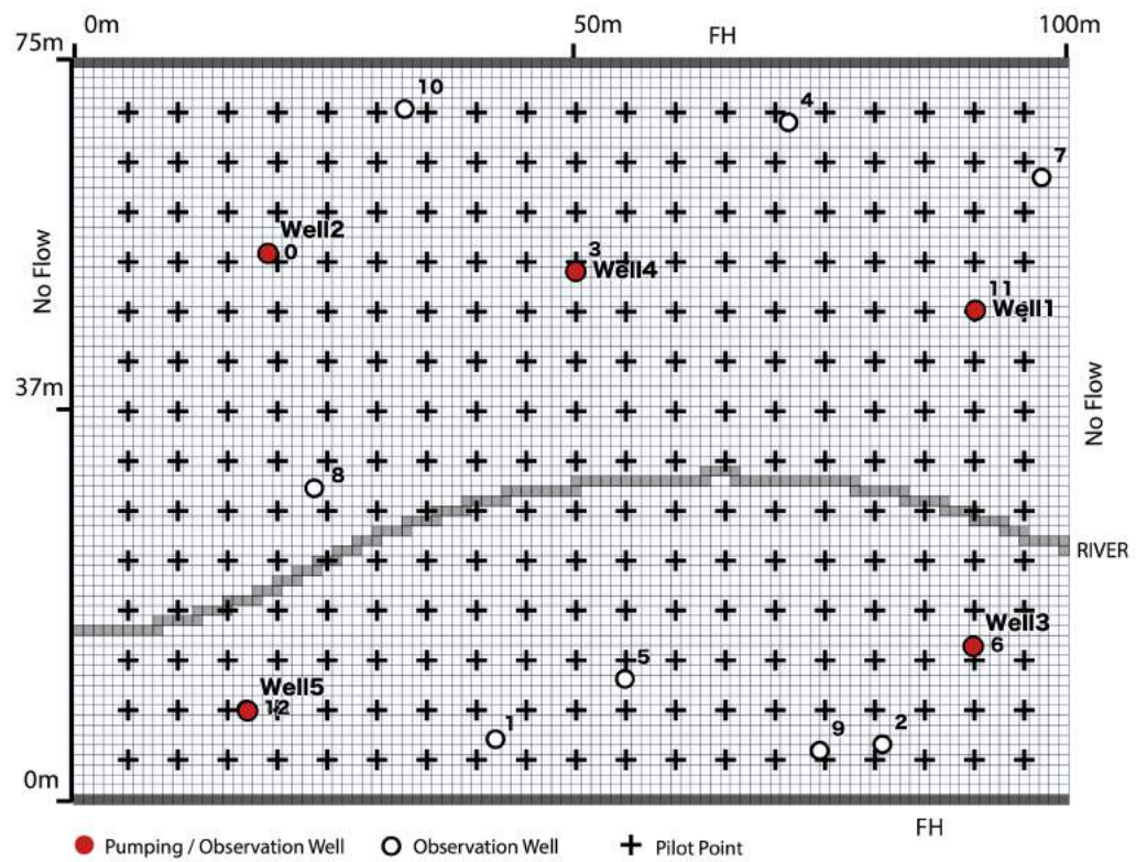
Figure 6.5 : Schematic diagram of the synthetic case
