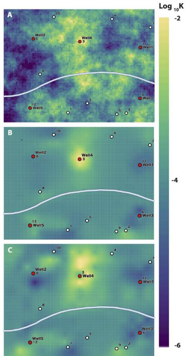
Figure 6.6 : Log of hydraulic conductivity field, observation wells (white) and pumping wells (red) A) "Real" hydraulic conductivity field obtained by unconditional Gaussian simulation, B) Calibrated hydraulic conductivity field against head observation only C) Calibrated hydraulic conductivity field against head and \alpha observations with the proposed surrogate model
