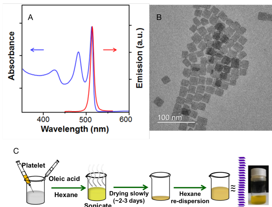
Figure 5.1: A) UV-VIS absorbance and emission spectra and B) TEM images of NPLs solutions used for the self-assembly. C) Scheme of the procedure for preparing self-assembled threads of CdSe platelets.
