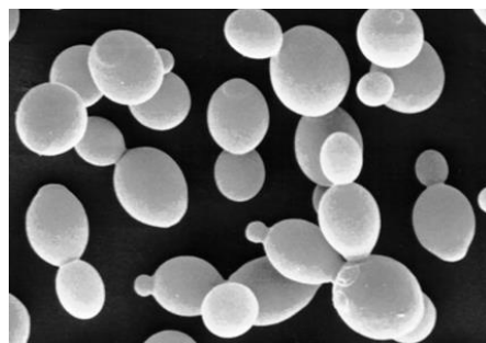
Figure 13 : Saccharomyces cerevisiae
