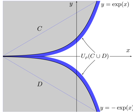
Figure 2.4: The union of two convex sets is not positively \alpha -far.
