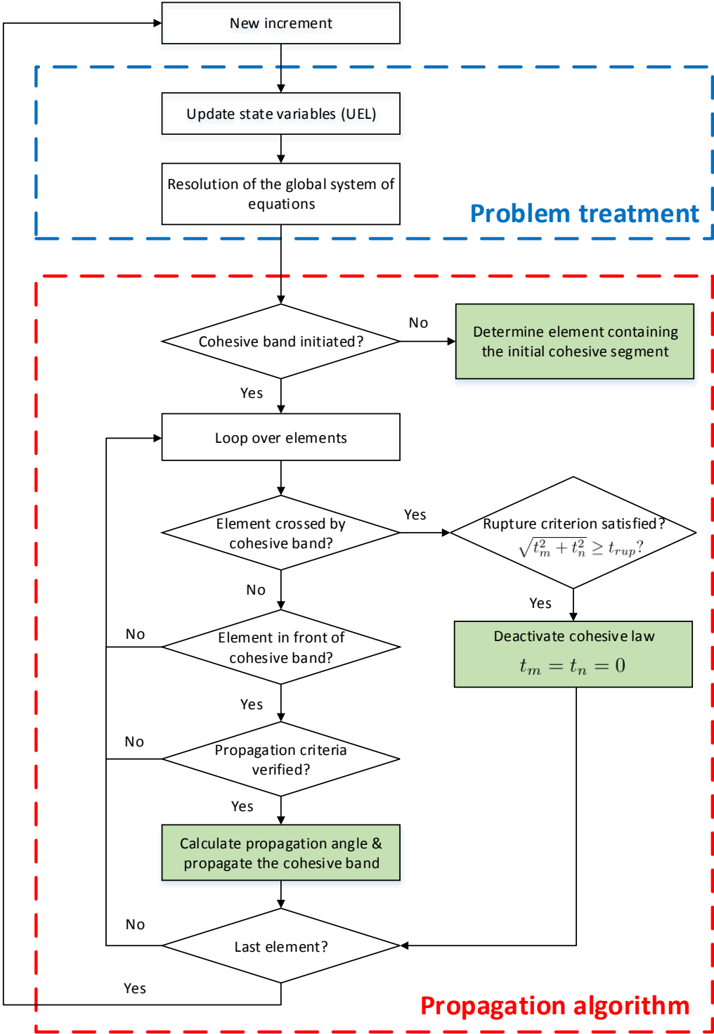
Figure IV.15 – Flow chart of propagation algorithm
