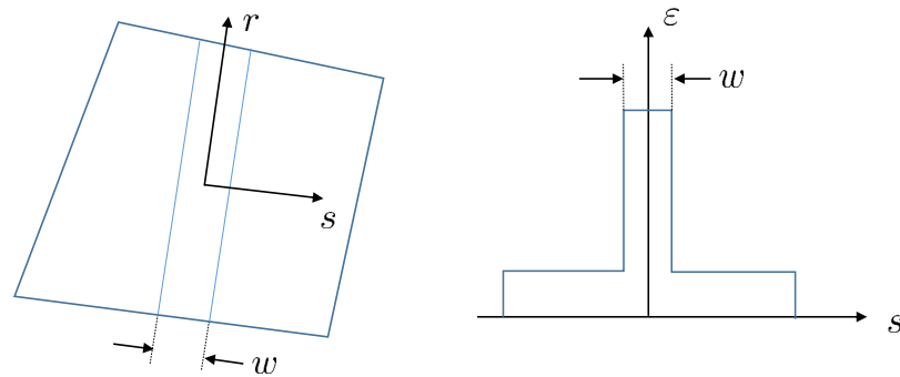
Figure II.5 – Embedded localization band inside a finite element (left) and strain field (right) (adapted from Belytschko [20])
