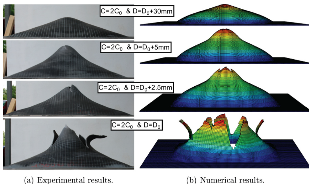
Figure I.3 – Comparison between experimental (a) and numerical (b) results of air-blast experiments using four different distances between the specimen and the explosive charge [58]
