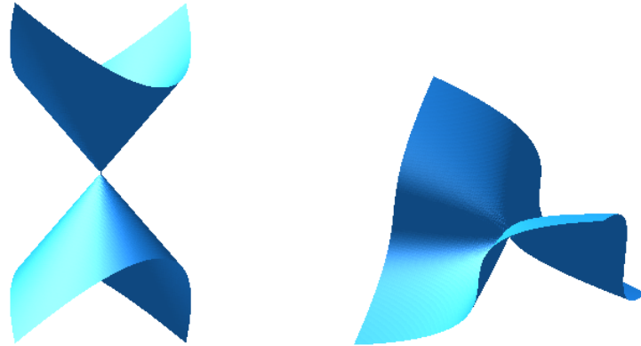
Representations of \mathbb{R}^3 \cap (\mathbb{C}^2/\mathcal{C}_n) for n = 2 and 3 .
