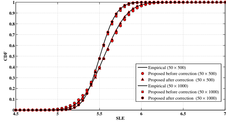
Figure 4.3: Empirical CDF of the SLE under \mathcal{H}_1 hypothesis and its corresponding proposed approximation for K = 50 with N = \{500, 1000\} and \rho = -10dB .
