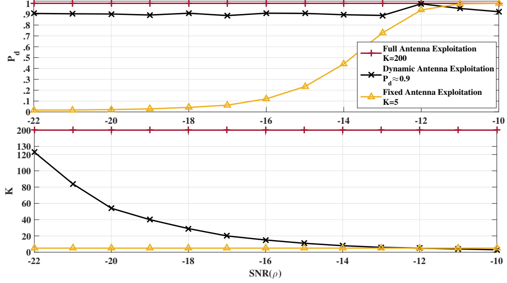
Figure 5.9: Empirical P_d of the SLE detector and the corresponding number of antennas, K , used for sensing in Full, Dynamic and Fixed methods w.r.t \rho and fixing N = 500 .
