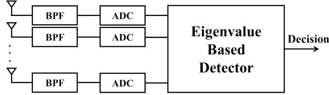
Figure 2.9: Eigenvalue based detector using multiple antennas.
