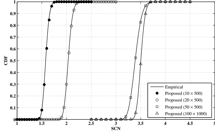
Figure 3.11: Empirical CDF of the SCN and its corresponding proposed GEV approximation for different values of K and N under \mathcal{H}_0 hypothesis.
